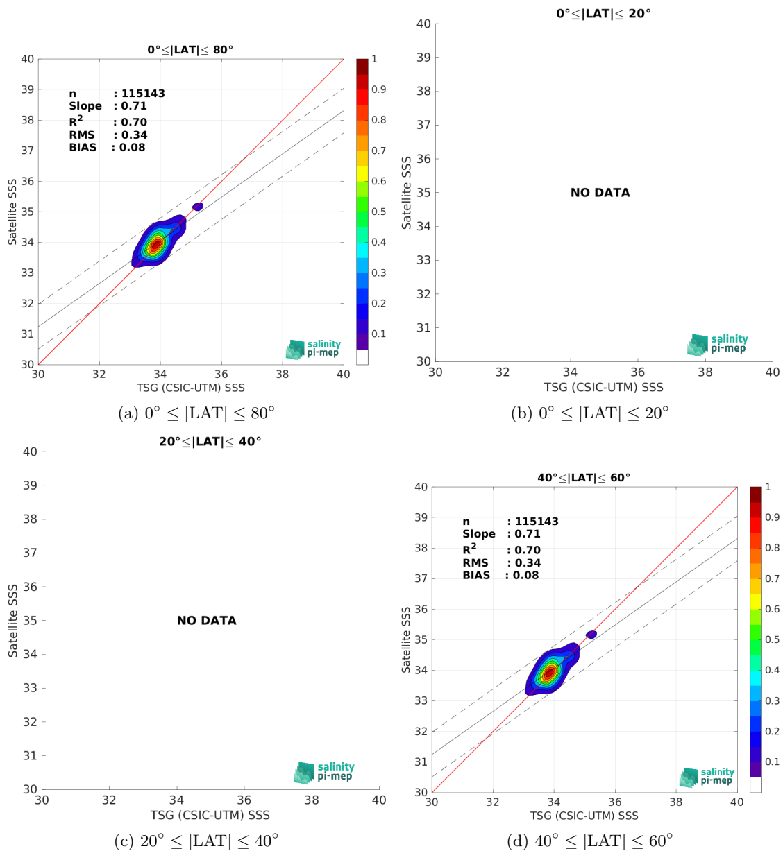
Figure 10: Contour maps of the concentration of CCI SSS L4 Merged-OI v4.41 - 7-day running (ESA) SSS (y-axis) versus TSG (CSIC-UTM) SSS (x-axis) at match-up pairs for different latitude bands. For each plot, the red line shows x=y . The black thin and dashed lines indicate a linear fit through the data cloud and the \pm 95\% confidence levels, respectively. The number match-up pairs n , the slope and R^2 coefficient of the linear fit, the root mean square (RMS) and the mean bias between satellite and in situ data are indicated for each latitude band in each plots.
