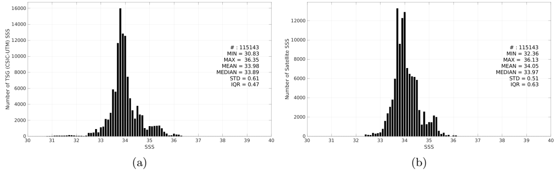
Figure 3: Histograms of SSS from TSG (CSIC-UTM) (a) and CCI SSS L4 Merged-OI v4.41 - 7-day running (ESA) (b) considering all match-up pairs per bins of 0.1 over the Roaring Forties and Furious Fifties Pi-MEP region and for the full satellite product period.
