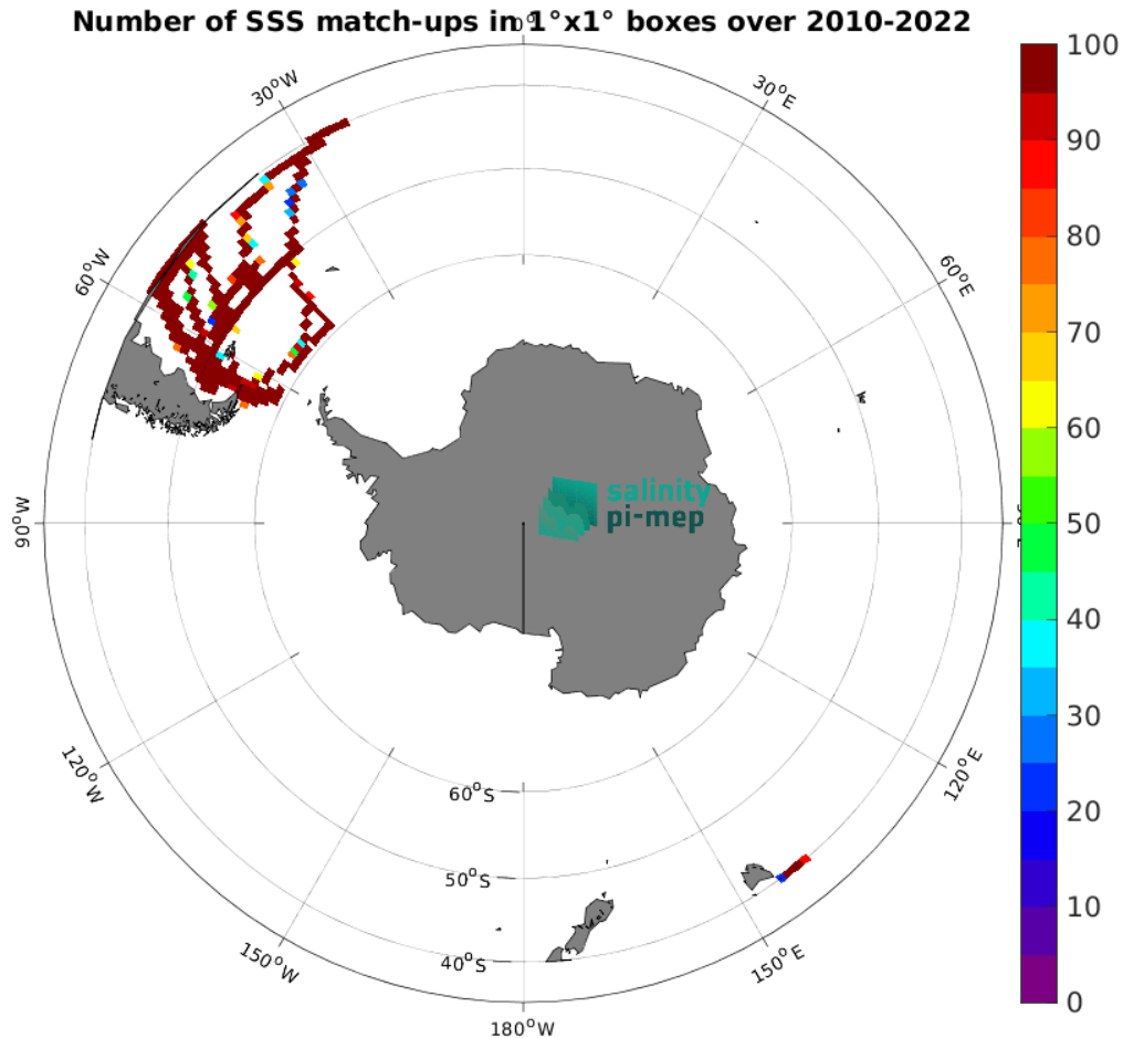
Figure 5: Number of SSS match-ups between TSG (CSIC-UTM) SSS and the CCI SSS L4 Merged-OI v4.41 - 7-day running (ESA) SSS product for the Roaring Forties and Furious Fifties Pi-MEP region over 1^\circ \times 1^\circ boxes and for the full satellite product period.
