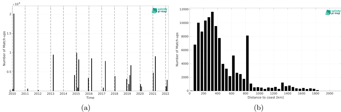
Figure 2: Number of match-ups between TSG (CSIC-UTM) and CCI SSS L4 Merged-OI v4.41 - 7-day running (ESA) SSS as a function of time (a) and as function of the distance to coast (b) over the Roaring Forties and Furious Fifties Pi-MEP region and for the full satellite product period.
