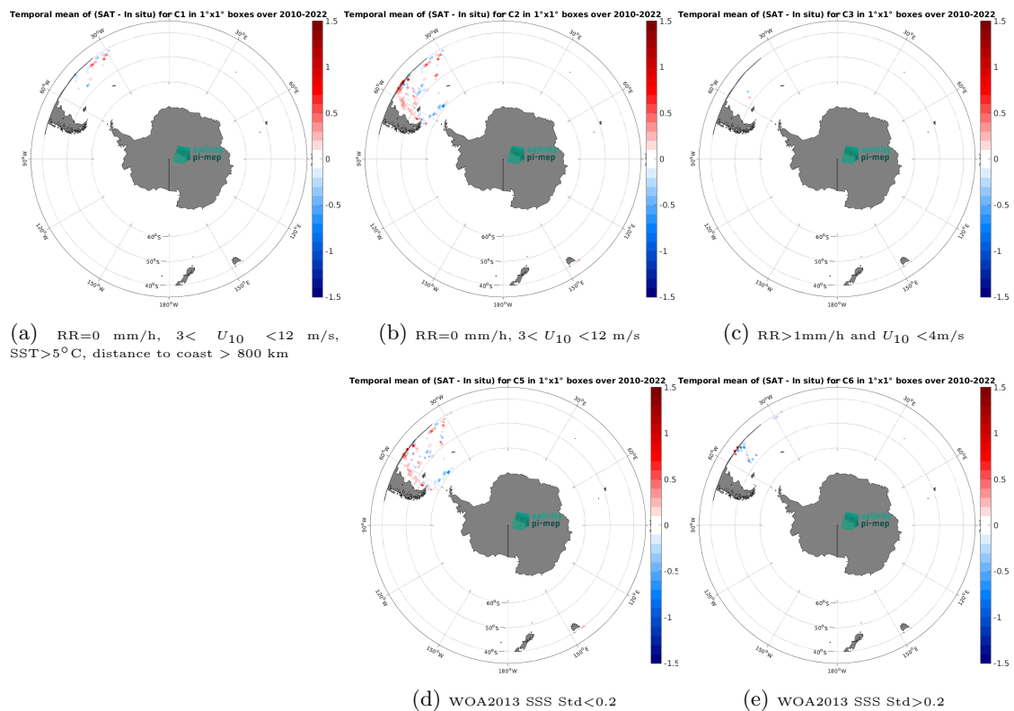
Figure 14: Temporal mean gridded over spatial boxes of size 1^\circ \times 1^\circ of \Delta\text{SSS} (CCI SSS L4 Merged-OI v4.41 - 7-day running (ESA) - TSG (CSIC-UTM)) for 5 different subdatasets corresponding to:RR=0 mm/h, 3 < U_{10} < 12 m/s, SST>5°C, distance to coast > 800 km (a), RR=0 mm/h, 3 < U_{10} < 12 m/s (b), RR>1mm/h and U_{10} < 4 m/s (c), WOA2013 SSS Std<0.2 (d), WOA2013 SSS Std>0.2 (e).
