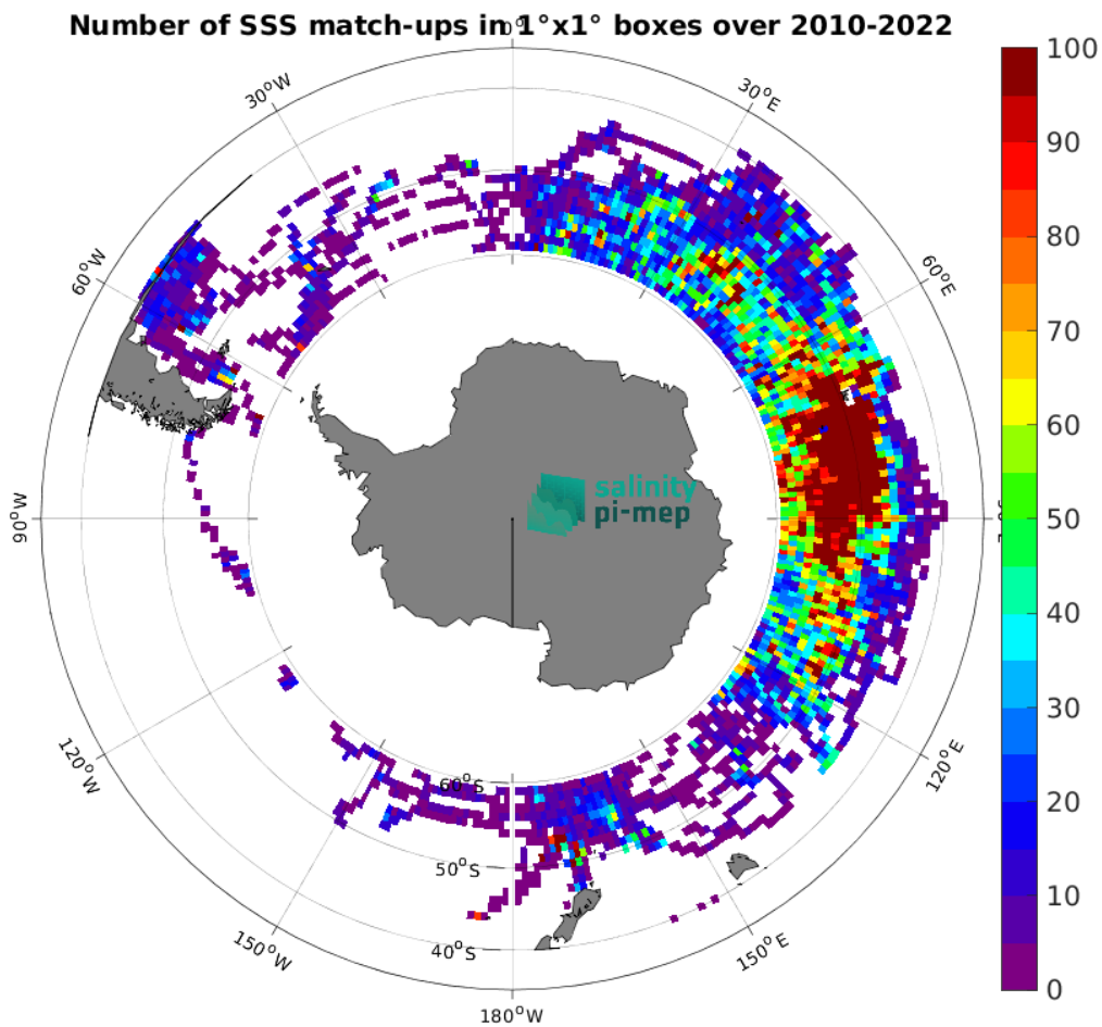
Figure 5: Number of SSS match-ups between Marine mammals SSS and the CCI SSS L4 Merged-OI v4.41 - 7-day running (ESA) SSS product for the Roaring Forties and Furious Fifties Pi-MEP region over 1^{\circ} \times 1^{\circ} boxes and for the full satellite product period.
