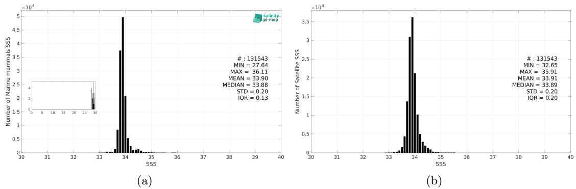
Figure 3: Histograms of SSS from Marine mammals (a) and CCI SSS L4 Merged-OI v4.41 - 7-day running (ESA) (b) considering all match-up pairs per bins of 0.1 over the Roaring Forties and Furious Fifties Pi-MEP region and for the full satellite product period.
