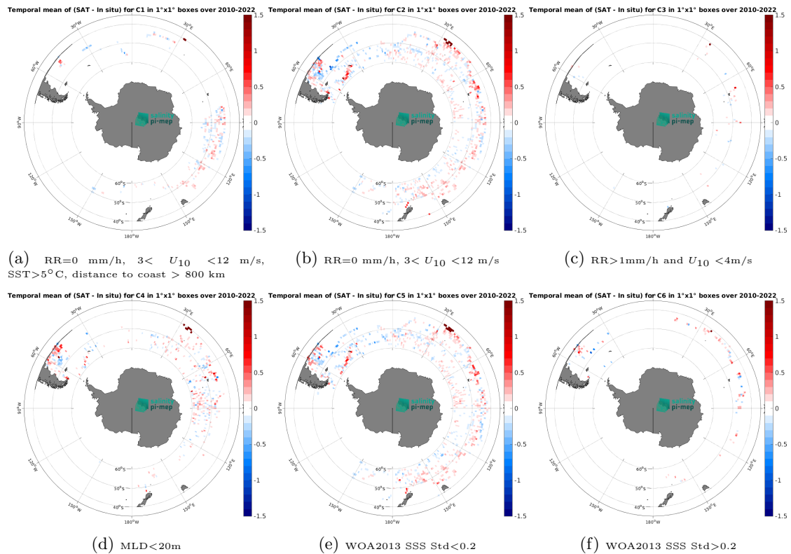
Figure 14: Temporal mean gridded over spatial boxes of size 1^\circ \times 1^\circ of \Delta SSS (CCI SSS L4 Merged-OI v4.41 - 7-day running (ESA) - Marine mammals) for 6 different subdatasets corresponding to:RR=0 mm/h, 3 < U_{10} < 12 m/s, SST >5^\circ C, distance to coast > 800 km (a), RR=0 mm/h, 3 < U_{10} < 12 m/s (b), RR >1 mm/h and U_{10} < 4 m/s (c),MLD <20 m (d),WOA2013 SSS Std <0.2 (e),WOA2013 SSS Std >0.2 (f).
