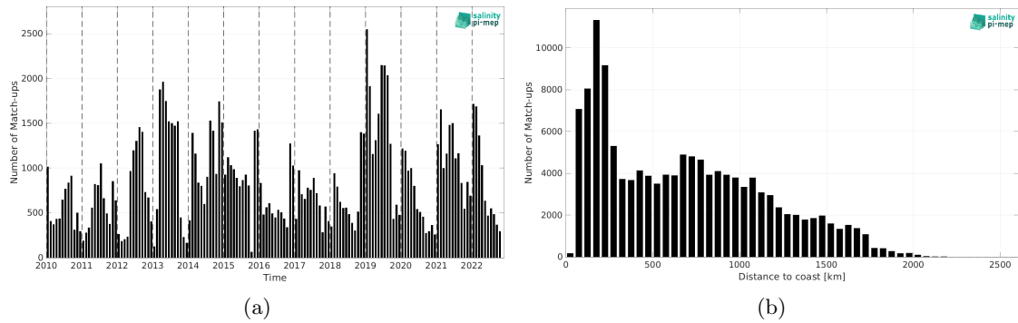
Figure 2: Number of match-ups between Marine mammals and CCI SSS L4 Merged-OI v4.41 - 7-day running (ESA) SSS as a function of time (a) and as function of the distance to coast (b) over the Roaring Forties and Furious Fifties Pi-MEP region and for the full satellite product period.
