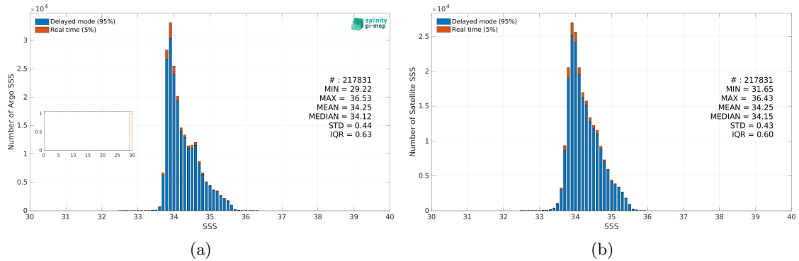
Figure 3: Histograms of SSS from Argo (a) and CCI SSS L4 Merged-OI v4.41 - 7-day running (ESA) (b) considering all match-up pairs per bins of 0.1 over the Roaring Forties and Furious Fifties Pi-MEP region and for the full satellite product period.
