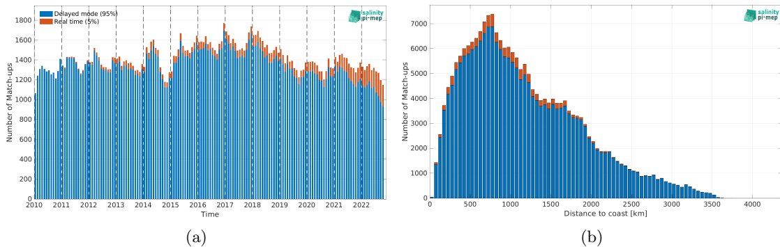
Figure 2: Number of match-ups between Argo and CCI SSS L4 Merged-OI v4.41 - 7-day running (ESA) SSS as a function of time (a) and as function of the distance to coast (b) over the Roaring Forties and Furious Fifties Pi-MEP region and for the full satellite product period.
