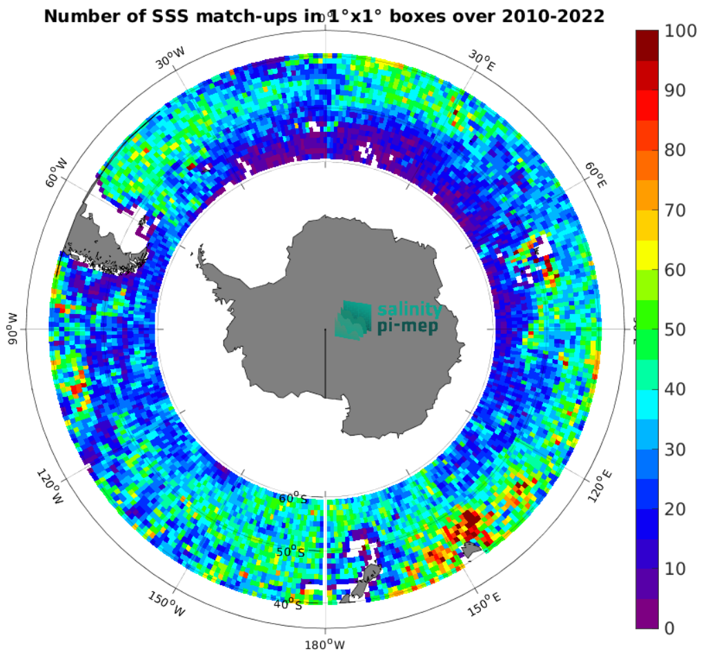
Figure 5: Number of SSS match-ups between Argo SSS and the CCI SSS L4 Merged-OI v4.41 - 7-day running (ESA) SSS product for the Roaring Forties and Furious Fifties Pi-MEP region over 1^\circ \times 1^\circ boxes and for the full satellite product period.
