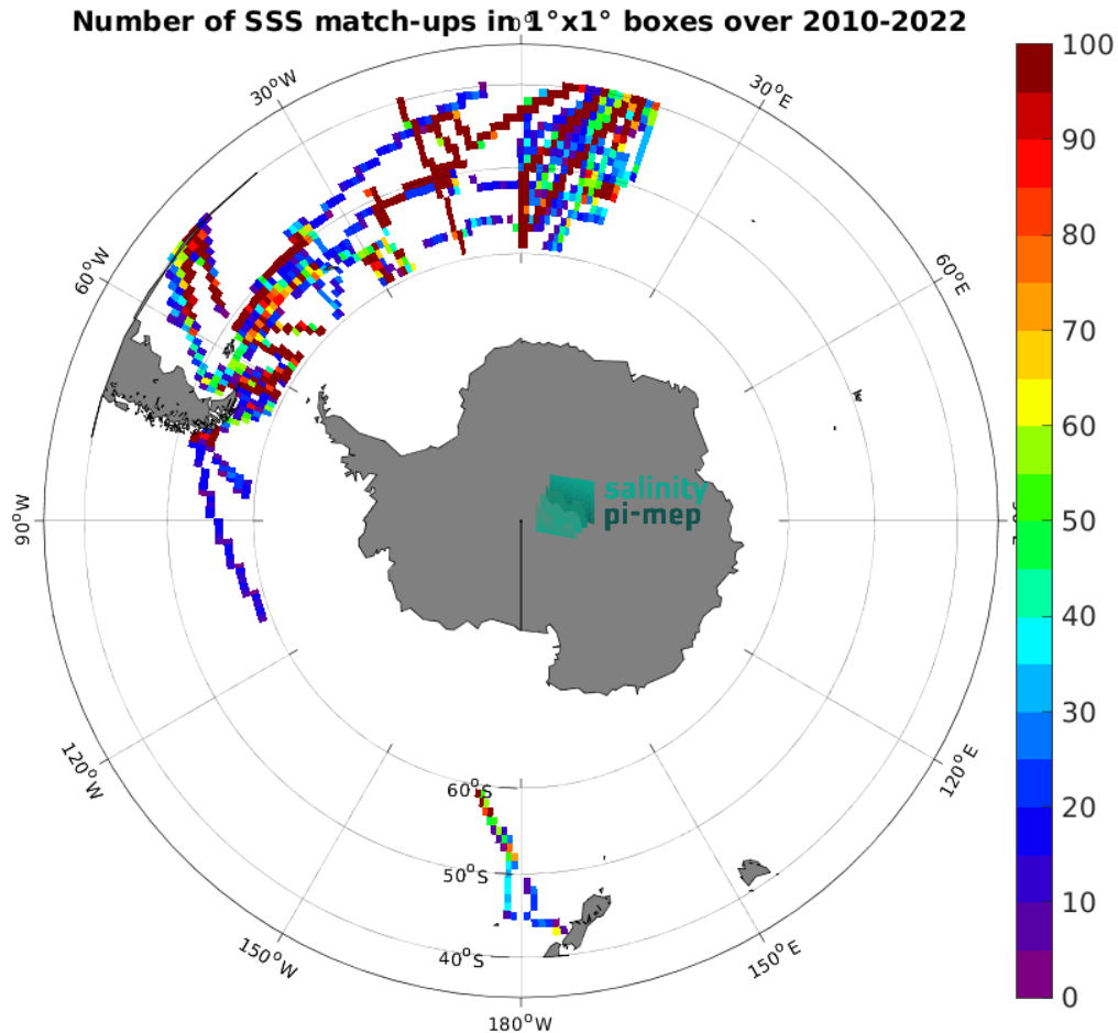
Figure 5: Number of SSS match-ups between TSG (Polarstern) SSS and the CCI SSS L4 Merged-OI v4.41 - 30-day running (ESA) SSS product for the Roaring Forties and Furious Fifties Pi-MEP region over 1^\circ \times 1^\circ boxes and for the full satellite product period.
