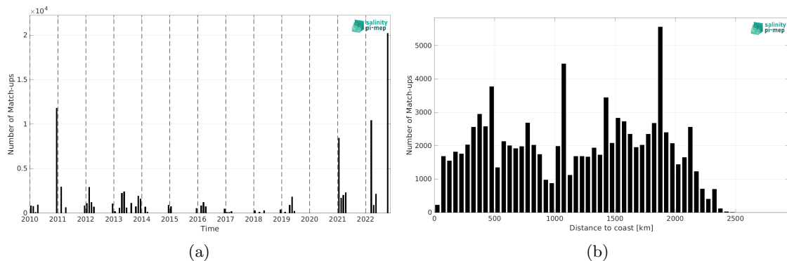
Figure 2: Number of match-ups between TSG (Polarstern) and CCI SSS L4 Merged-OI v4.41 - 30-day running (ESA) SSS as a function of time (a) and as function of the distance to coast (b) over the Roaring Forties and Furious Fifties Pi-MEP region and for the full satellite product period.
