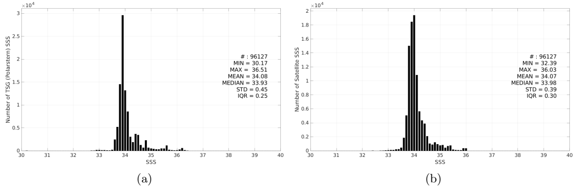
Figure 3: Histograms of SSS from TSG (Polarstern) (a) and CCI SSS L4 Merged-OI v4.41 - 30-day running (ESA) (b) considering all match-up pairs per bins of 0.1 over the Roaring Forties and Furious Fifties Pi-MEP region and for the full satellite product period.
