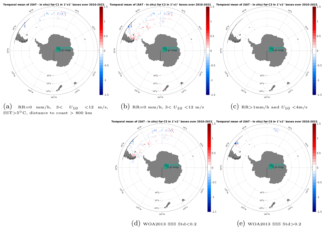
Figure 14: Temporal mean gridded over spatial boxes of size 1^\circ \times 1^\circ of \Delta SSS (CCI SSS L4 Merged-OI v4.41 - 30-day running (ESA) - TSG (Polarstern)) for 5 different subdatasets corresponding to:RR=0 mm/h, 3 < U_{10} < 12 m/s, SST >5^\circ C, distance to coast > 800 km (a), RR=0 mm/h, 3 < U_{10} < 12 m/s (b), RR >1 mm/h and U_{10} < 4 m/s (c), WOA2013 SSS Std <0.2 (d), WOA2013 SSS Std >0.2 (e).
