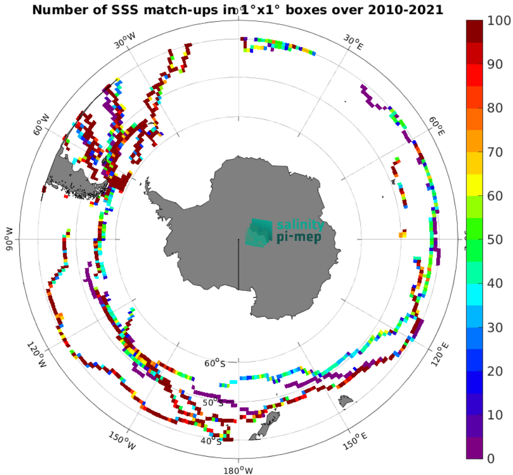
Figure 5: Number of SSS match-ups between TSG (GOSUD-Sailing-ship) SSS and the CCI SSS L4 Merged-OI v4.41 - 30-day running (ESA) SSS product for the Roaring Forties and Furious Fifties Pi-MEP region over 1^\circ \times 1^\circ boxes and for the full satellite product period.
