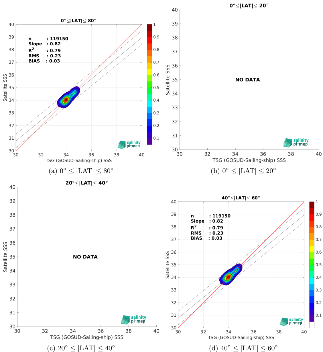
Figure 10: Contour maps of the concentration of CCI SSS L4 Merged-OI v4.41 - 30-day running (ESA) SSS (y-axis) versus TSG (GOSUD-Sailing-ship) SSS (x-axis) at match-up pairs for different latitude bands. For each plot, the red line shows x=y . The black thin and dashed lines indicate a linear fit through the data cloud and the \pm 95\% confidence levels, respectively. The number match-up pairs n , the slope and R^2 coefficient of the linear fit, the root mean square (RMS) and the mean bias between satellite and in situ data are indicated for each latitude band in each plots.
