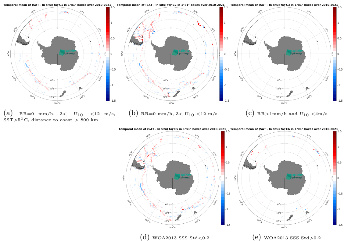
Figure 14: Temporal mean gridded over spatial boxes of size 1^\circ \times 1^\circ of \Delta SSS (CCI SSS L4 Merged-OI v4.41 - 30-day running (ESA) - TSG (GOSUD-Sailing-ship)) for 5 different subdatasets corresponding to:RR=0 mm/h, 3 < U_{10} < 12 m/s, SST >5^\circ C, distance to coast > 800 km (a), RR=0 mm/h, 3 < U_{10} < 12 m/s (b), RR >1 mm/h and U_{10} < 4 m/s (c), WOA2013 SSS Std <0.2 (d), WOA2013 SSS Std >0.2 (e).
