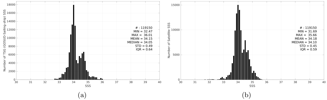
Figure 3: Histograms of SSS from TSG (GOSUD-Sailing-ship) (a) and CCI SSS L4 Merged-OI v4.41 - 30-day running (ESA) (b) considering all match-up pairs per bins of 0.1 over the Roaring Forties and Furious Fifties Pi-MEP region and for the full satellite product period.
