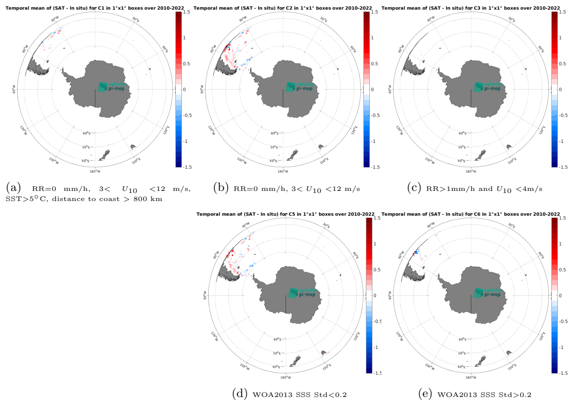
Figure 14: Temporal mean gridded over spatial boxes of size 1^\circ \times 1^\circ of \Delta\text{SSS} (CCI SSS L4 Merged-OI v4.41 - 30-day running (ESA) - TSG (CSIC-UTM)) for 5 different subdatasets corresponding to:RR=0 mm/h, 3 < U_{10} < 12 m/s, SST>5°C, distance to coast > 800 km (a), RR=0 mm/h, 3 < U_{10} < 12 m/s (b), RR>1mm/h and U_{10} < 4 m/s (c), WOA2013 SSS Std<0.2 (d), WOA2013 SSS Std>0.2 (e).
