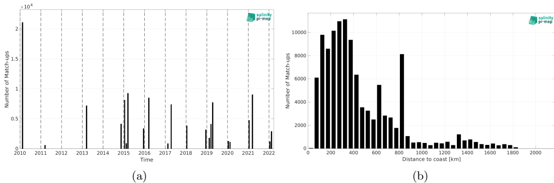
Figure 2: Number of match-ups between TSG (CSIC-UTM) and CCI SSS L4 Merged-OI v4.41 - 30-day running (ESA) SSS as a function of time (a) and as function of the distance to coast (b) over the Roaring Forties and Furious Fifties Pi-MEP region and for the full satellite product period.
