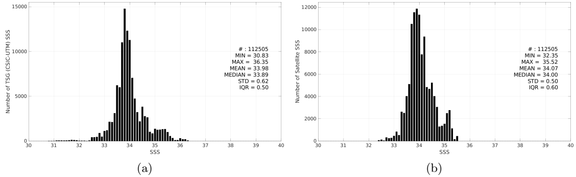
Figure 3: Histograms of SSS from TSG (CSIC-UTM) (a) and CCI SSS L4 Merged-OI v4.41 - 30-day running (ESA) (b) considering all match-up pairs per bins of 0.1 over the Roaring Forties and Furious Fifties Pi-MEP region and for the full satellite product period.
