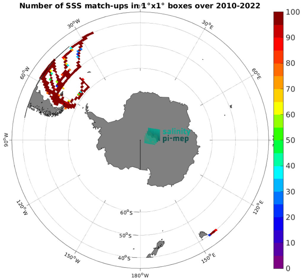
Figure 5: Number of SSS match-ups between TSG (CSIC-UTM) SSS and the CCI SSS L4 Merged-OI v4.41 - 30-day running (ESA) SSS product for the Roaring Forties and Furious Fifties Pi-MEP region over 1^\circ \times 1^\circ boxes and for the full satellite product period.
