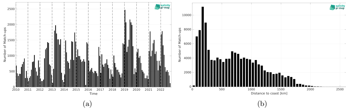
Figure 2: Number of match-ups between Marine mammals and CCI SSS L4 Merged-OI v4.41 - 30-day running (ESA) SSS as a function of time (a) and as function of the distance to coast (b) over the Roaring Forties and Furious Fifties Pi-MEP region and for the full satellite product period.
