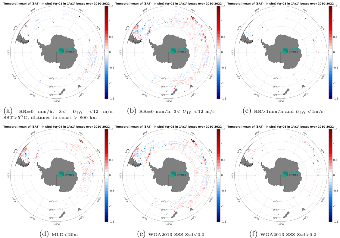
Figure 14: Temporal mean gridded over spatial boxes of size 1^\circ \times 1^\circ of \Delta SSS (CCI SSS L4 Merged-OI v4.41 - 30-day running (ESA) - Marine mammals) for 6 different subdatasets corresponding to:RR=0 mm/h, 3 < U_{10} < 12 m/s, SST >5^\circ C, distance to coast > 800 km (a), RR=0 mm/h, 3 < U_{10} < 12 m/s (b), RR >1 mm/h and U_{10} < 4 m/s (c),MLD <20 m (d),WOA2013 SSS Std <0.2 (e),WOA2013 SSS Std >0.2 (f).
