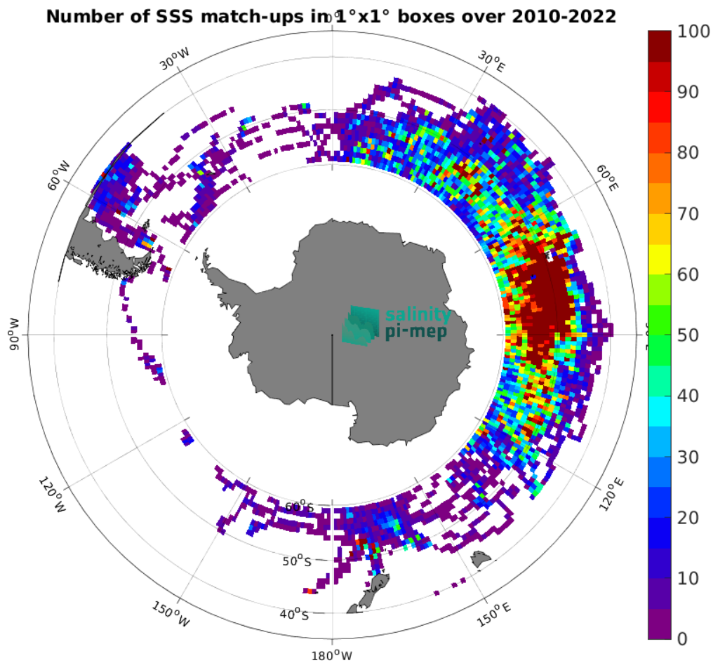
Figure 5: Number of SSS match-ups between Marine mammals SSS and the CCI SSS L4 Merged-OI v4.41 - 30-day running (ESA) SSS product for the Roaring Forties and Furious Fifties Pi-MEP region over 1^{\circ} \times 1^{\circ} boxes and for the full satellite product period.
