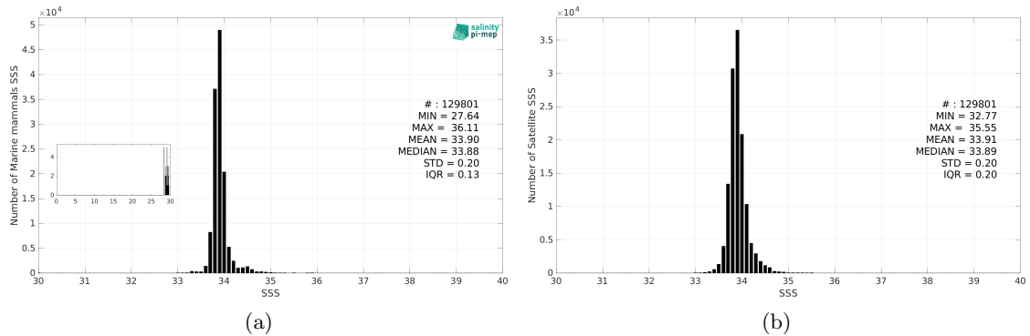
Figure 3: Histograms of SSS from Marine mammals (a) and CCI SSS L4 Merged-OI v4.41 - 30-day running (ESA) (b) considering all match-up pairs per bins of 0.1 over the Roaring Forties and Furious Fifties Pi-MEP region and for the full satellite product period.
