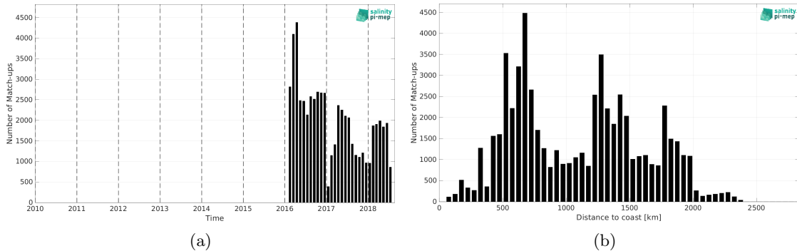
Figure 2: Number of match-ups between Surface drifters and CCI SSS L4 Merged-OI v4.41 - 30-day running (ESA) SSS as a function of time (a) and as function of the distance to coast (b) over the Roaring Forties and Furious Fifties Pi-MEP region and for the full satellite product period.
