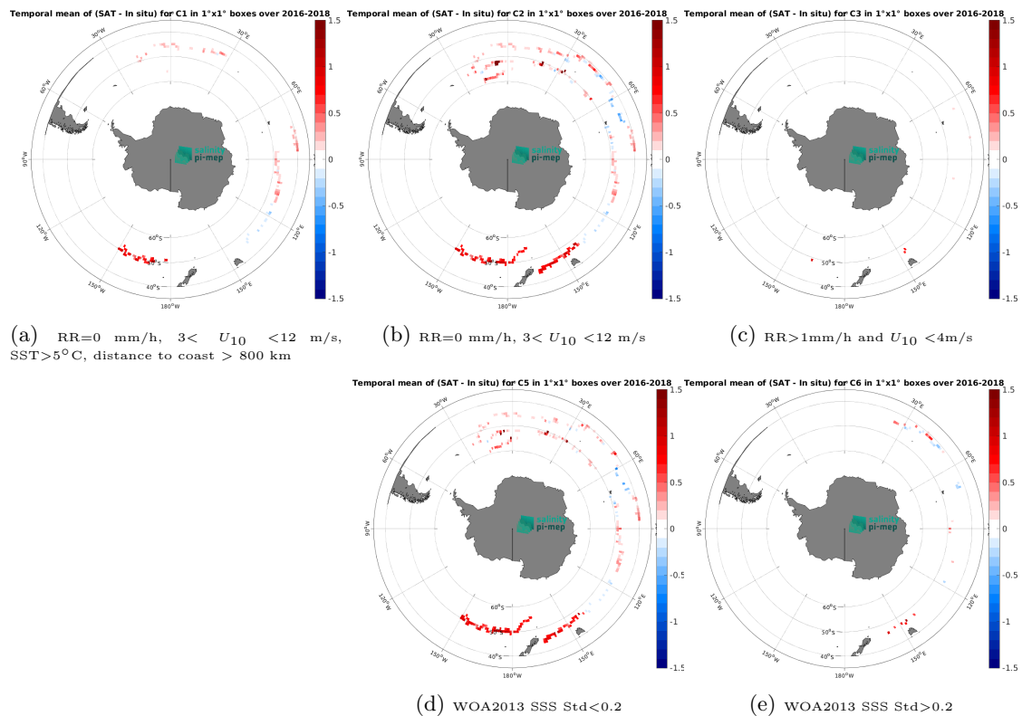
Figure 13: Temporal mean gridded over spatial boxes of size 1^\circ \times 1^\circ of \Delta\text{SSS} (CCI SSS L4 Merged-OI v4.41 - 30-day running (ESA) - Surface drifters) for 5 different subdatasets corresponding to:RR=0 mm/h, 3 < U_{10} < 12 m/s, SST >5^\circ\text{C} , distance to coast > 800 km (a), RR=0 mm/h, 3 < U_{10} < 12 m/s (b), RR >1 mm/h and U_{10} < 4 m/s (c), WOA2013 SSS Std <0.2 (d), WOA2013 SSS Std >0.2 (e).
