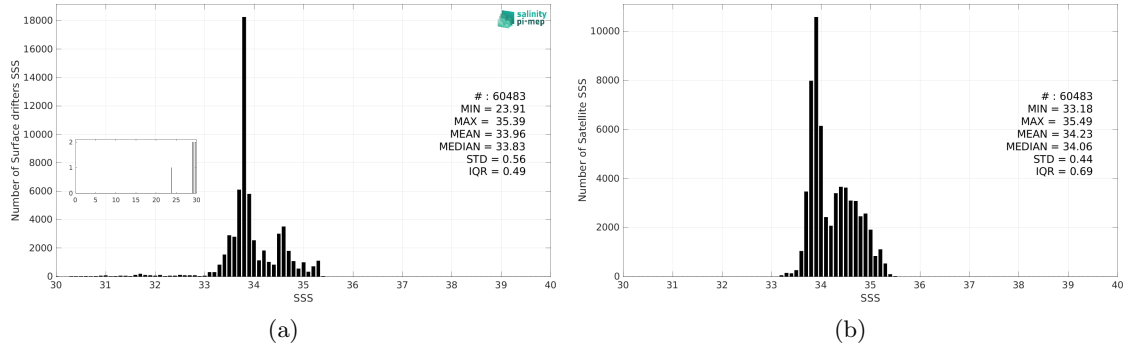
Figure 3: Histograms of SSS from Surface drifters (a) and CCI SSS L4 Merged-OI v4.41 - 30-day running (ESA) (b) considering all match-up pairs per bins of 0.1 over the Roaring Forties and Furious Fifties Pi-MEP region and for the full satellite product period.
