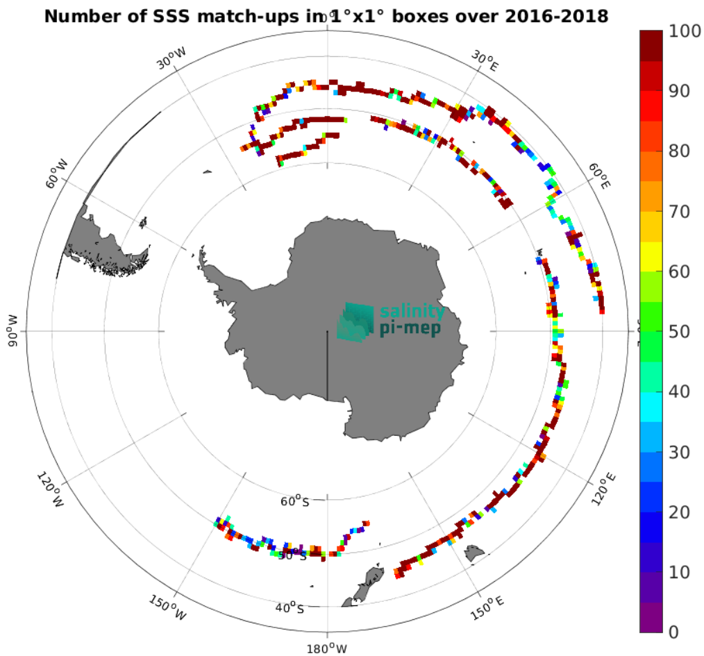
Figure 4: Number of SSS match-ups between Surface drifters SSS and the CCI SSS L4 Merged-OI v4.41 - 30-day running (ESA) SSS product for the Roaring Forties and Furious Fifties Pi-MEP region over 1^\circ \times 1^\circ boxes and for the full satellite product period.
