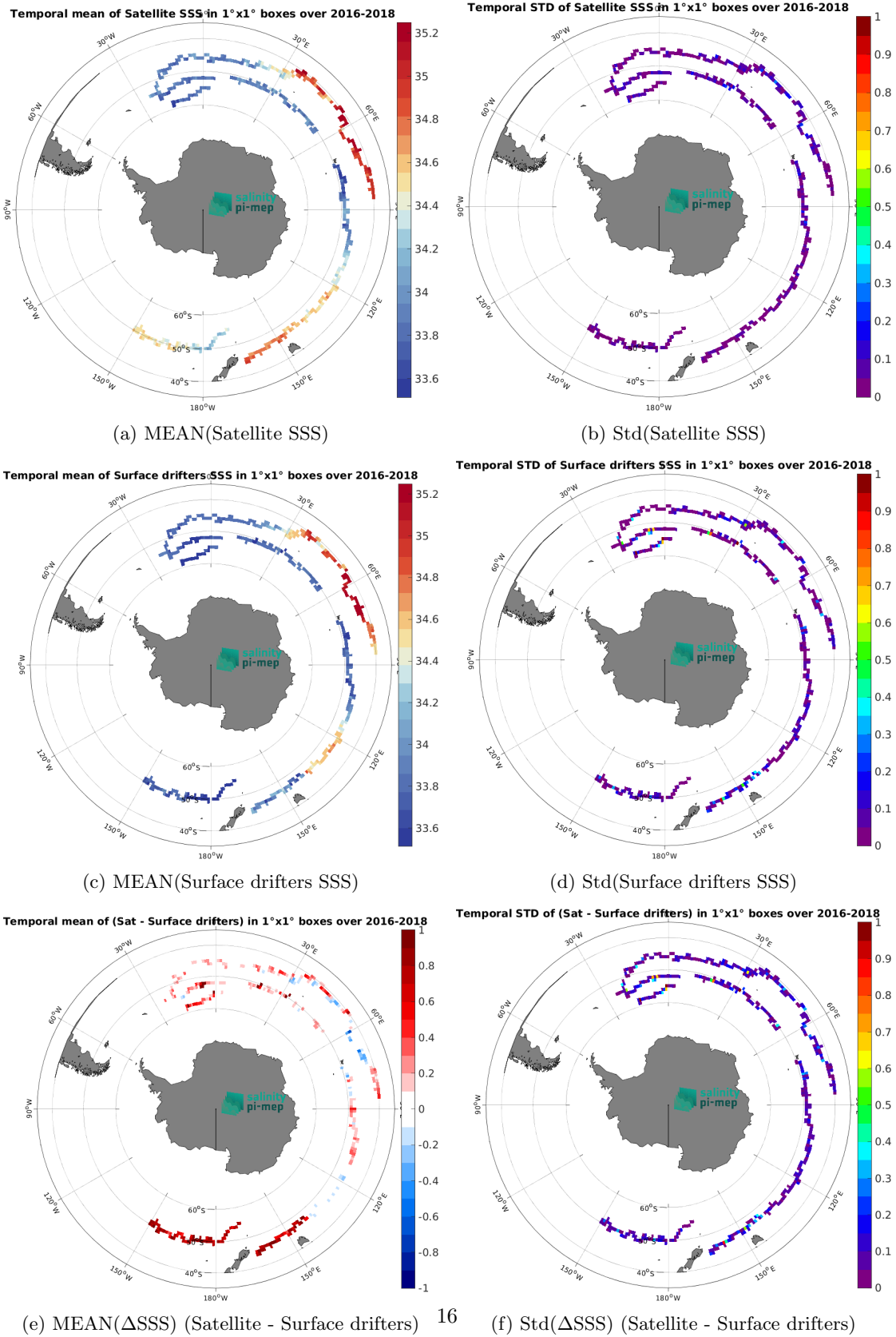
Figure 6: Temporal mean (left) and Std (right) of SSS from CCI SSS L4 Merged-OI v4.41 - 30-day running (ESA) (top), Surface drifters (middle), and of \Delta SSS (Satellite - Surface drifters). Only match-up pairs are used to generate these maps.
