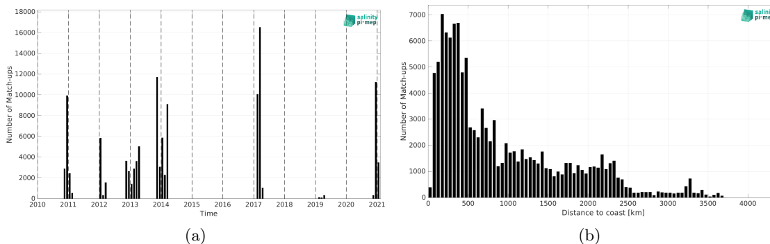
Figure 1: Number of match-ups between TSG (GOSUD-Sailing-ship) and CCI SSS L4 Merged-OI v4.4 - 7-day running (ESA) SSS as a function of time (a) and as function of the distance to coast (b) over the Roaring Forties and Furious Fifties Pi-MEP region and for the full satellite product period.
