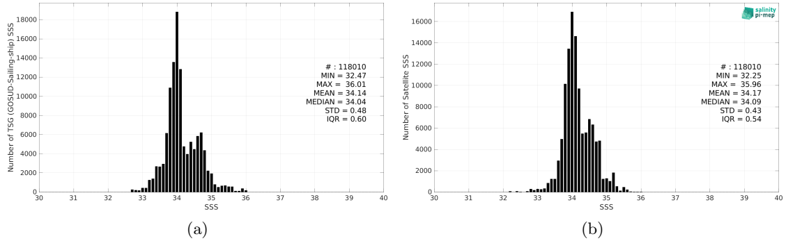
Figure 2: Histograms of SSS from TSG (GOSUD-Sailing-ship) (a) and CCI SSS L4 Merged-OI v4.4 - 7-day running (ESA) (b) considering all match-up pairs per bins of 0.1 over the Roaring Forties and Furious Fifties Pi-MEP region and for the full satellite product period.
