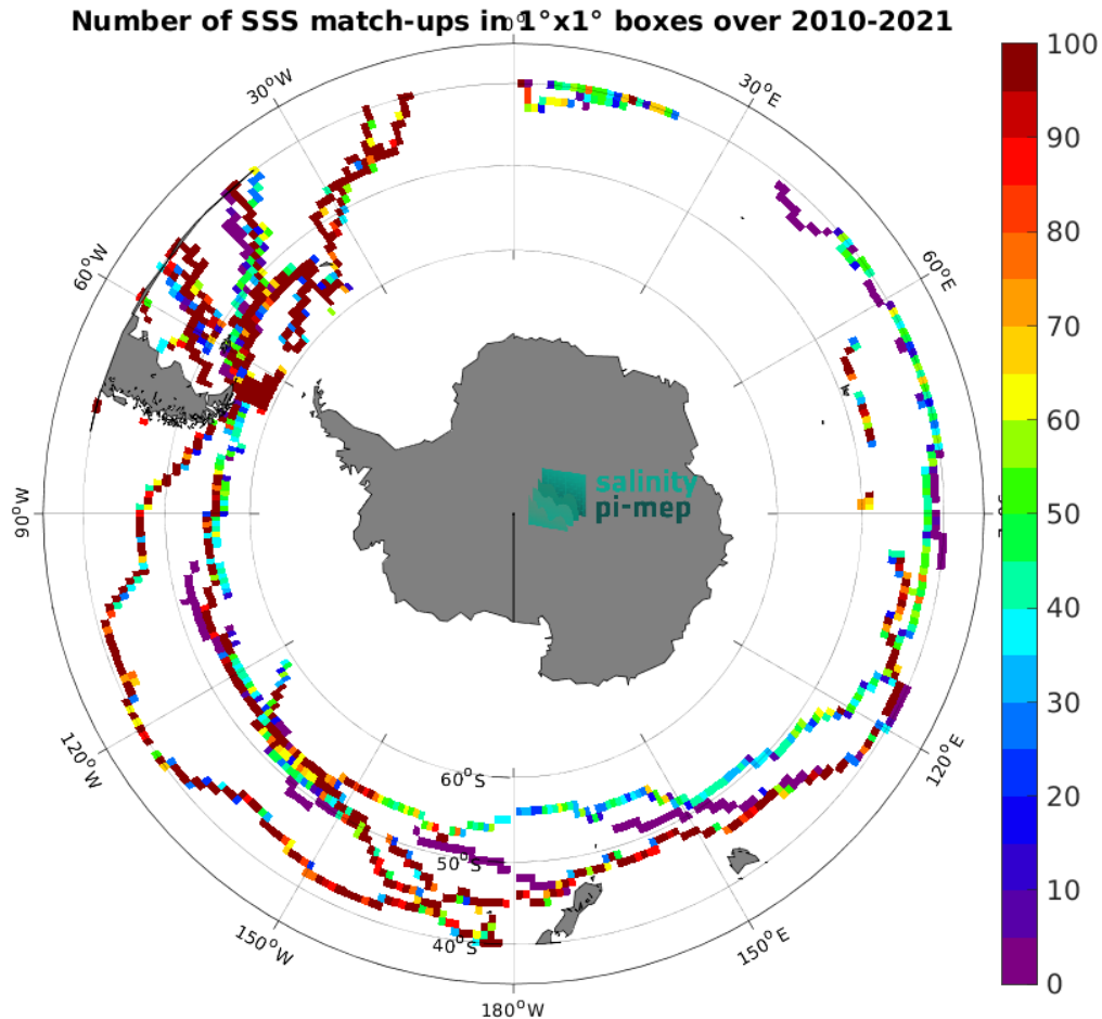
Figure 4: Number of SSS match-ups between TSG (GOSUD-Sailing-ship) SSS and the CCI SSS L4 Merged-OI v4.4 - 7-day running (ESA) SSS product for the Roaring Forties and Furious Fifties Pi-MEP region over 1^\circ \times 1^\circ boxes and for the full satellite product period.
