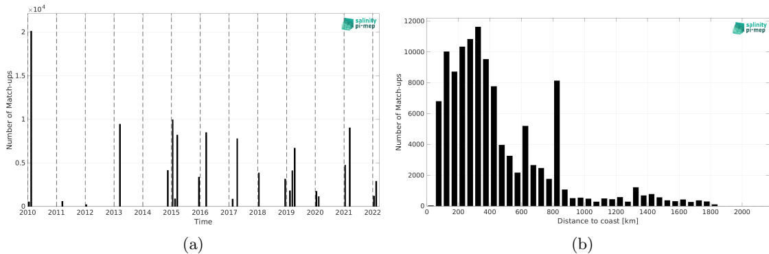
Figure 1: Number of match-ups between TSG (CSIC-UTM) and CCI SSS L4 Merged-OI v4.4 - 7-day running (ESA) SSS as a function of time (a) and as function of the distance to coast (b) over the Roaring Forties and Furious Fifties Pi-MEP region and for the full satellite product period.
