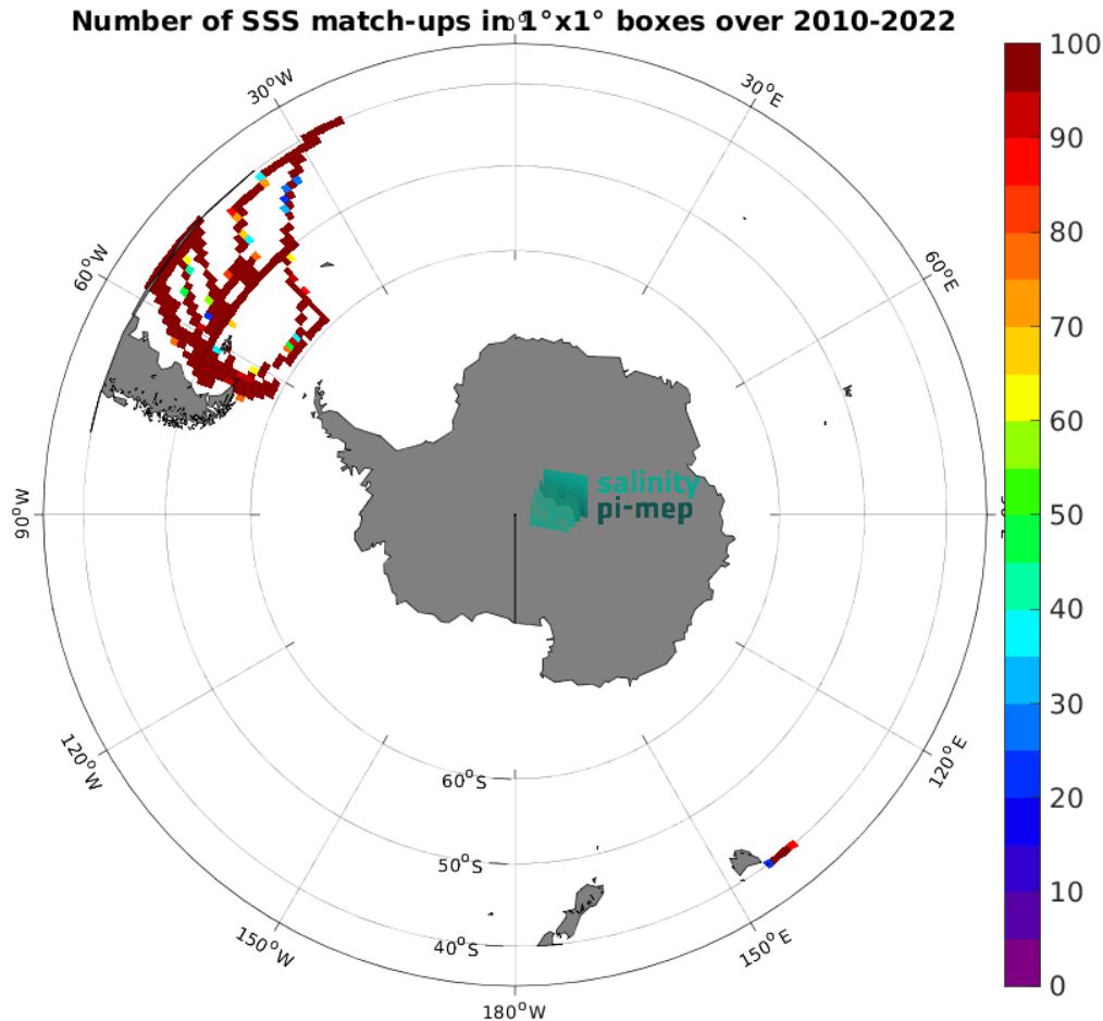
Figure 4: Number of SSS match-ups between TSG (CSIC-UTM) SSS and the CCI SSS L4 Merged-OI v4.4 - 7-day running (ESA) SSS product for the Roaring Forties and Furious Fifties Pi-MEP region over 1^\circ \times 1^\circ boxes and for the full satellite product period.
