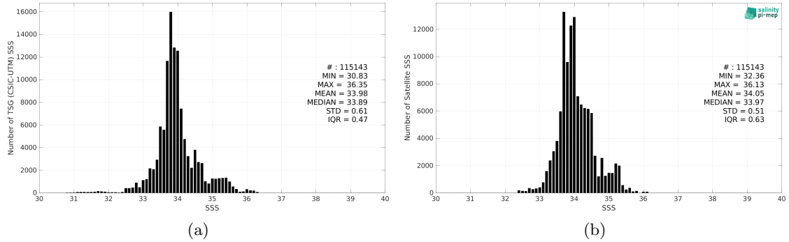
Figure 2: Histograms of SSS from TSG (CSIC-UTM) (a) and CCI SSS L4 Merged-OI v4.4 - 7-day running (ESA) (b) considering all match-up pairs per bins of 0.1 over the Roaring Forties and Furious Fifties Pi-MEP region and for the full satellite product period.
