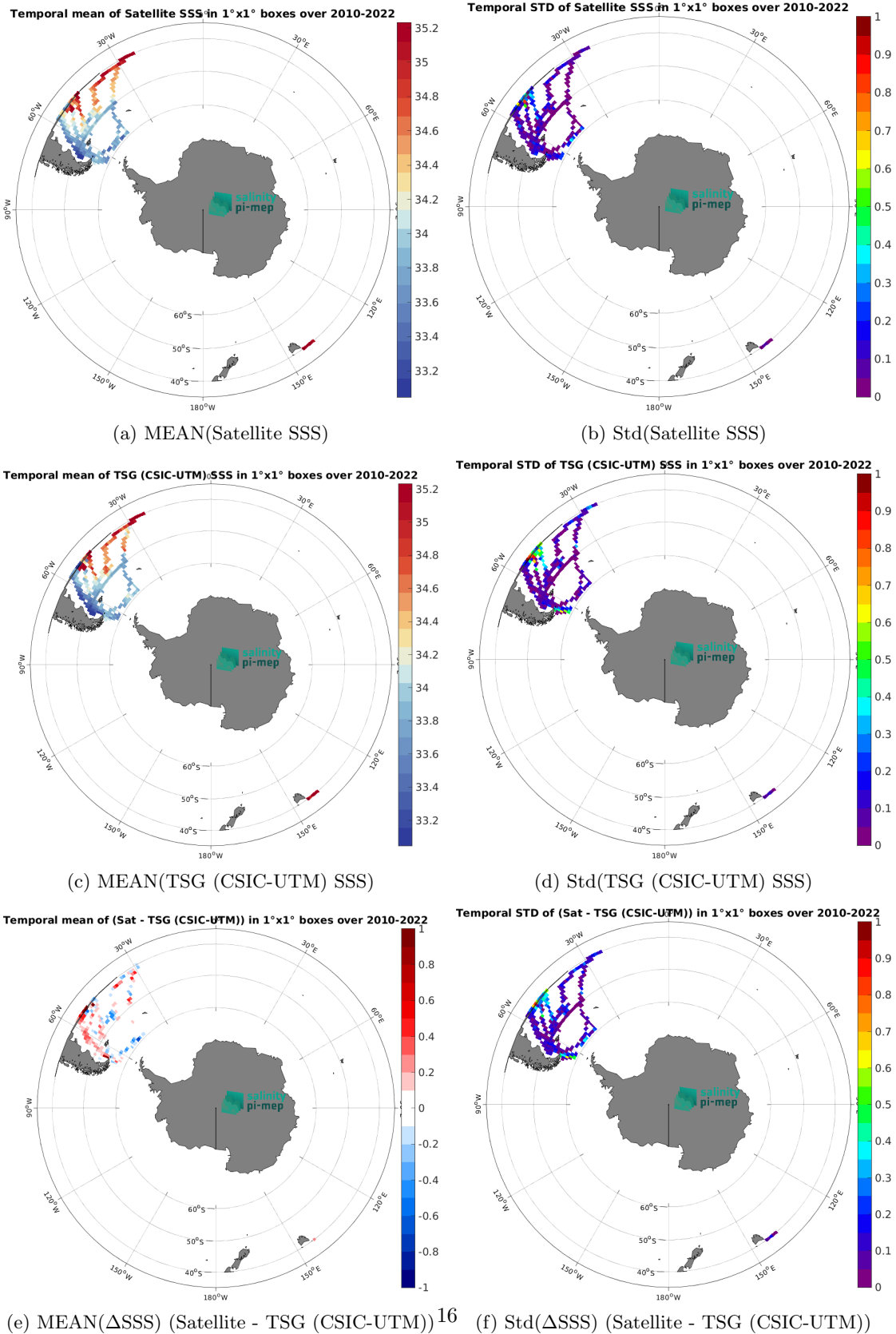
Figure 6: Temporal mean (left) and Std (right) of SSS from CCI SSS L4 Merged-OI v4.4 - 7-day running (ESA) (top), TSG (CSIC-UTM) (middle), and of \Delta SSS (Satellite - TSG (CSIC-UTM)). Only match-up pairs are used to generate these maps.
