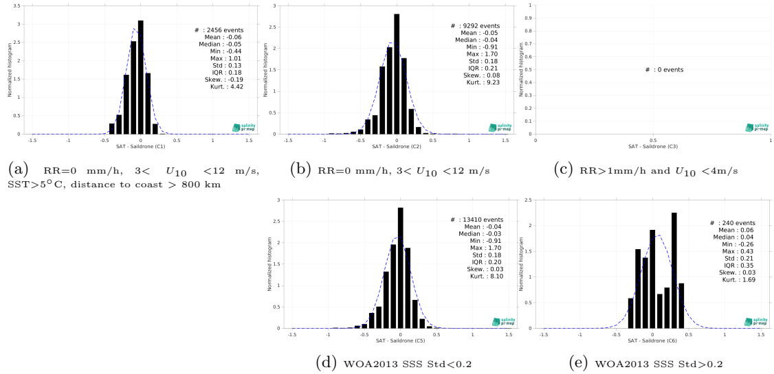
Figure 13: Normalized histogram of \Delta SSS (CCI SSS L4 Merged-OI v4.4 - 7-day running (ESA) - Saildrone) for 5 different subdatasets corresponding to: RR=0 mm/h, 3 < U_{10} < 12 m/s, SST > 5°C, distance to coast > 800 km (a), RR=0 mm/h, 3 < U_{10} < 12 m/s (b), RR > 1mm/h and U_{10} < 4 m/s (c), WOA2013 SSS Std < 0.2 (d), WOA2013 SSS Std > 0.2 (e).
