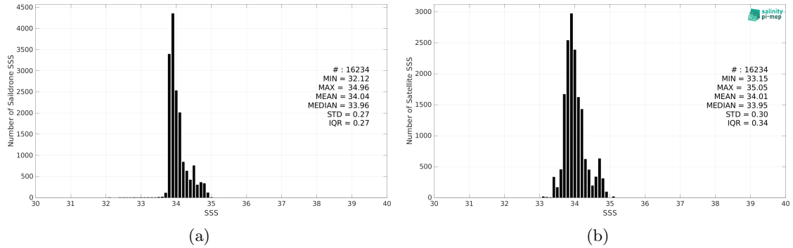
Figure 2: Histograms of SSS from Saildrone (a) and CCI SSS L4 Merged-OI v4.4 - 7-day running (ESA) (b) considering all match-up pairs per bins of 0.1 over the Roaring Forties and Furious Fifties Pi-MEP region and for the full satellite product period.
