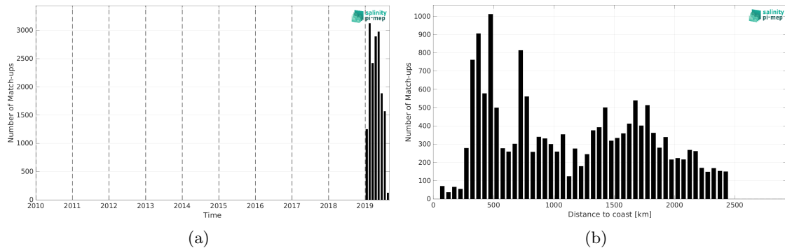
Figure 1: Number of match-ups between Saildrone and CCI SSS L4 Merged-OI v4.4 - 7-day running (ESA) SSS as a function of time (a) and as function of the distance to coast (b) over the Roaring Forties and Furious Fifties Pi-MEP region and for the full satellite product period.
