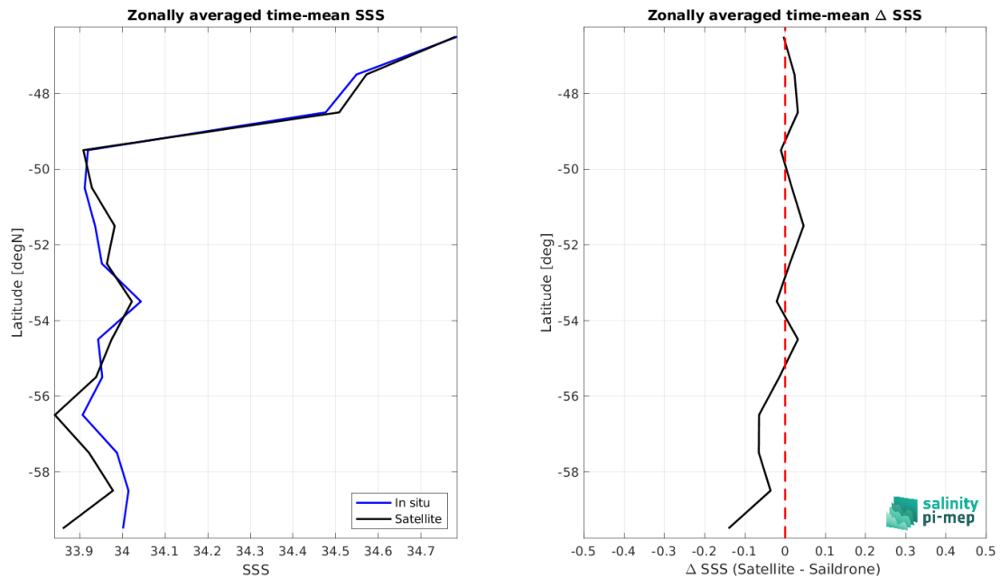
Figure 8: Left panel: Zonal mean SSS from CCI SSS L4 Merged-OI v4.4 - 7-day running (ESA) satellite product (black) and from Sairdronne (blue). Right panel: Zonal mean of \Delta SSS (Satellite - Sairdronne) for all the collected Pi-MEP match-up pairs estimated over the full satellite product period.
