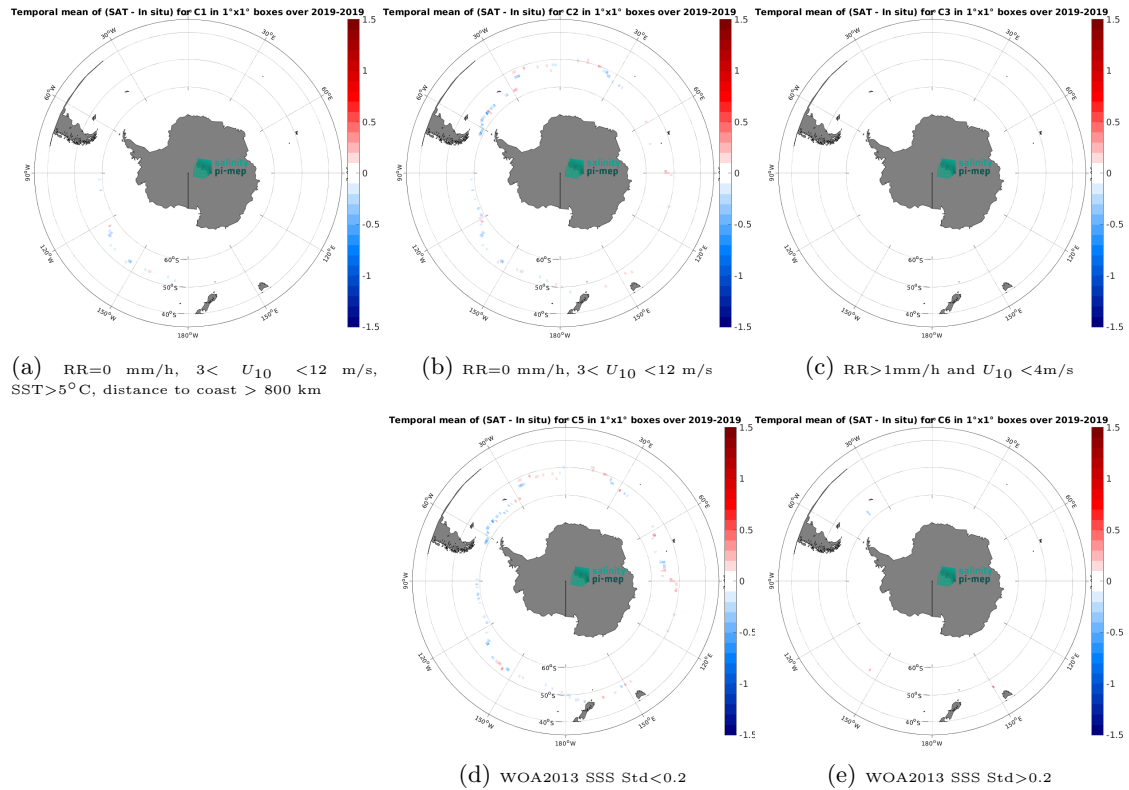
Figure 12: Temporal mean gridded over spatial boxes of size 1^{\circ}\times 1^{\circ} of \Delta\text{SSS} (CCI SSS L4 Merged-OI v4.4 - 7-day running (ESA) - Saildrone) for 5 different subdatasets corresponding to:RR=0 mm/h, 3 < U_{10} < 12 m/s, SST >5^{\circ}\text{C} , distance to coast > 800 km (a), RR=0 mm/h, 3 < U_{10} < 12 m/s (b), RR >1 mm/h and U_{10} < 4 m/s (c), WOA2013 SSS Std <0.2 (d), WOA2013 SSS Std >0.2 (e).
