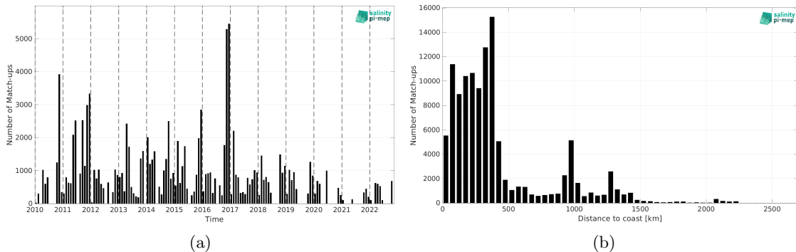
Figure 1: Number of match-ups between TSG (SAMOS) and CCI SSS L4 Merged-OI v4.4 - 30-day running (ESA) SSS as a function of time (a) and as function of the distance to coast (b) over the Roaring Forties and Furious Fifties Pi-MEP region and for the full satellite product period.
