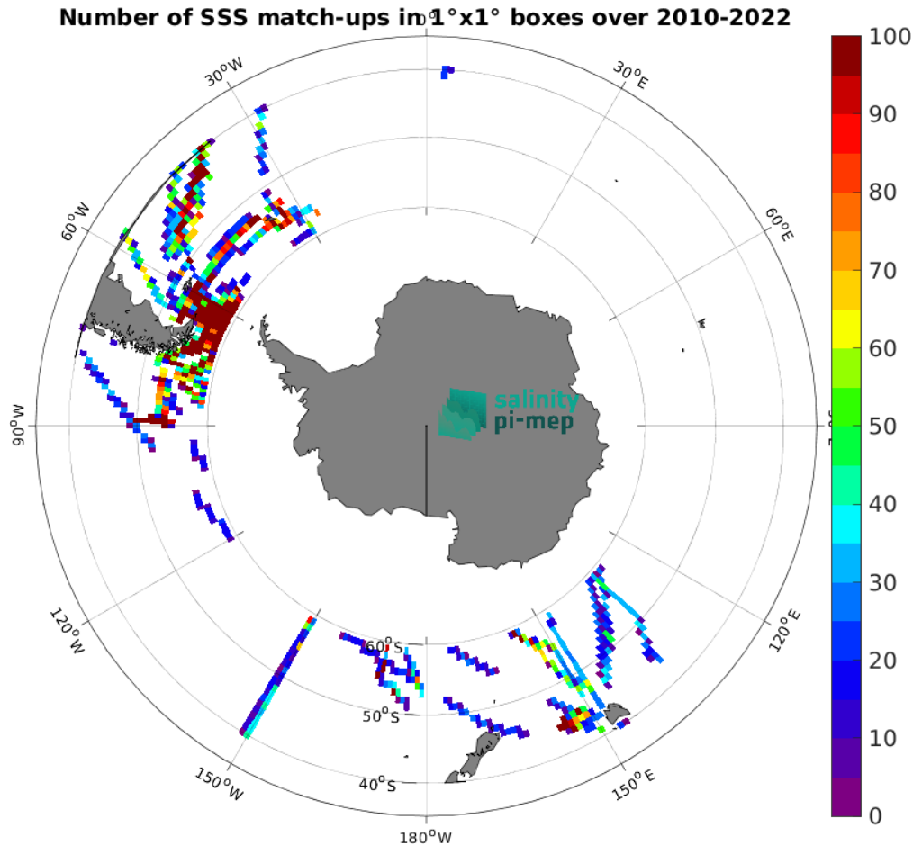
Figure 4: Number of SSS match-ups between TSG (SAMOS) SSS and the CCI SSS L4 Merged-OI v4.4 - 30-day running (ESA) SSS product for the Roaring Forties and Furious Fifties Pi-MEP region over 1^\circ \times 1^\circ boxes and for the full satellite product period.
