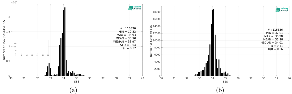
Figure 2: Histograms of SSS from TSG (SAMOS) (a) and CCI SSS L4 Merged-OI v4.4 - 30-day running (ESA) (b) considering all match-up pairs per bins of 0.1 over the Roaring Forties and Furious Fifties Pi-MEP region and for the full satellite product period.
