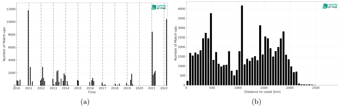
Figure 1: Number of match-ups between TSG (Polarstern) and CCI SSS L4 Merged-OI v4.4 - 30-day running (ESA) SSS as a function of time (a) and as function of the distance to coast (b) over the Roaring Forties and Furious Fifties Pi-MEP region and for the full satellite product period.
