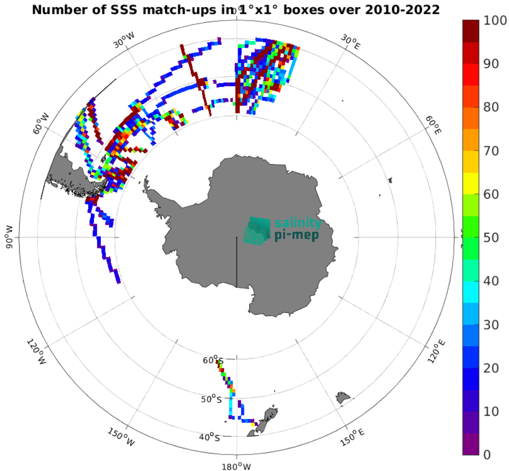
Figure 4: Number of SSS match-ups between TSG (Polarstern) SSS and the CCI SSS L4 Merged-OI v4.4 - 30-day running (ESA) SSS product for the Roaring Forties and Furious Fifties Pi-MEP region over 1^\circ \times 1^\circ boxes and for the full satellite product period.
