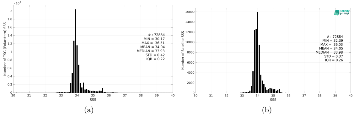
Figure 2: Histograms of SSS from TSG (Polarstern) (a) and CCI SSS L4 Merged-OI v4.4 - 30-day running (ESA) (b) considering all match-up pairs per bins of 0.1 over the Roaring Forties and Furious Fifties Pi-MEP region and for the full satellite product period.
