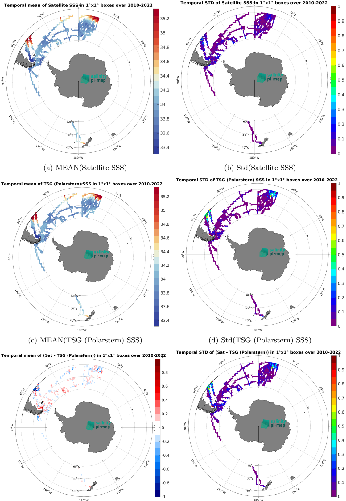
Figure 6: Temporal mean (left) and Std (right) of SSS from CCI SSS L4 Merged-OI v4.4 - 30-day running (ESA) (top), TSG (Polarstern) (middle), and of \Delta SSS (Satellite - TSG (Polarstern)). Only match-up pairs are used to generate these maps.
