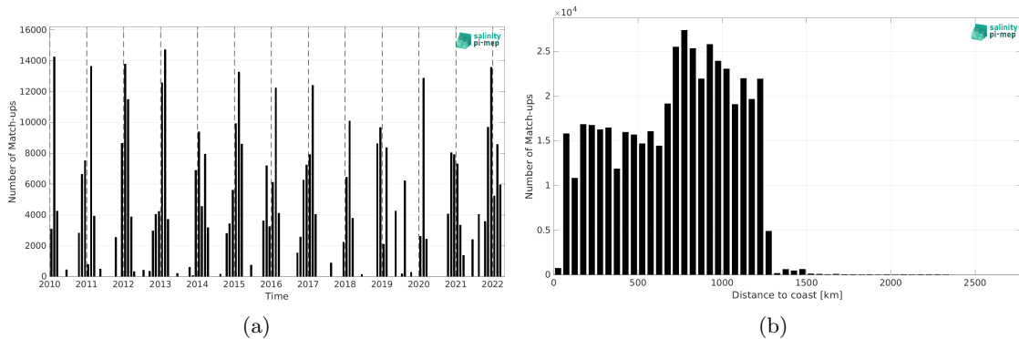
Figure 1: Number of match-ups between TSG (LEGOS-DM) and CCI SSS L4 Merged-OI v4.4 - 30-day running (ESA) SSS as a function of time (a) and as function of the distance to coast (b) over the Roaring Forties and Furious Fifties Pi-MEP region and for the full satellite product period.
