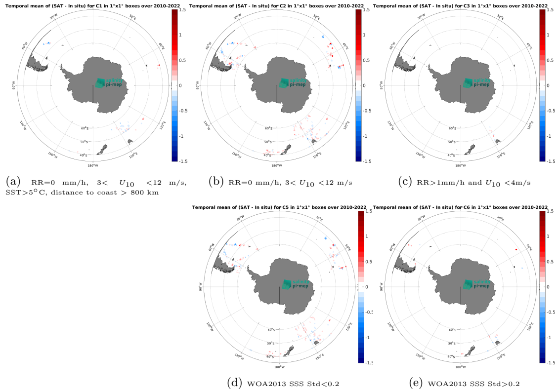
Figure 12: Temporal mean gridded over spatial boxes of size 1^{\circ}\times 1^{\circ} of \Delta\text{SSS} (CCI SSS L4 Merged-OI v4.4 - 30-day running (ESA) - TSG (LEGOS-DM)) for 5 different subdatasets corresponding to:RR=0 mm/h, 3 < U_{10} < 12 m/s, SST >5^{\circ}\text{C} , distance to coast > 800 km (a), RR=0 mm/h, 3 < U_{10} < 12 m/s (b), RR >1 mm/h and U_{10} < 4 m/s (c), WOA2013 SSS Std <0.2 (d), WOA2013 SSS Std >0.2 (e).
