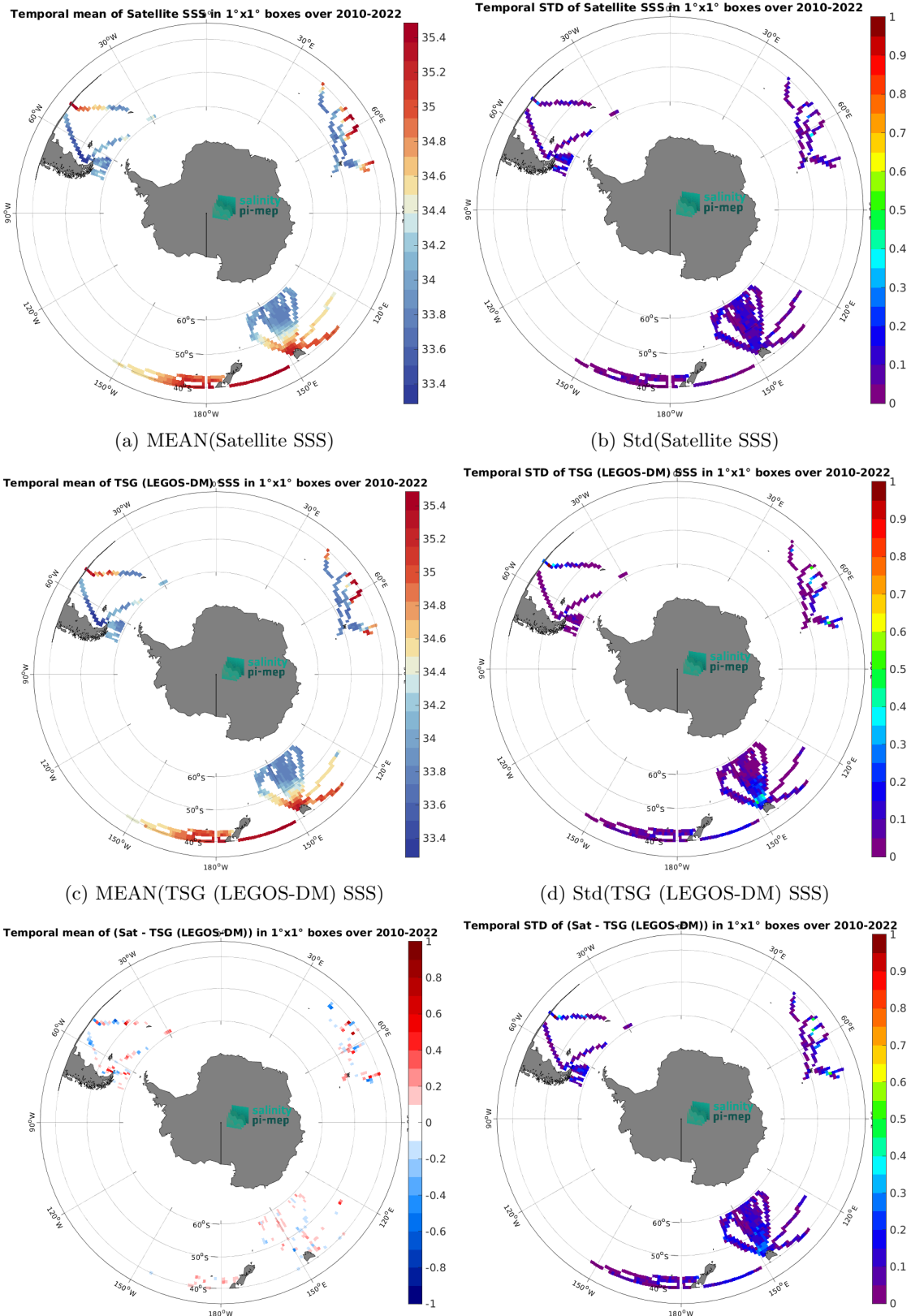
Figure 6: Temporal mean (left) and Std (right) of SSS from CCI SSS L4 Merged-OI v4.4 - 30-day running (ESA) (top), TSG (LEGOS-DM) (middle), and of \Delta SSS (Satellite - TSG (LEGOS-DM)). Only match-up pairs are used to generate these maps.
