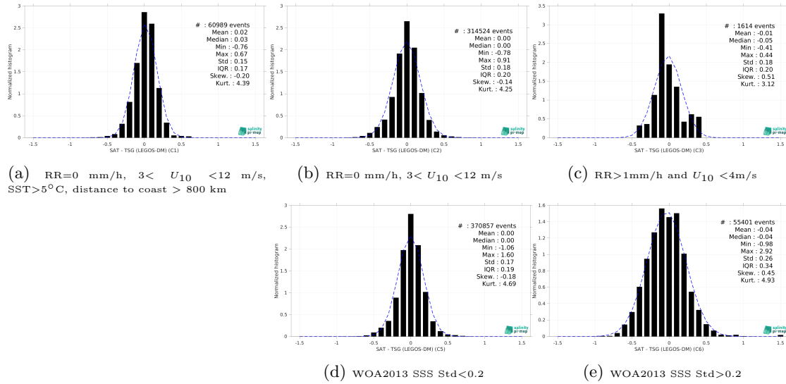
Figure 13: Normalized histogram of \Delta\text{SSS} (CCI SSS L4 Merged-OI v4.4 - 30-day running (ESA) - TSG (LEGOS-DM)) for 5 different subdatasets corresponding to: RR=0 mm/h, 3 < U_{10} < 12 m/s, SST>5°C, distance to coast > 800 km (a), RR=0 mm/h, 3 < U_{10} < 12 m/s (b), RR>1mm/h and U_{10} < 4 m/s (c), WOA2013 SSS Std<0.2 (d), WOA2013 SSS Std>0.2 (e).
