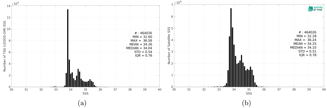
Figure 2: Histograms of SSS from TSG (LEGOS-DM) (a) and CCI SSS L4 Merged-OI v4.4 - 30-day running (ESA) (b) considering all match-up pairs per bins of 0.1 over the Roaring Forties and Furious Fifties Pi-MEP region and for the full satellite product period.
