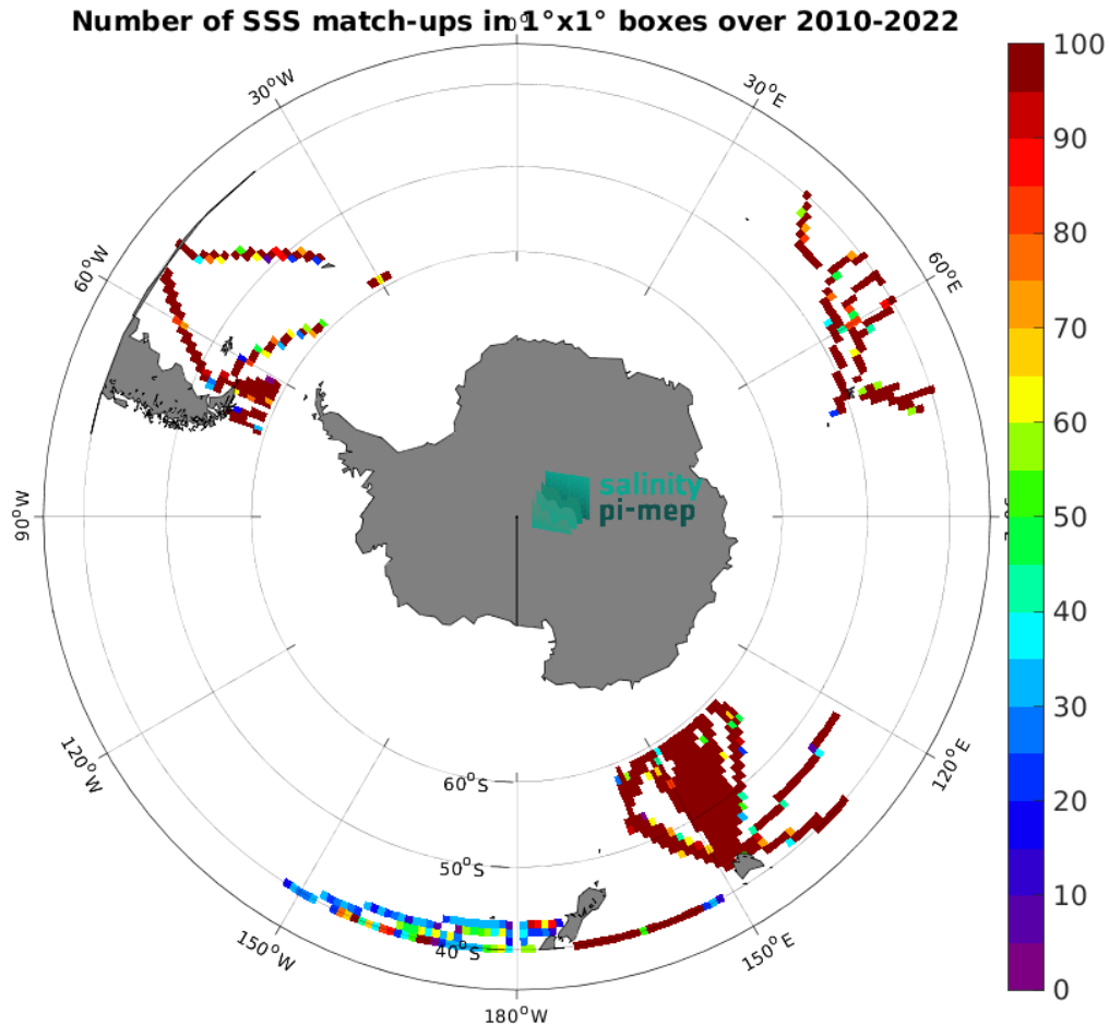
Figure 4: Number of SSS match-ups between TSG (LEGOS-DM) SSS and the CCI SSS L4 Merged-OI v4.4 - 30-day running (ESA) SSS product for the Roaring Forties and Furious Fifties Pi-MEP region over 1^\circ \times 1^\circ boxes and for the full satellite product period.
