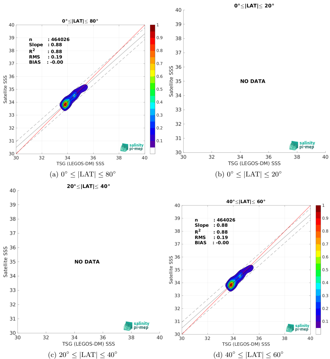
Figure 9: Contour maps of the concentration of CCI SSS L4 Merged-OI v4.4 - 30-day running (ESA) SSS (y-axis) versus TSG (LEGOS-DM) SSS (x-axis) at match-up pairs for different latitude bands. For each plot, the red line shows x=y . The black thin and dashed lines indicate a linear fit through the data cloud and the \pm 95\% confidence levels, respectively. The number match-up pairs n , the slope and R^2 coefficient of the linear fit, the root mean square (RMS) and the mean bias between satellite and in situ data are indicated for each latitude band in each plots.
