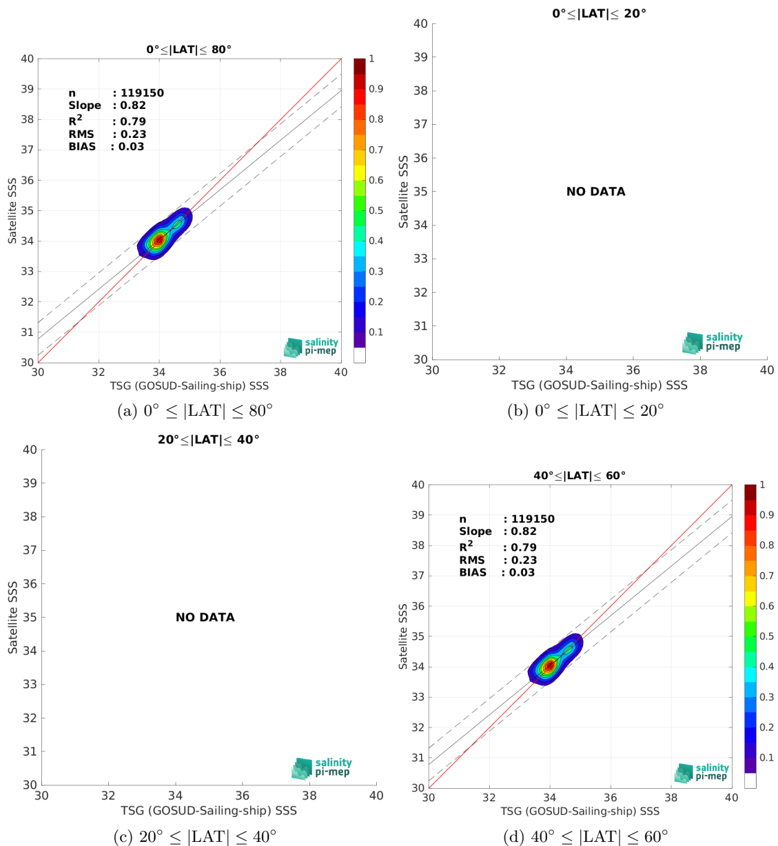
Figure 9: Contour maps of the concentration of CCI SSS L4 Merged-OI v4.4 - 30-day running (ESA) SSS (y-axis) versus TSG (GOSUD-Sailing-ship) SSS (x-axis) at match-up pairs for different latitude bands. For each plot, the red line shows x=y . The black thin and dashed lines indicate a linear fit through the data cloud and the \pm 95\% confidence levels, respectively. The number match-up pairs n , the slope and R^2 coefficient of the linear fit, the root mean square (RMS) and the mean bias between satellite and in situ data are indicated for each latitude band in each plots.
