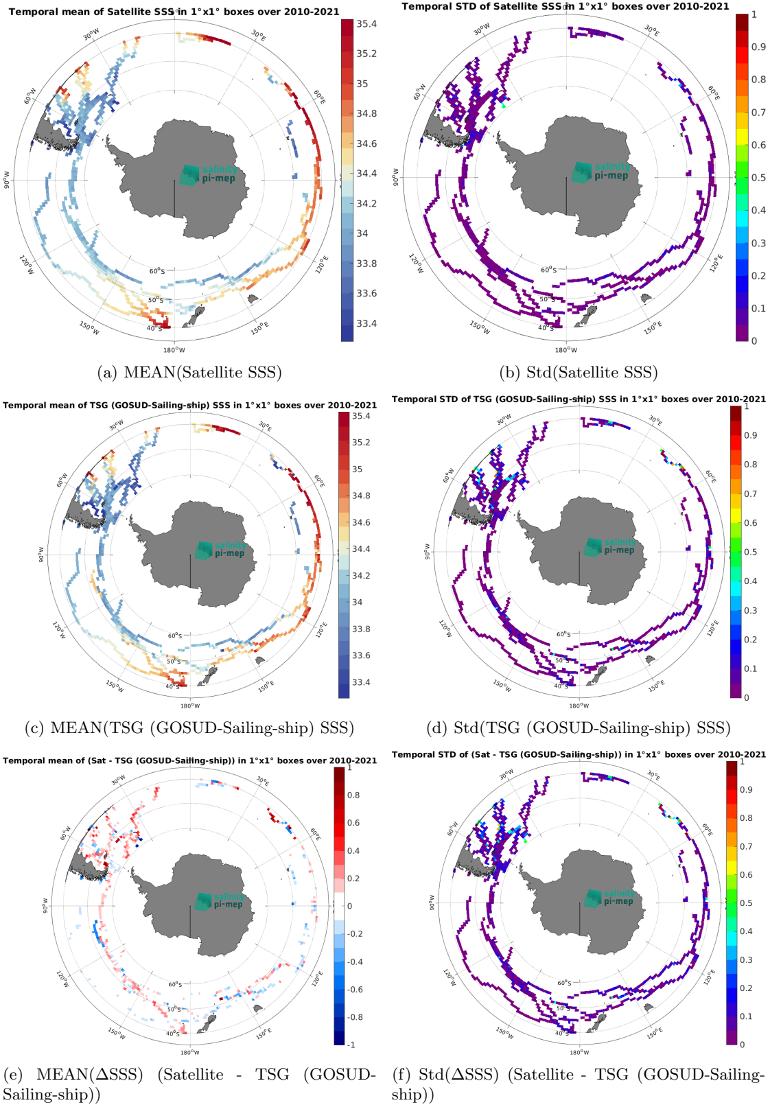
Figure 6: Temporal mean (left) and Std (right) of SSS from CCI SSS L4 Merged-OI v4.4 - 30-day running (ESA) (top), TSG (GOSUD-Sailing-ship) (middle), and of \Delta SSS (Satellite - TSG (GOSUD-Sailing-ship)). Only match-up pairs are used to generate these maps.
