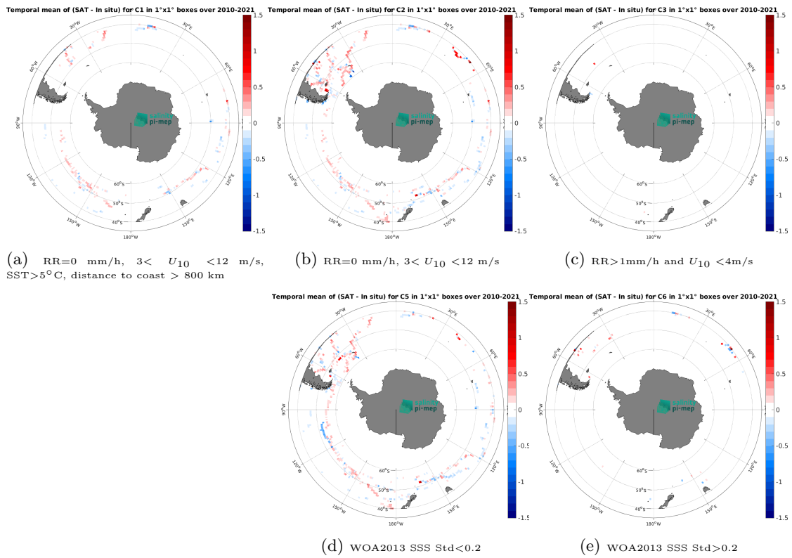
Figure 12: Temporal mean gridded over spatial boxes of size 1^\circ \times 1^\circ of \Delta SSS (CCI SSS L4 Merged-OI v4.4 - 30-day running (ESA) - TSG (GOSUD-Sailing-ship)) for 5 different subdatasets corresponding to:RR=0 mm/h, 3 < U_{10} < 12 m/s, SST>5°C, distance to coast > 800 km (a), RR=0 mm/h, 3 < U_{10} < 12 m/s (b), RR>1mm/h and U_{10} < 4 m/s (c), WOA2013 SSS Std<0.2 (d), WOA2013 SSS Std>0.2 (e).
