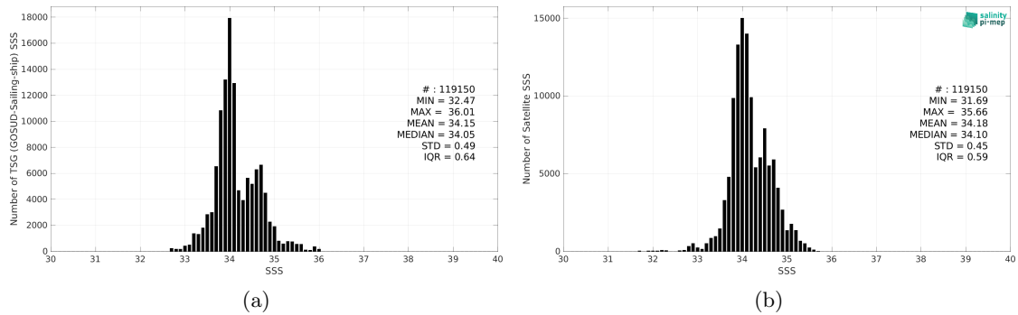
Figure 2: Histograms of SSS from TSG (GOSUD-Sailing-ship) (a) and CCI SSS L4 Merged-OI v4.4 - 30-day running (ESA) (b) considering all match-up pairs per bins of 0.1 over the Roaring Forties and Furious Fifties Pi-MEP region and for the full satellite product period.
