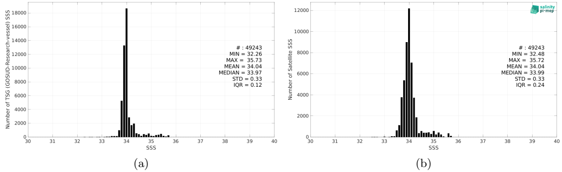
Figure 2: Histograms of SSS from TSG (GOSUD-Research-vessel) (a) and CCI SSS L4 Merged-OI v4.4 - 30-day running (ESA) (b) considering all match-up pairs per bins of 0.1 over the Roaring Forties and Furious Fifties Pi-MEP region and for the full satellite product period.
