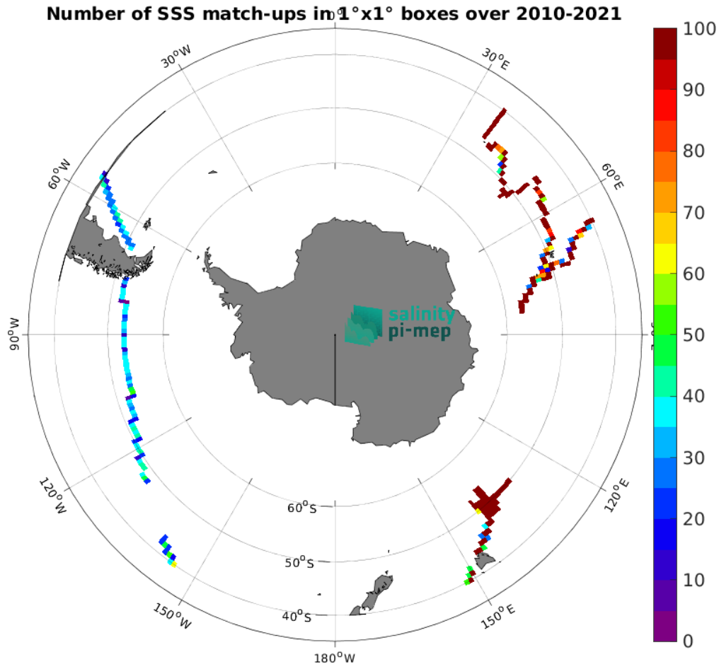
Figure 4: Number of SSS match-ups between TSG (GOSUD-Research-vessel) SSS and the CCI SSS L4 Merged-OI v4.4 - 30-day running (ESA) SSS product for the Roaring Forties and Furious Fifties Pi-MEP region over 1^\circ \times 1^\circ boxes and for the full satellite product period.
