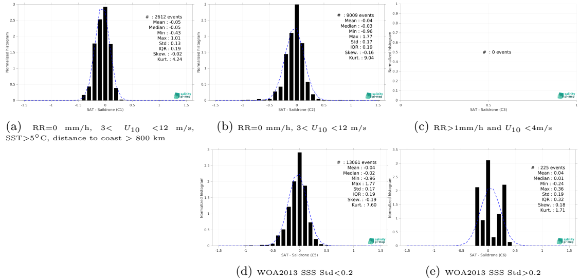
Figure 13: Normalized histogram of \Delta SSS (CCI SSS L4 Merged-OI v4.4 - 30-day running (ESA) - Saildrone) for 5 different subdatasets corresponding to: RR=0 mm/h, 3 < U_{10} < 12 m/s, SST > 5°C, distance to coast > 800 km (a), RR=0 mm/h, 3 < U_{10} < 12 m/s (b), RR > 1mm/h and U_{10} < 4 m/s (c), WOA2013 SSS Std < 0.2 (d), WOA2013 SSS Std > 0.2 (e).
