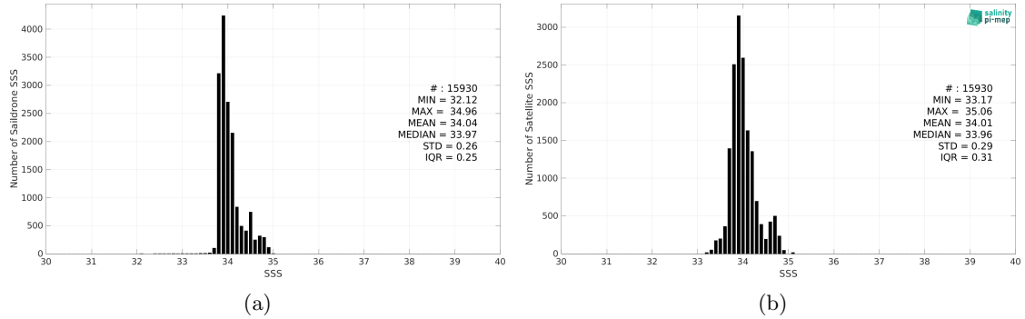
Figure 2: Histograms of SSS from Saildrone (a) and CCI SSS L4 Merged-OI v4.4 - 30-day running (ESA) (b) considering all match-up pairs per bins of 0.1 over the Roaring Forties and Furious Fifties Pi-MEP region and for the full satellite product period.
