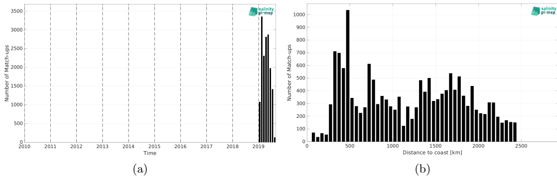
Figure 1: Number of match-ups between Saildrone and CCI SSS L4 Merged-OI v4.4 - 30-day running (ESA) SSS as a function of time (a) and as function of the distance to coast (b) over the Roaring Forties and Furious Fifties Pi-MEP region and for the full satellite product period.
