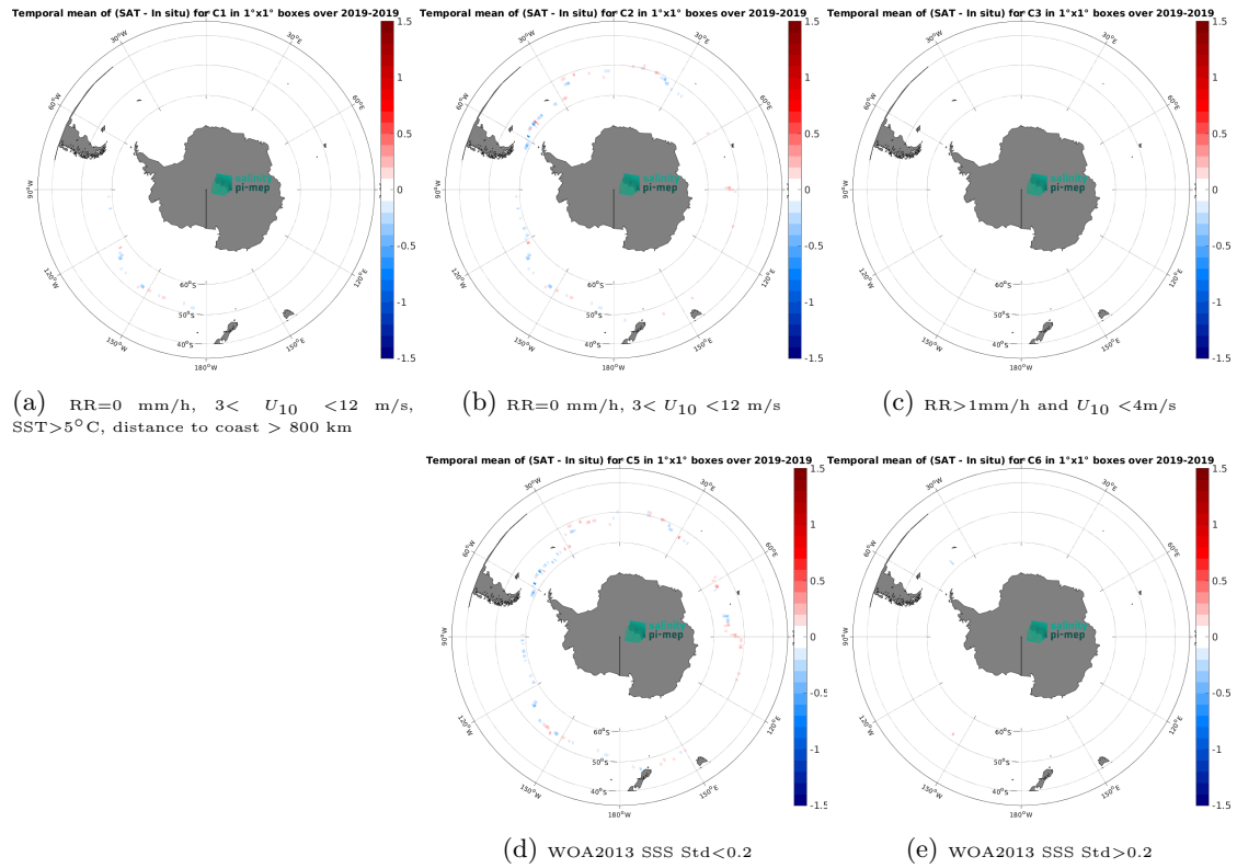
Figure 12: Temporal mean gridded over spatial boxes of size 1^{\circ}\times 1^{\circ} of \Delta\text{SSS} (CCI SSS L4 Merged-OI v4.4 - 30-day running (ESA) - Saildrone) for 5 different subdatasets corresponding to:RR=0 mm/h, 3 < U_{10} < 12 m/s, SST >5^{\circ}\text{C} , distance to coast > 800 km (a), RR=0 mm/h, 3 < U_{10} < 12 m/s (b), RR >1 mm/h and U_{10} < 4 m/s (c), WOA2013 SSS Std <0.2 (d), WOA2013 SSS Std >0.2 (e).
