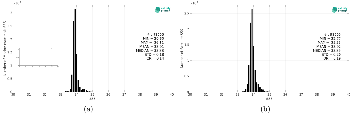
Figure 2: Histograms of SSS from Marine mammals (a) and CCI SSS L4 Merged-OI v4.4 - 30-day running (ESA) (b) considering all match-up pairs per bins of 0.1 over the Roaring Forties and Furious Fifties Pi-MEP region and for the full satellite product period.
