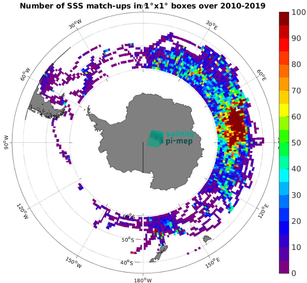
Figure 4: Number of SSS match-ups between Marine mammals SSS and the CCI SSS L4 Merged-OI v4.4 - 30-day running (ESA) SSS product for the Roaring Forties and Furious Fifties Pi-MEP region over 1^\circ \times 1^\circ boxes and for the full satellite product period.
