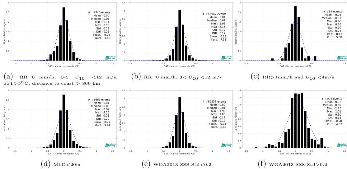
Figure 13: Normalized histogram of \Delta\text{SSS} (CCI SSS L4 Merged-OI v4.4 - 30-day running (ESA) - Marine mammals) for 6 different subdatasets corresponding to: RR=0 mm/h, 3 < U_{10} < 12 m/s, SST>5°C, distance to coast > 800 km (a), RR=0 mm/h, 3 < U_{10} < 12 m/s (b), RR>1mm/h and U_{10} < 4 m/s (c), MLD<20m (d), WOA2013 SSS Std<0.2 (e), WOA2013 SSS Std>0.2 (f).
