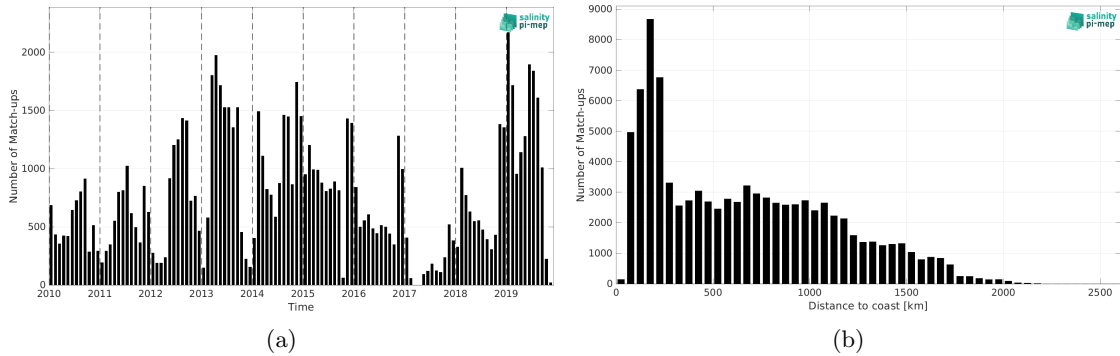
Figure 1: Number of match-ups between Marine mammals and CCI SSS L4 Merged-OI v4.4 - 30-day running (ESA) SSS as a function of time (a) and as function of the distance to coast (b) over the Roaring Forties and Furious Fifties Pi-MEP region and for the full satellite product period.
