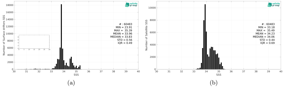
Figure 2: Histograms of SSS from Surface drifters (a) and CCI SSS L4 Merged-OI v4.4 - 30-day running (ESA) (b) considering all match-up pairs per bins of 0.1 over the Roaring Forties and Furious Fifties Pi-MEP region and for the full satellite product period.
