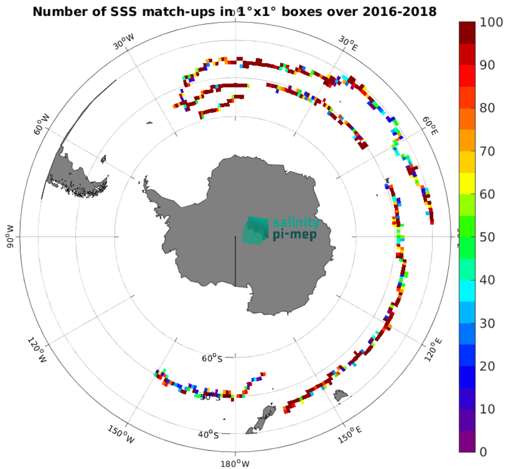
Figure 3: Number of SSS match-ups between Surface drifters SSS and the CCI SSS L4 Merged-OI v4.4 - 30-day running (ESA) SSS product for the Roaring Forties and Furious Fifties Pi-MEP region over 1^\circ \times 1^\circ boxes and for the full satellite product period.
