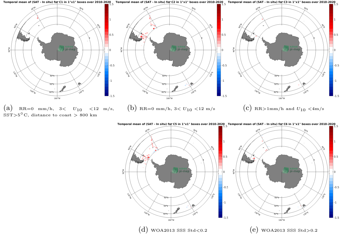
Figure 12: Temporal mean gridded over spatial boxes of size 1^{\circ}\times 1^{\circ} of \Delta\text{SSS} (CCI SSS L4 Merged-OI v3.2 - 7-day running (ESA) - TSG (SAMOS)) for 5 different subdatasets corresponding to:RR=0 mm/h, 3 < U_{10} < 12 m/s, SST >5^{\circ}\text{C} , distance to coast > 800 km (a), RR=0 mm/h, 3 < U_{10} < 12 m/s (b), RR >1 mm/h and U_{10} < 4 m/s (c), WOA2013 SSS Std <0.2 (d), WOA2013 SSS Std >0.2 (e).
