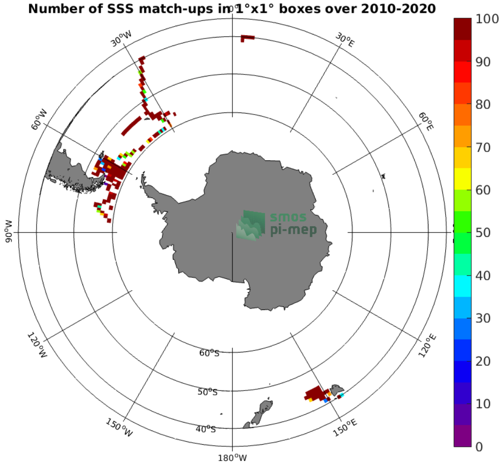
Figure 4: Number of SSS match-ups between TSG (SAMOS) SSS and the CCI SSS L4 Merged-OI v3.2 - 7-day running (ESA) SSS product for the Roaring Forties and Furious Fifties Pi-MEP region over 1^\circ \times 1^\circ boxes and for the full satellite product period.
