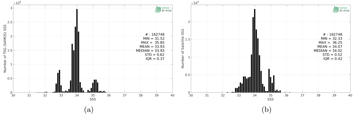
Figure 2: Histograms of SSS from TSG (SAMOS) (a) and CCI SSS L4 Merged-OI v3.2 - 7-day running (ESA) (b) considering all match-up pairs per bins of 0.1 over the Roaring Forties and Furious Fifties Pi-MEP region and for the full satellite product period.
