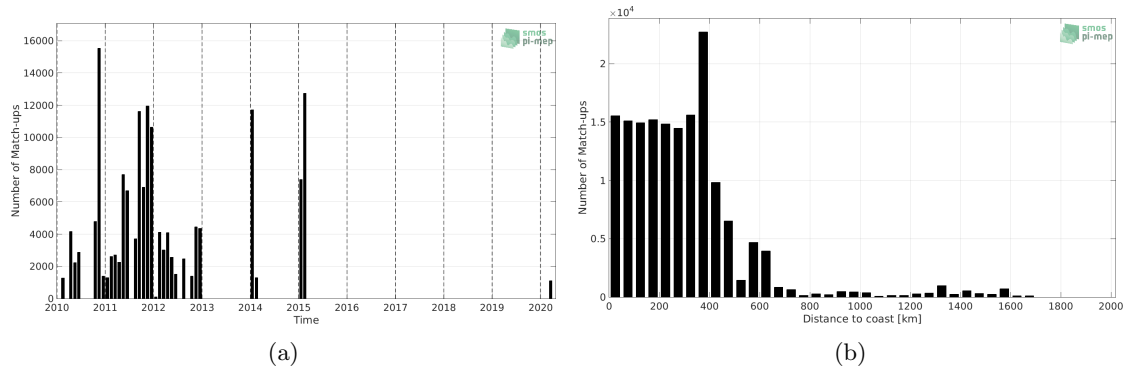
Figure 1: Number of match-ups between TSG (SAMOS) and CCI SSS L4 Merged-OI v3.2 - 7-day running (ESA) SSS as a function of time (a) and as function of the distance to coast (b) over the Roaring Forties and Furious Fifties Pi-MEP region and for the full satellite product period.
