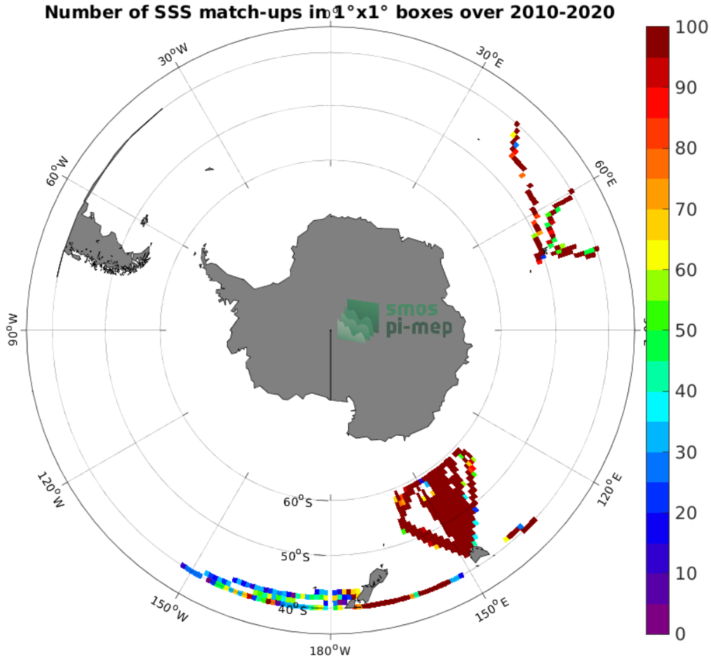
Figure 4: Number of SSS match-ups between TSG (LEGOS-DM) SSS and the CCI SSS L4 Merged-OI v3.2 - 7-day running (ESA) SSS product for the Roaring Forties and Furious Fifties Pi-MEP region over 1^\circ \times 1^\circ boxes and for the full satellite product period.
