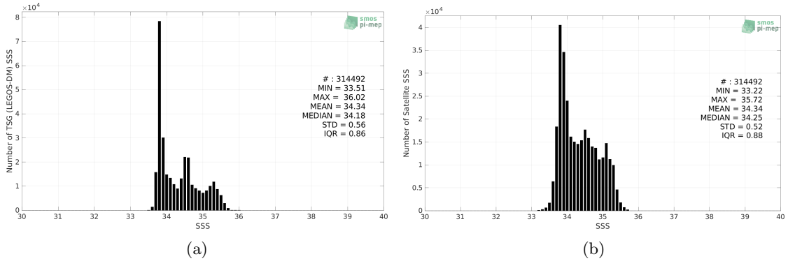
Figure 2: Histograms of SSS from TSG (LEGOS-DM) (a) and CCI SSS L4 Merged-OI v3.2 - 7-day running (ESA) (b) considering all match-up pairs per bins of 0.1 over the Roaring Forties and Furious Fifties Pi-MEP region and for the full satellite product period.
