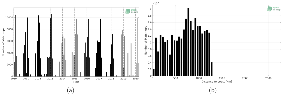
Figure 1: Number of match-ups between TSG (LEGOS-DM) and CCI SSS L4 Merged-OI v3.2 - 7-day running (ESA) SSS as a function of time (a) and as function of the distance to coast (b) over the Roaring Forties and Furious Fifties Pi-MEP region and for the full satellite product period.
