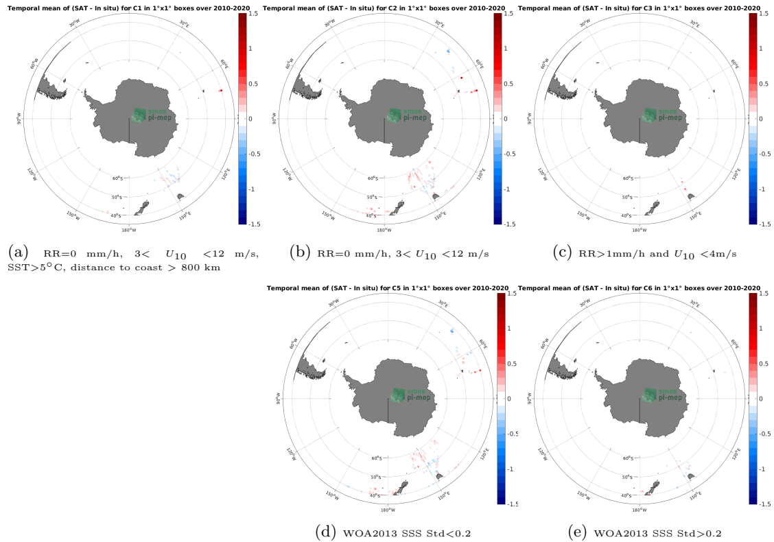
Figure 12: Temporal mean gridded over spatial boxes of size 1^{\circ}\times 1^{\circ} of \Delta\text{SSS} (CCI SSS L4 Merged-OI v3.2 - 7-day running (ESA) - TSG (LEGOS-DM)) for 5 different subdatasets corresponding to:RR=0 mm/h, 3 < U_{10} < 12 m/s, SST >5^{\circ}\text{C} , distance to coast > 800 km (a), RR=0 mm/h, 3 < U_{10} < 12 m/s (b), RR >1 mm/h and U_{10} < 4 m/s (c), WOA2013 SSS Std <0.2 (d), WOA2013 SSS Std >0.2 (e).
