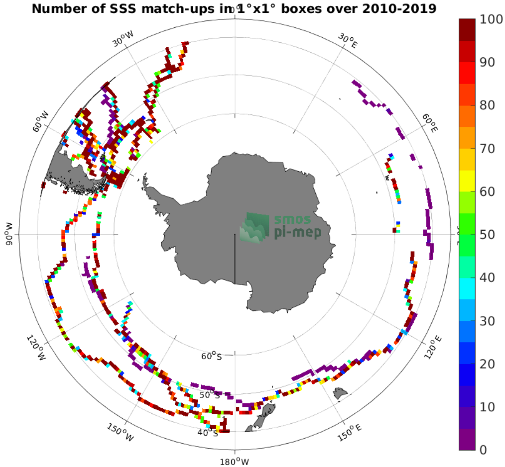
Figure 4: Number of SSS match-ups between TSG (GOSUD-Sailing-ship) SSS and the CCI SSS L4 Merged-OI v3.2 - 7-day running (ESA) SSS product for the Roaring Forties and Furious Fifties Pi-MEP region over 1^\circ \times 1^\circ boxes and for the full satellite product period.
