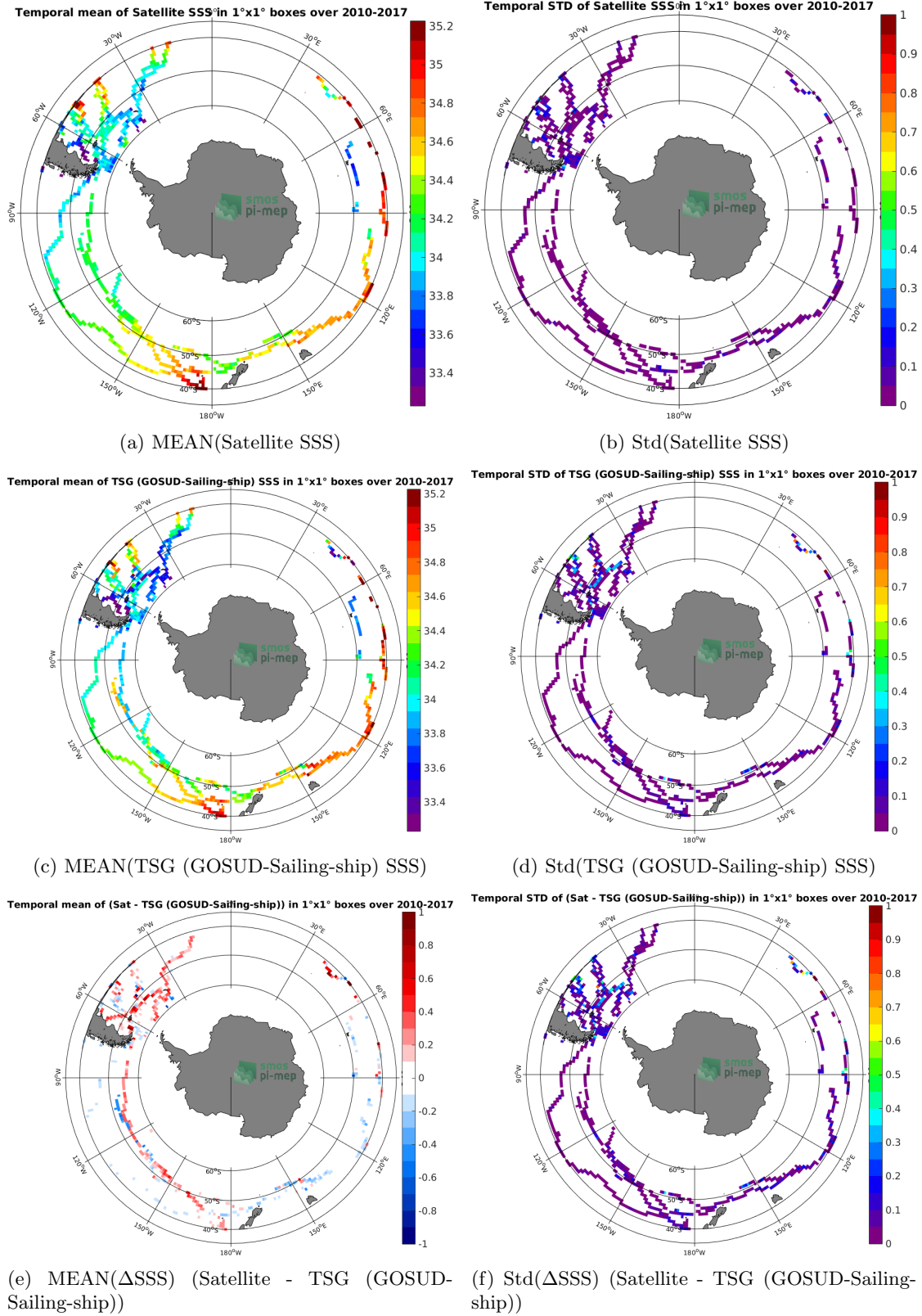
Figure 6: Temporal mean (left) and Std (right), of SSS from CCI SSS L4 Merged-OI v3.2 - 7-day running (ESA) (top), TSG (GOSUD-Sailing-ship) (middle), and of \Delta SSS (Satellite - TSG (GOSUD-Sailing-ship)). Only match-up pairs are used to generate these maps.
