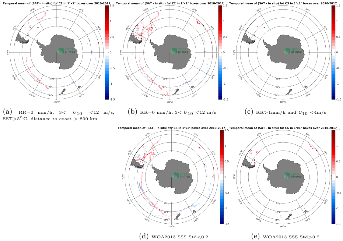
Figure 12: Temporal mean gridded over spatial boxes of size 1°x1° of \Delta SSS (CCI SSS L4 Merged-OI v3.2 - 7-day running (ESA) - TSG (GOSUD-Sailing-ship)) for 5 different subdatasets corresponding to:RR=0 mm/h, 3 < U_{10} < 12 m/s, SST>5°C, distance to coast > 800 km (a), RR=0 mm/h, 3 < U_{10} < 12 m/s (b), RR>1mm/h and U_{10} < 4 m/s (c), WOA2013 SSS Std<0.2 (d), WOA2013 SSS Std>0.2 (e).
