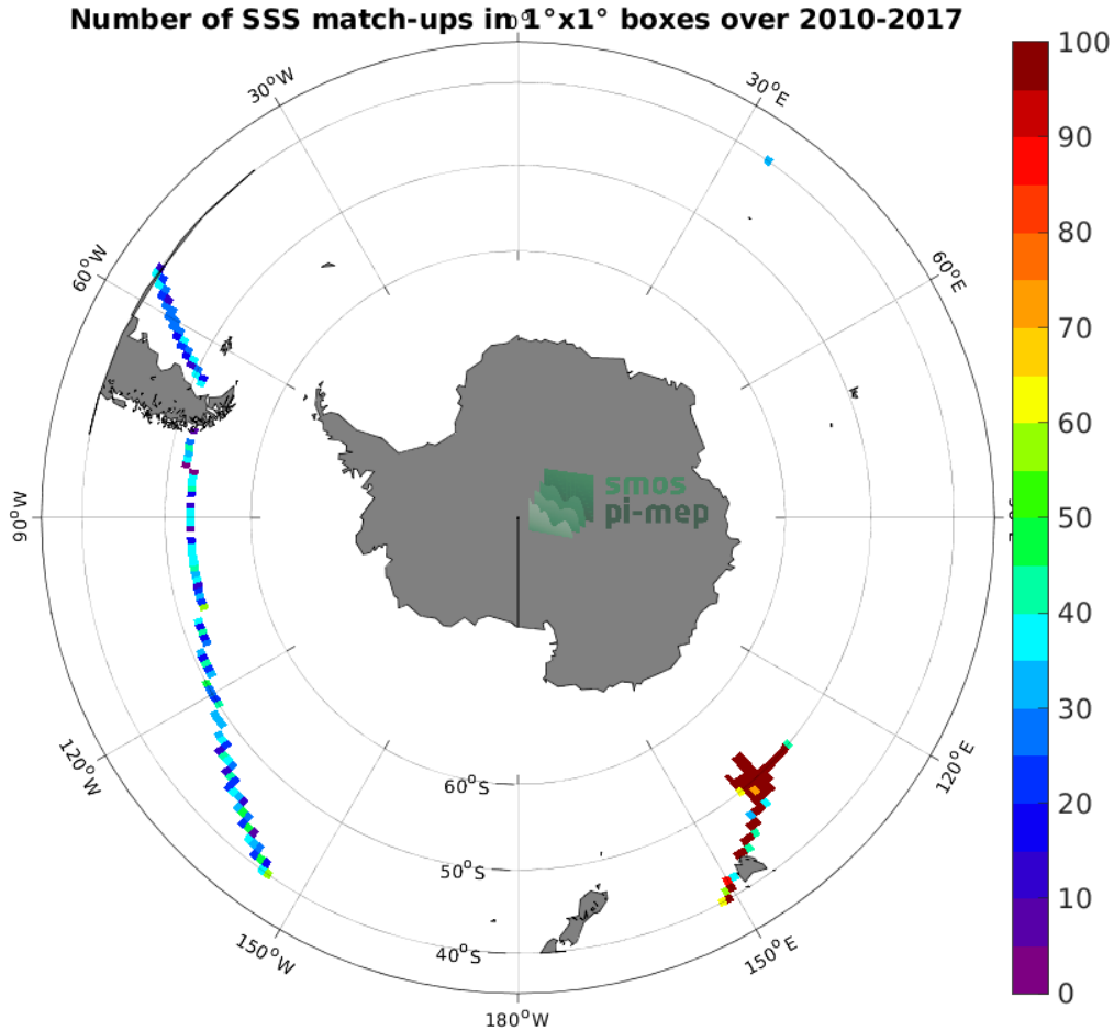
Figure 4: Number of SSS match-ups between TSG (GOSUD-Research-vessel) SSS and the CCI SSS L4 Merged-OI v3.2 - 7-day running (ESA) SSS product for the Roaring Forties and Furious Fifties Pi-MEP region over 1^\circ \times 1^\circ boxes and for the full satellite product period.
