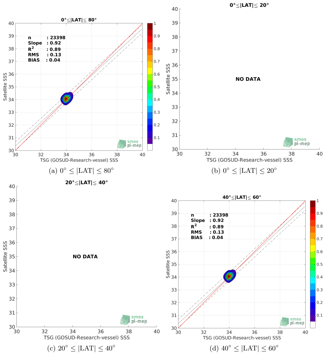
Figure 9: Contour maps of the concentration of CCI SSS L4 Merged-OI v3.2 - 7-day running (ESA) SSS ( y -axis) versus TSG (GOSUD-Research-vessel) SSS ( x -axis) at match-up pairs for different latitude bands. For each plot, the red line shows x=y . The black thin and dashed lines indicate a linear fit through the data cloud and the \pm 95\% confidence levels, respectively. The number match-up pairs n , the slope and R^2 coefficient of the linear fit, the root mean square (RMS) and the mean bias between satellite and in situ data are indicated for each latitude band in each plots.
