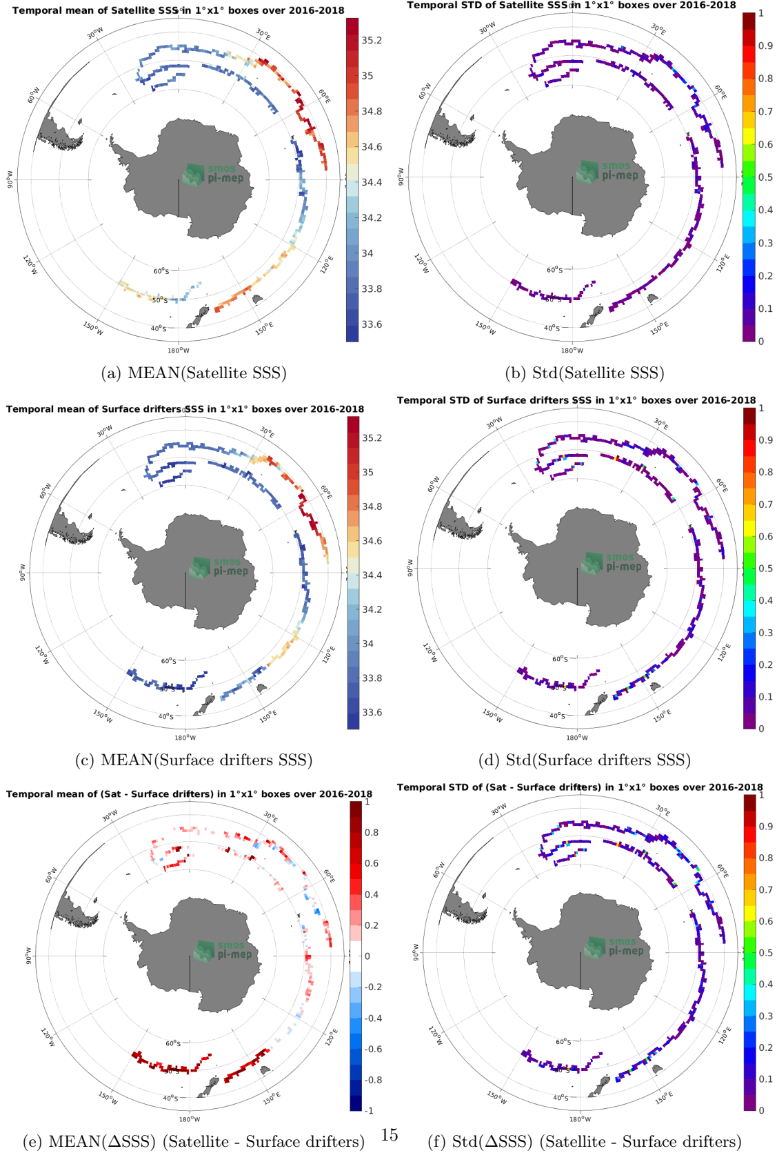
Figure 5: Temporal mean (left) and Std (right) of SSS from CCI SSS L4 Merged-OI v3.2 - 7-day running (ESA) (top), Surface drifters (middle), and of \Delta SSS (Satellite - Surface drifters). Only match-up pairs are used to generate these maps.
