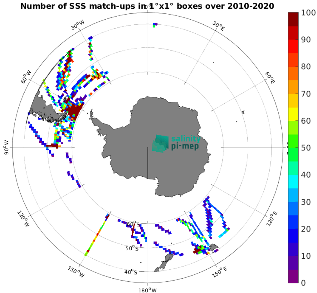
Figure 4: Number of SSS match-ups between TSG (SAMOS) SSS and the CCI SSS L4 Merged-OI v3.2 - 30-day running (ESA) SSS product for the Roaring Forties and Furious Fifties Pi-MEP region over 1^\circ \times 1^\circ boxes and for the full satellite product period.
