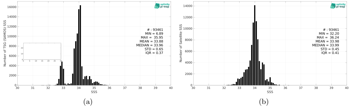
Figure 2: Histograms of SSS from TSG (SAMOS) (a) and CCI SSS L4 Merged-OI v3.2 - 30-day running (ESA) (b) considering all match-up pairs per bins of 0.1 over the Roaring Forties and Furious Fifties Pi-MEP region and for the full satellite product period.
