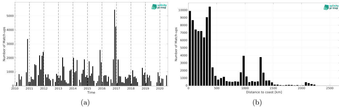
Figure 1: Number of match-ups between TSG (SAMOS) and CCI SSS L4 Merged-OI v3.2 - 30-day running (ESA) SSS as a function of time (a) and as function of the distance to coast (b) over the Roaring Forties and Furious Fifties Pi-MEP region and for the full satellite product period.
