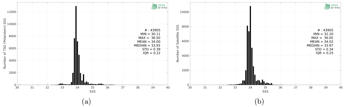
Figure 2: Histograms of SSS from TSG (Polarstern) (a) and CCI SSS L4 Merged-OI v3.2 - 30-day running (ESA) (b) considering all match-up pairs per bins of 0.1 over the Roaring Forties and Furious Fifties Pi-MEP region and for the full satellite product period.
