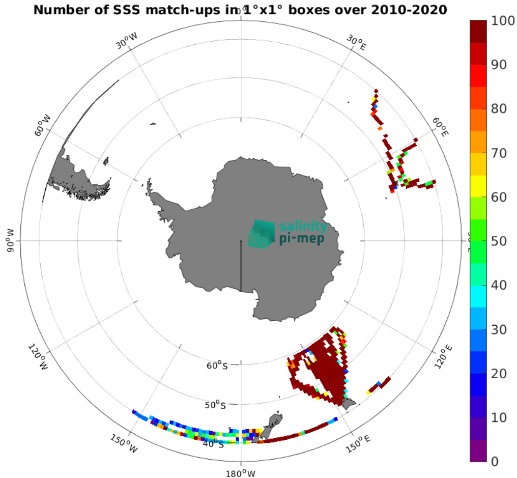
Figure 4: Number of SSS match-ups between TSG (LEGOS-DM) SSS and the CCI SSS L4 Merged-OI v3.2 - 30-day running (ESA) SSS product for the Roaring Forties and Furious Fifties Pi-MEP region over 1^\circ \times 1^\circ boxes and for the full satellite product period.
