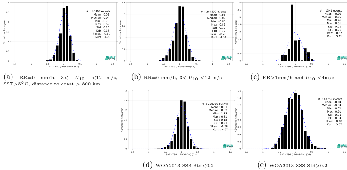
Figure 13: Normalized histogram of \Delta\text{SSS} (CCI SSS L4 Merged-OI v3.2 - 30-day running (ESA) - TSG (LEGOS-DM)) for 5 different subdatasets corresponding to: RR=0 mm/h, 3 < U_{10} < 12 m/s, SST>5°C, distance to coast > 800 km (a), RR=0 mm/h, 3 < U_{10} < 12 m/s (b), RR>1mm/h and U_{10} < 4 m/s (c), WOA2013 SSS Std<0.2 (d), WOA2013 SSS Std>0.2 (e).
