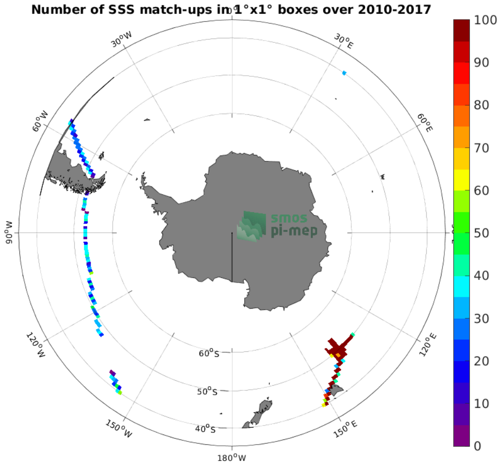
Figure 4: Number of SSS match-ups between TSG (GOSUD-Research-vessel) SSS and the CCI SSS L4 Merged-OI v3.2 - 30-day running (ESA) SSS product for the Roaring Forties and Furious Fifties Pi-MEP region over 1^\circ \times 1^\circ boxes and for the full satellite product period.
