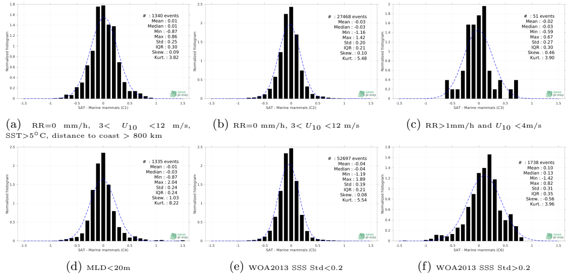
Figure 13: Normalized histogram of \Delta SSS (CCI SSS L4 Merged-OI v3.2 - 30-day running (ESA) - Marine mammals) for 6 different subdatasets corresponding to: RR=0 mm/h, 3 < U_{10} < 12 m/s, SST > 5°C, distance to coast > 800 km (a), RR=0 mm/h, 3 < U_{10} < 12 m/s (b), RR > 1mm/h and U_{10} < 4 m/s (c), MLD < 20m (d), WOA2013 SSS Std < 0.2 (e), WOA2013 SSS Std > 0.2 (f).
