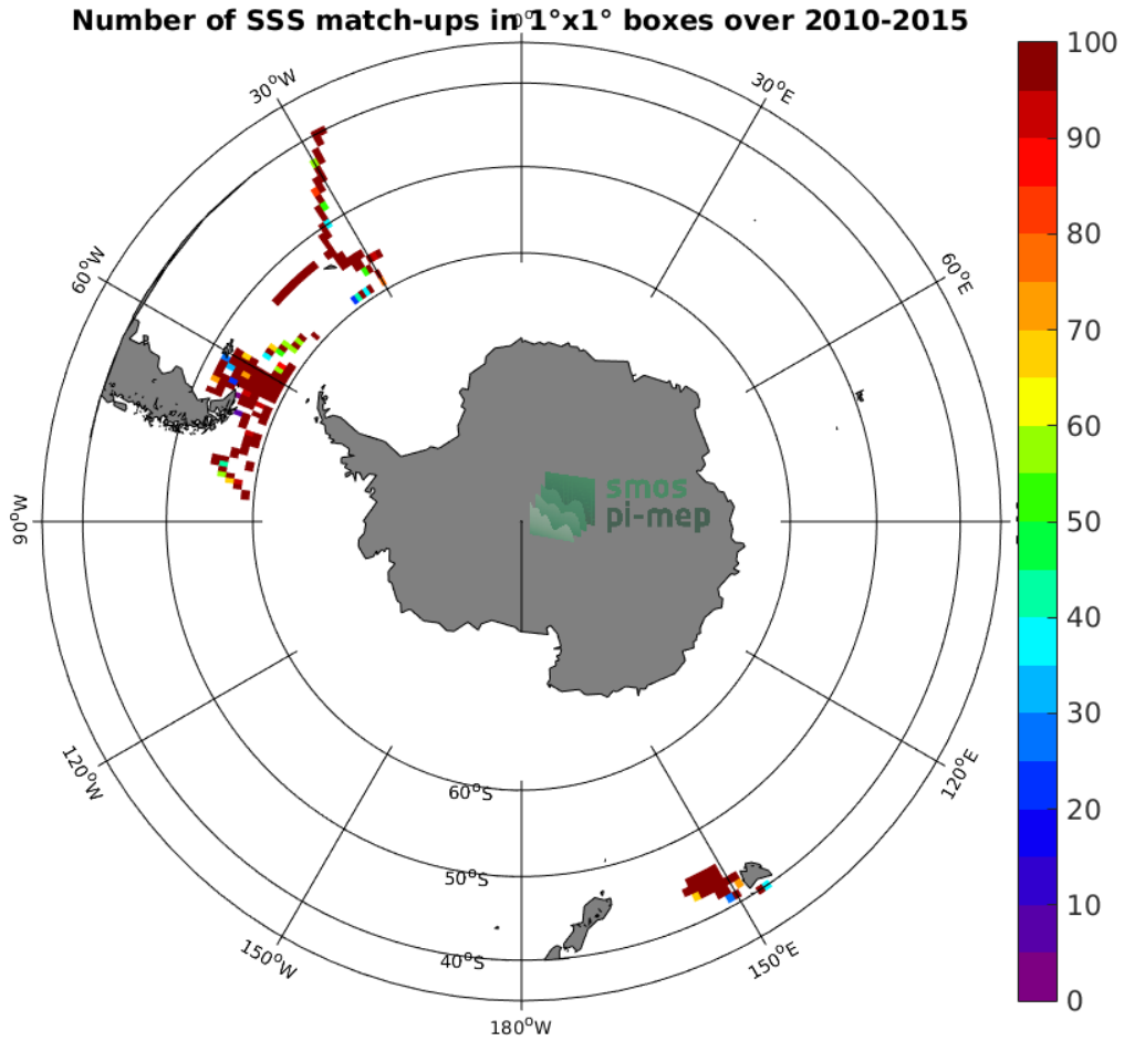
Figure 4: Number of SSS match-ups between TSG (SAMOS) SSS and the CCI SSS L4 Merged-OI v2.31 - 7-day running (ESA) SSS product for the Roaring Forties and Furious Fifties Pi-MEP region over 1°x1° boxes and for the full satellite product period.
