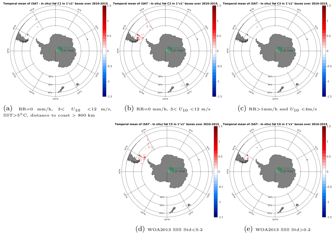
Figure 12: Temporal mean gridded over spatial boxes of size 1^{\circ}\times 1^{\circ} of \Delta\text{SSS} (CCI L4 Merged-OI v2.31 - 7-day running (ESA) - TSG (SAMOS)) for 5 different subdatasets corresponding to:RR=0 mm/h, 3 < U_{10} < 12 m/s, SST >5^{\circ}\text{C} , distance to coast > 800 km (a), RR=0 mm/h, 3 < U_{10} < 12 m/s (b), RR >1 mm/h and U_{10} < 4 m/s (c), WOA2013 SSS Std <0.2 (d), WOA2013 SSS Std >0.2 (e).
