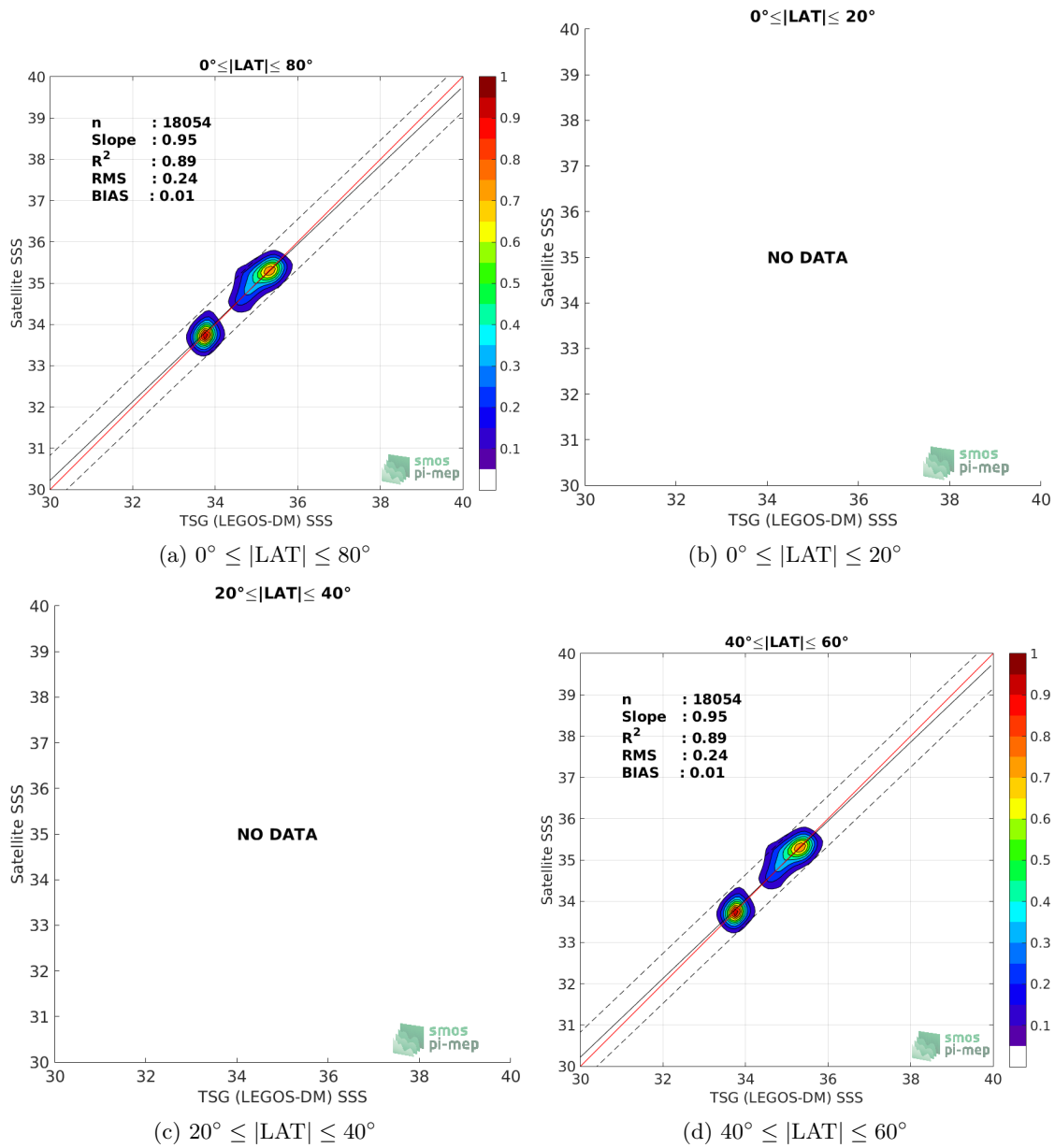
Figure 9: Contour maps of the concentration of CCI L4 Merged-OI v2.31 - 7-day running (ESA) SSS (y-axis) versus TSG (LEGOS-DM) SSS (x-axis) at match-up pairs for different latitude bands. For each plot, the red line shows x=y . The black thin and dashed lines indicate a linear fit through the data cloud and the \pm 95\% confidence levels, respectively. The number match-up pairs n , the slope and R^2 coefficient of the linear fit, the root mean square (RMS) and the mean bias between satellite and in situ data are indicated for each latitude band in each plots.
