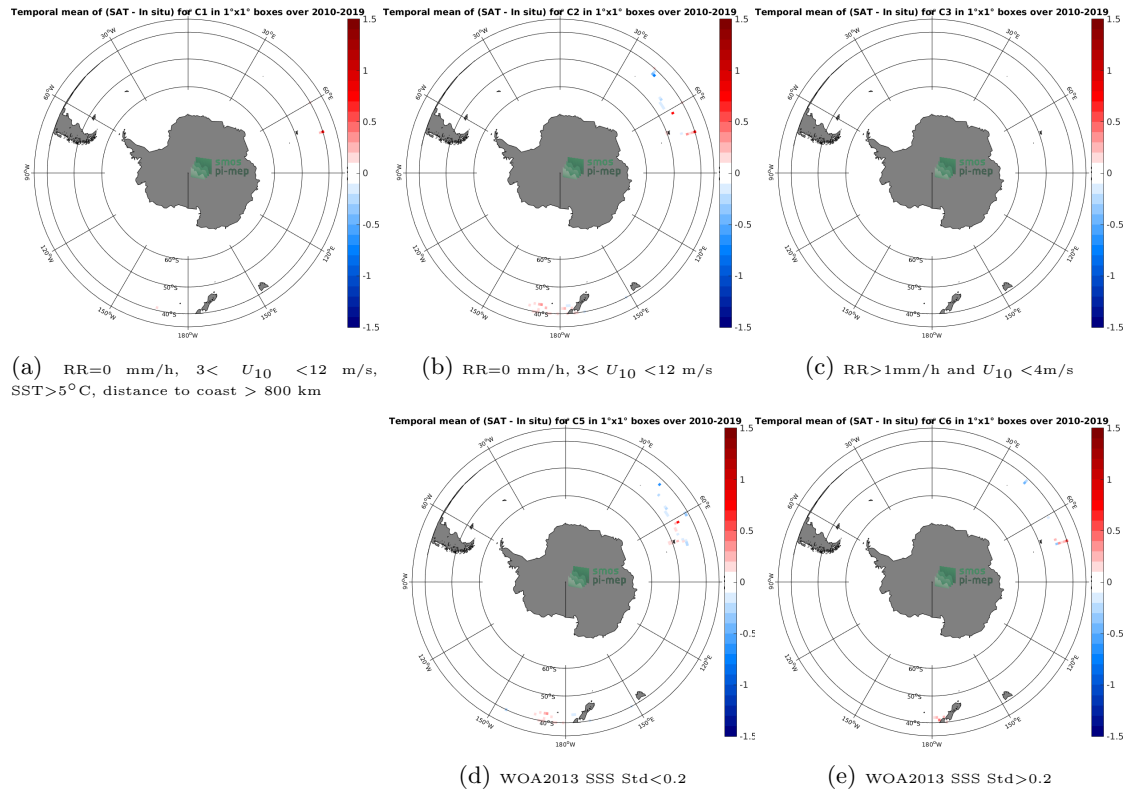
Figure 12: Temporal mean gridded over spatial boxes of size 1^{\circ}\times 1^{\circ} of \Delta\text{SSS} (CCI L4 Merged-OI v2.31 - 7-day running (ESA) - TSG (LEGOS-DM)) for 5 different subdatasets corresponding to: RR=0 mm/h, 3 < U_{10} < 12 m/s, SST >5^{\circ}\text{C} , distance to coast > 800 km (a), RR=0 mm/h, 3 < U_{10} < 12 m/s (b), RR >1 mm/h and U_{10} < 4 m/s (c), WOA2013 SSS Std <0.2 (d), WOA2013 SSS Std >0.2 (e).
