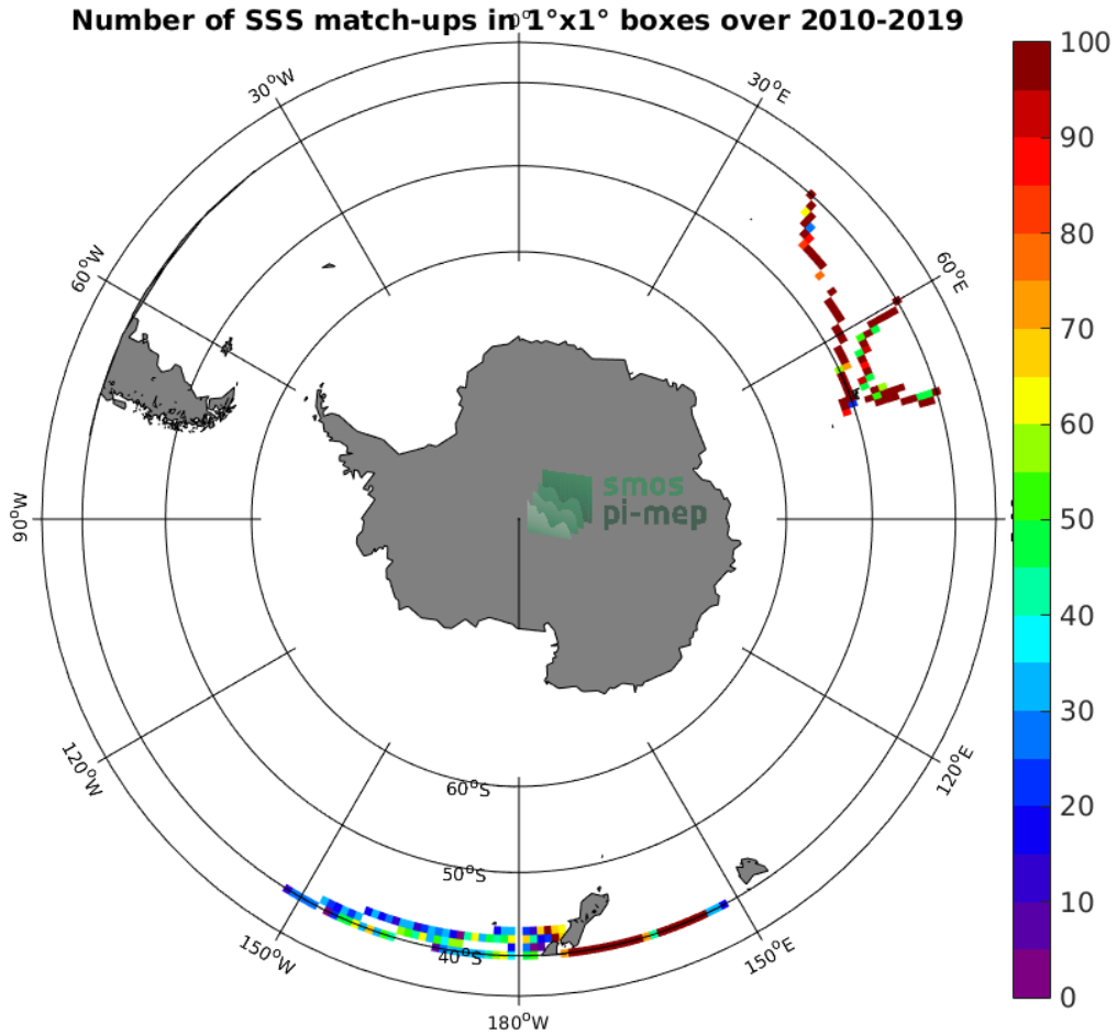
Figure 4: Number of SSS match-ups between TSG (LEGOS-DM) SSS and the CCI L4 Merged-OI v2.31 - 7-day running (ESA) SSS product for the Roaring Forties and Furious Fifties Pi-MEP region over 1°x1° boxes and for the full satellite product period.
