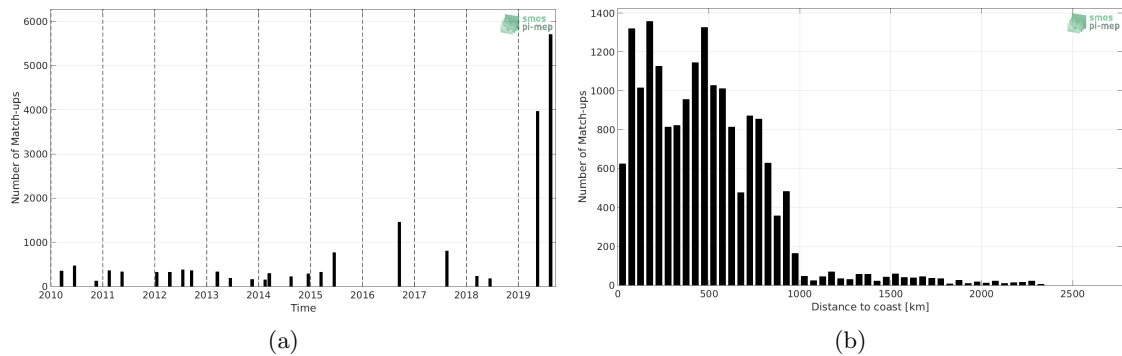
Figure 1: Number of match-ups between TSG (LEGOS-DM) and CCI L4 Merged-OI v2.31 - 7-day running (ESA) SSS as a function of time (a) and as function of the distance to coast (b) over the Roaring Forties and Furious Fifties Pi-MEP region and for the full satellite product period.
