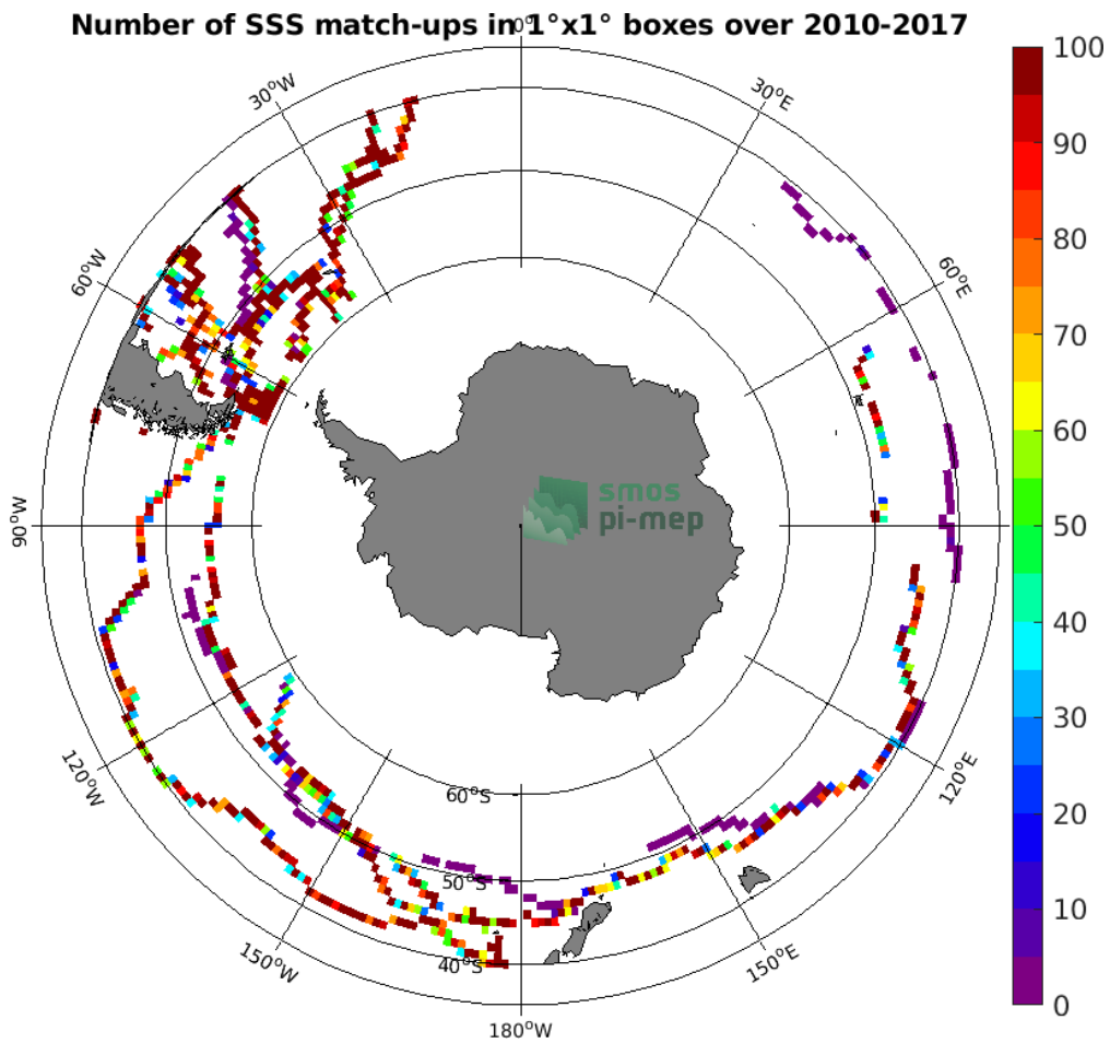
Figure 4: Number of SSS match-ups between TSG (GOSUD-Sailing-ship) SSS and the CCI SSS L4 Merged-OI v2.31 - 7-day running (ESA) SSS product for the Roaring Forties and Furious Fifties Pi-MEP region over 1^\circ \times 1^\circ boxes and for the full satellite product period.
