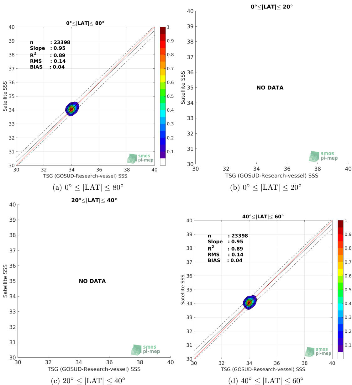
Figure 9: Contour maps of the concentration of CCI SSS L4 Merged-OI v2.31 - 7-day running (ESA) SSS ( y -axis) versus TSG (GOSUD-Research-vessel) SSS ( x -axis) at match-up pairs for different latitude bands. For each plot, the red line shows x=y . The black thin and dashed lines indicate a linear fit through the data cloud and the \pm 95\% confidence levels, respectively. The number match-up pairs n , the slope and R^2 coefficient of the linear fit, the root mean square (RMS) and the mean bias between satellite and in situ data are indicated for each latitude band in each plots.
