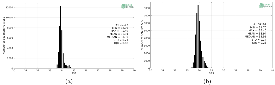
Figure 2: Histograms of SSS from Sea mammals (a) and CCI SSS L4 Merged-OI v2.31 - 7-day running (ESA) (b) considering all match-up pairs per bins of 0.1 over the Roaring Forties and Furious Fifties Pi-MEP region and for the full satellite product period.
