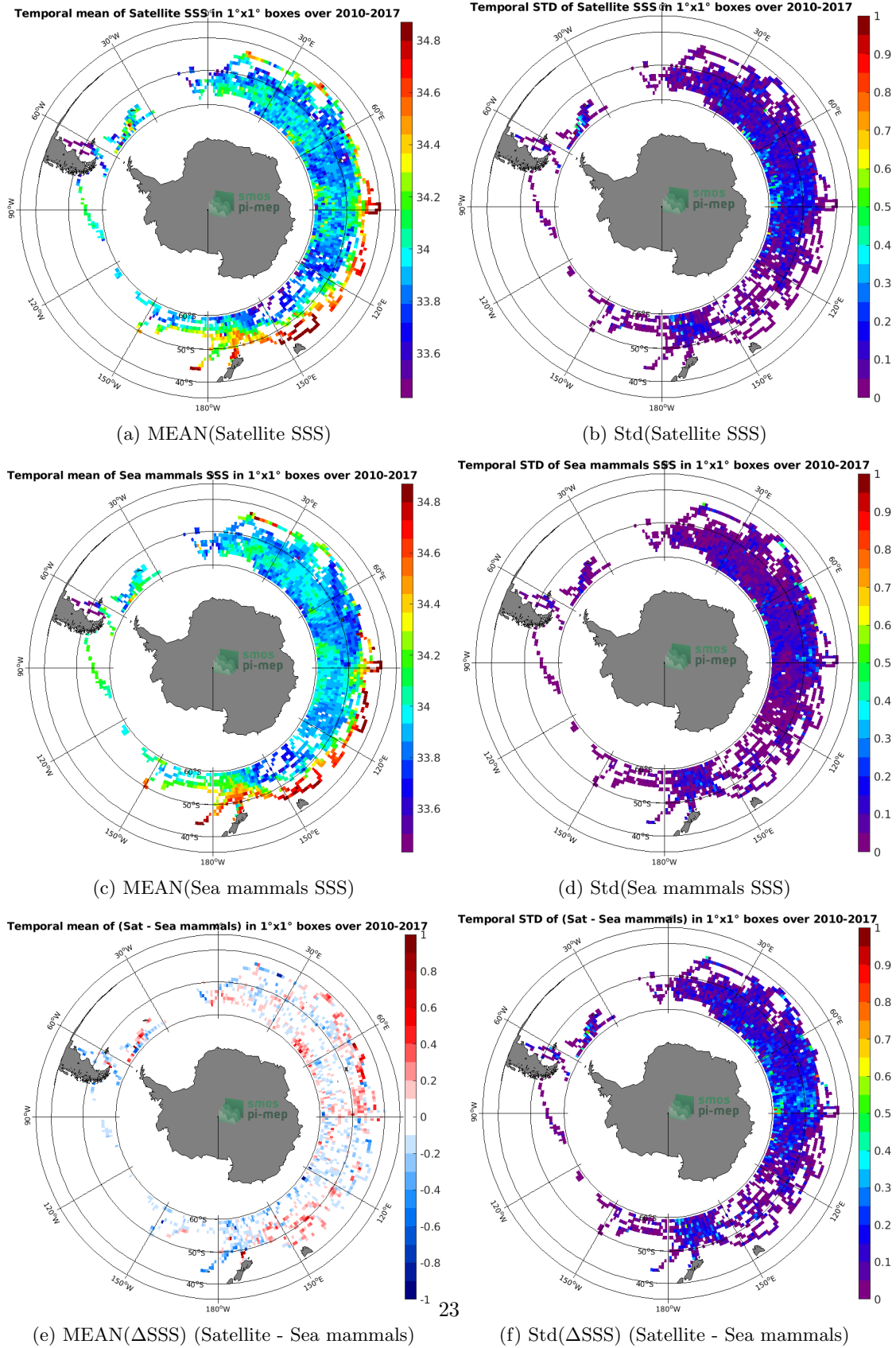
Figure 6: Temporal mean (left) and Std (right) of SSS from CCI SSS L4 Merged-OI v2.31 - 7-day running (ESA) (top), Sea mammals (middle), and of \Delta SSS (Satellite - Sea mammals). Only match-up pairs are used to generate these maps.
