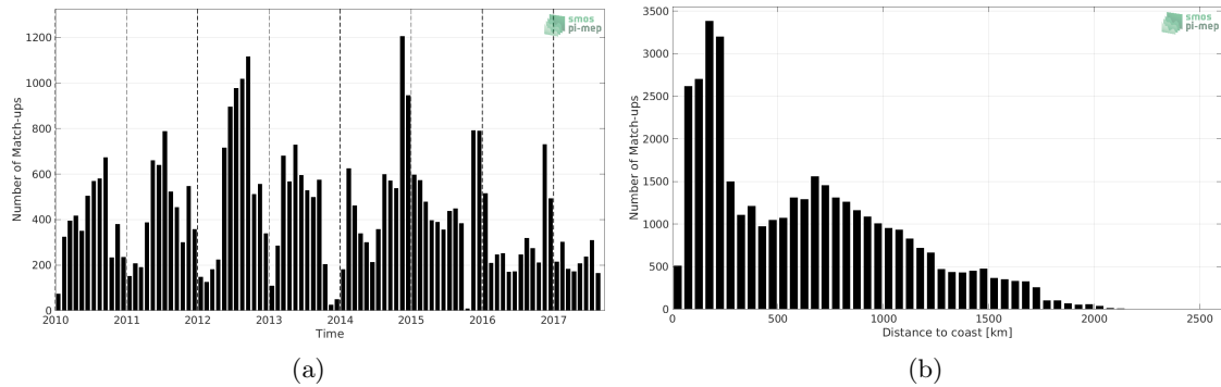
Figure 1: Number of match-ups between Sea mammals and CCI SSS L4 Merged-OI v2.31 - 7-day running (ESA) SSS as a function of time (a) and as function of the distance to coast (b) over the Roaring Forties and Furious Fifties Pi-MEP region and for the full satellite product period.
