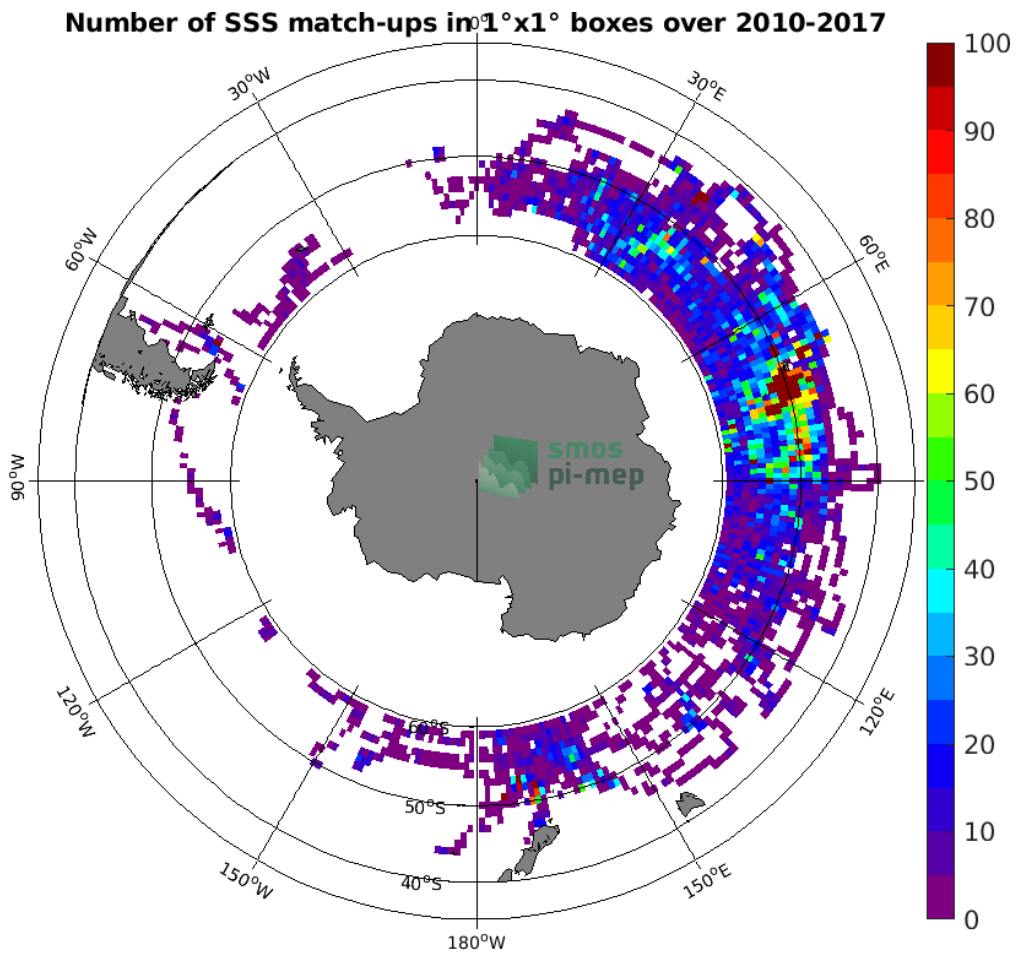
Figure 4: Number of SSS match-ups between Sea mammals SSS and the CCI SSS L4 Merged-OI v2.31 - 7-day running (ESA) SSS product for the Roaring Forties and Furious Fifties Pi-MEP region over 1^\circ \times 1^\circ boxes and for the full satellite product period.
