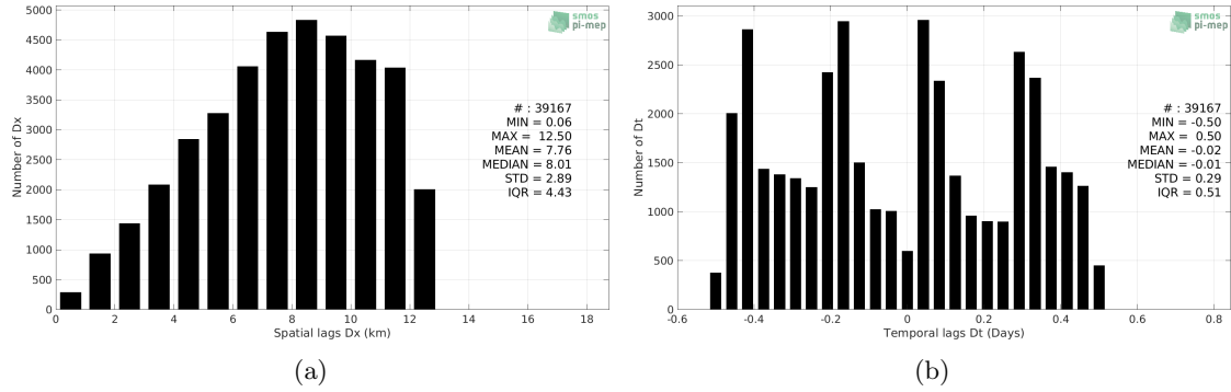
Figure 5: Histograms of the spatial (a) and temporal (b) lags between the location/time of the Sea mammals measurement and the date of the corresponding CCI SSS L4 Merged-OI v2.31 - 7-day running (ESA) SSS pixel.
