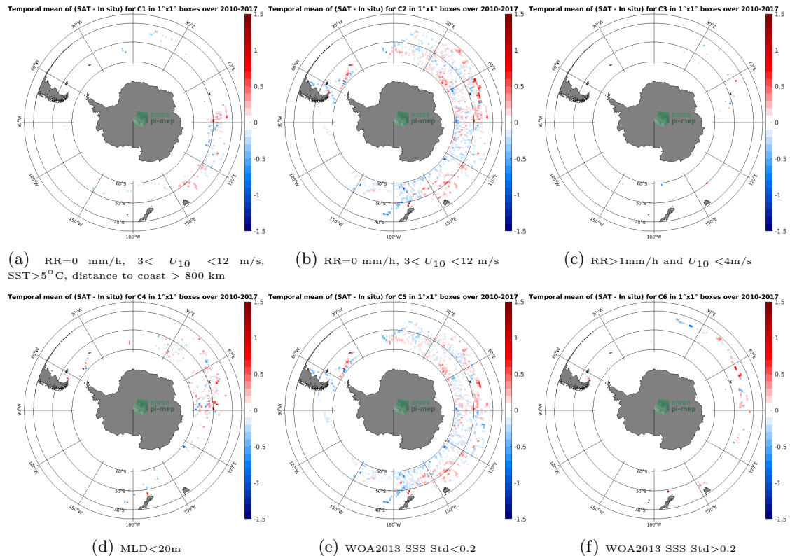
Figure 12: Temporal mean gridded over spatial boxes of size 1^{\circ}\times 1^{\circ} of \Delta\text{SSS} (CCI SSS L4 Merged-OI v2.31 - 7-day running (ESA) - Sea mammals) for 6 different subdatasets corresponding to: RR=0 mm/h, 3 < U_{10} < 12 m/s, SST > 5^{\circ}\text{C} , distance to coast > 800 km (a), RR=0 mm/h, 3 < U_{10} < 12 m/s (b), RR > 1\text{mm/h} and U_{10} < 4\text{m/s} (c), MLD < 20\text{m} (d), WOA2013 SSS Std < 0.2 (e), WOA2013 SSS Std > 0.2 (f).
