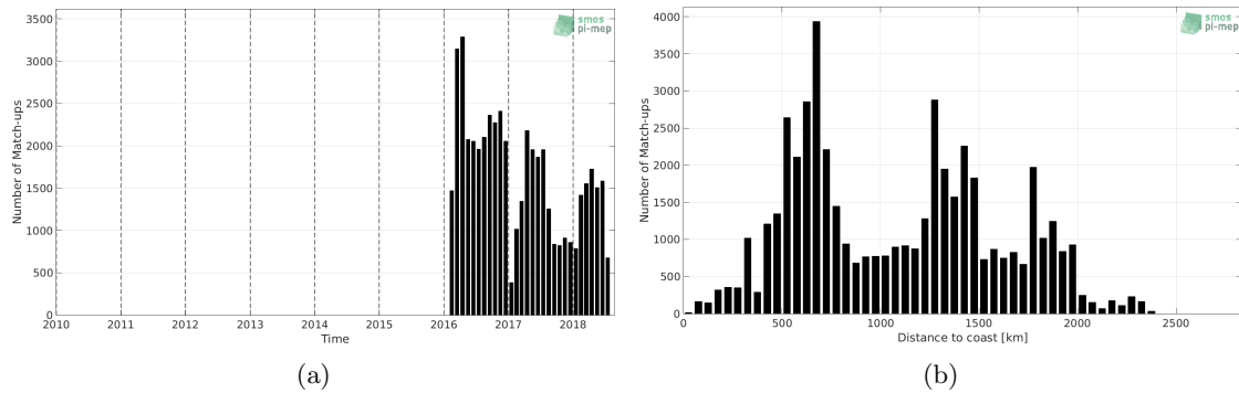
Figure 1: Number of match-ups between Surface drifters and CCI SSS L4 Merged-OI v2.31 - 7-day running (ESA) SSS as a function of time (a) and as function of the distance to coast (b) over the Roaring Forties and Furious Fifties Pi-MEP region and for the full satellite product period.
