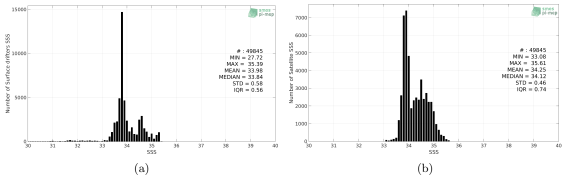
Figure 2: Histograms of SSS from Surface drifters (a) and CCI SSS L4 Merged-OI v2.31 - 7-day running (ESA) (b) considering all match-up pairs per bins of 0.1 over the Roaring Forties and Furious Fifties Pi-MEP region and for the full satellite product period.
