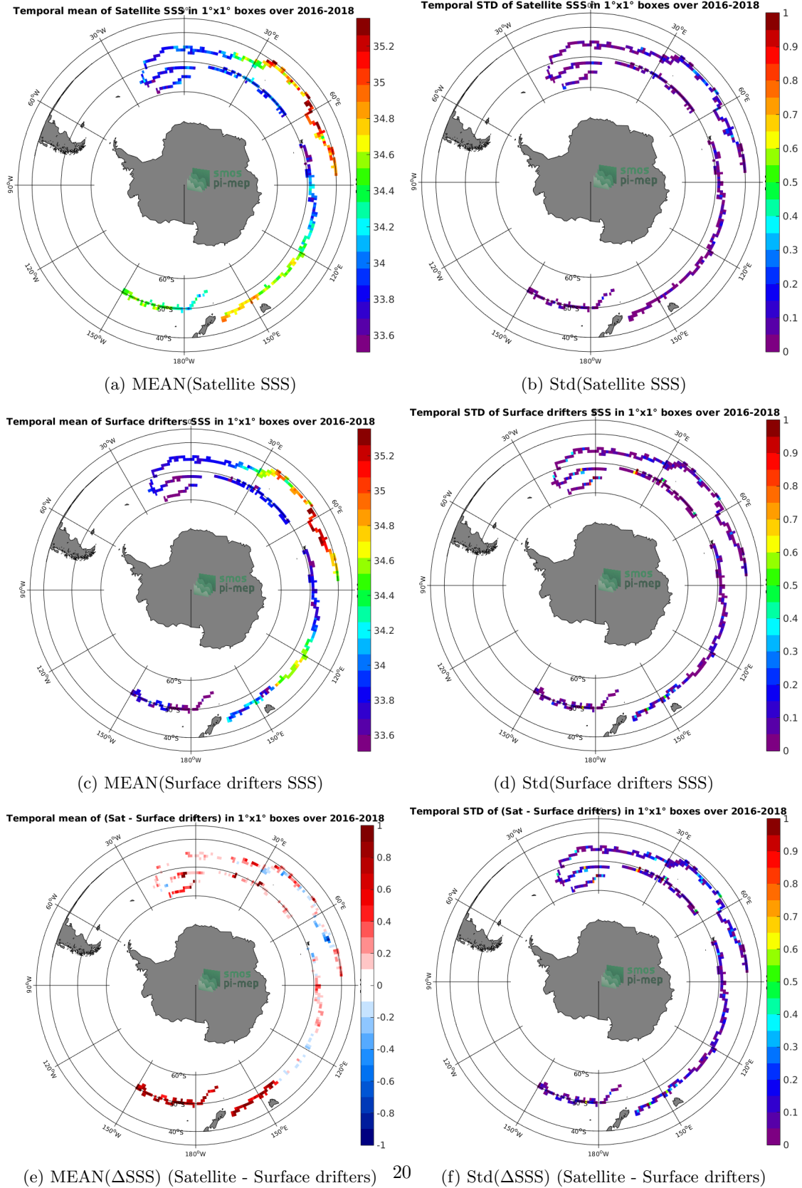
Figure 5: Temporal mean (left) and Std (right) of SSS from CCI SSS L4 Merged-OI v2.31 - 7-day running (ESA) (top), Surface drifters (middle), and of \Delta SSS (Satellite - Surface drifters). Only match-up pairs are used to generate these maps.
