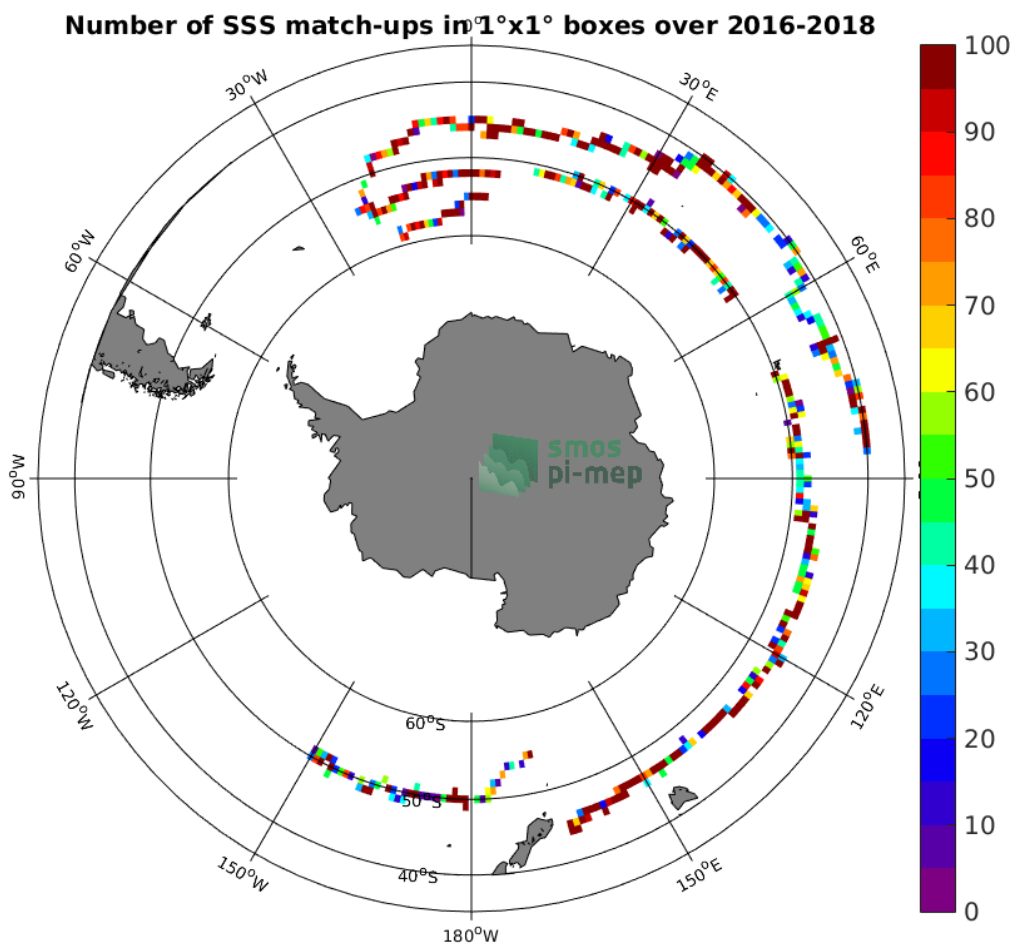
Figure 3: Number of SSS match-ups between Surface drifters SSS and the CCI SSS L4 Merged-OI v2.31 - 7-day running (ESA) SSS product for the Roaring Forties and Furious Fifties Pi-MEP region over 1^\circ \times 1^\circ boxes and for the full satellite product period.
