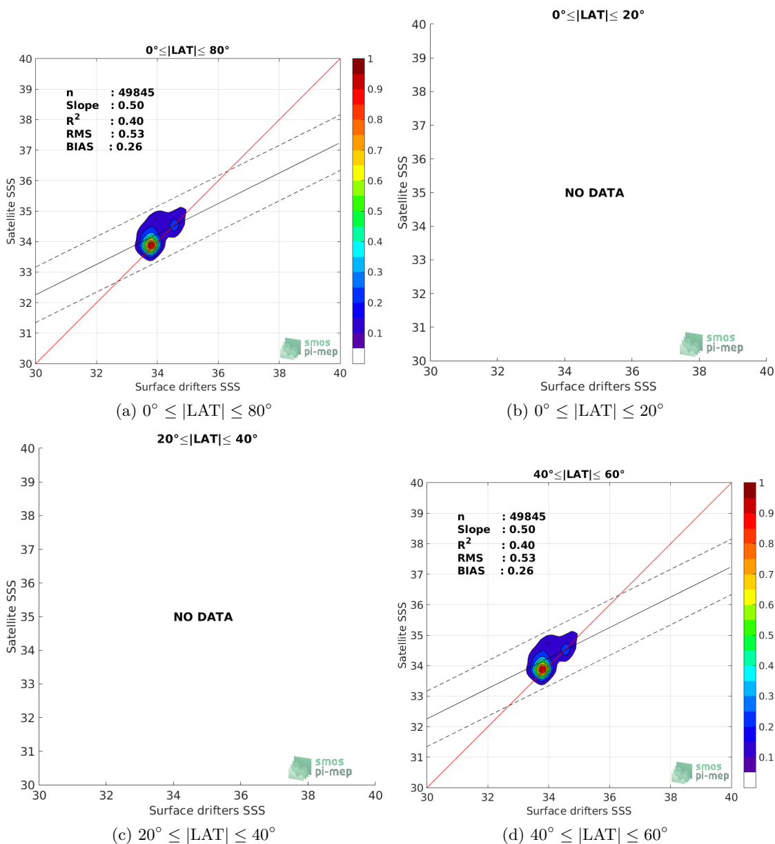
Figure 8: Contour maps of the concentration of CCI SSS L4 Merged-OI v2.31 - 7-day running (ESA) SSS (y-axis) versus Surface drifters SSS (x-axis) at match-up pairs for different latitude bands. For each plot, the red line shows x=y . The black thin and dashed lines indicate a linear fit through the data cloud and the \pm 95\% confidence levels, respectively. The number match-up pairs n , the slope and R^2 coefficient of the linear fit, the root mean square (RMS) and the mean bias between satellite and in situ data are indicated for each latitude band in each plots.
