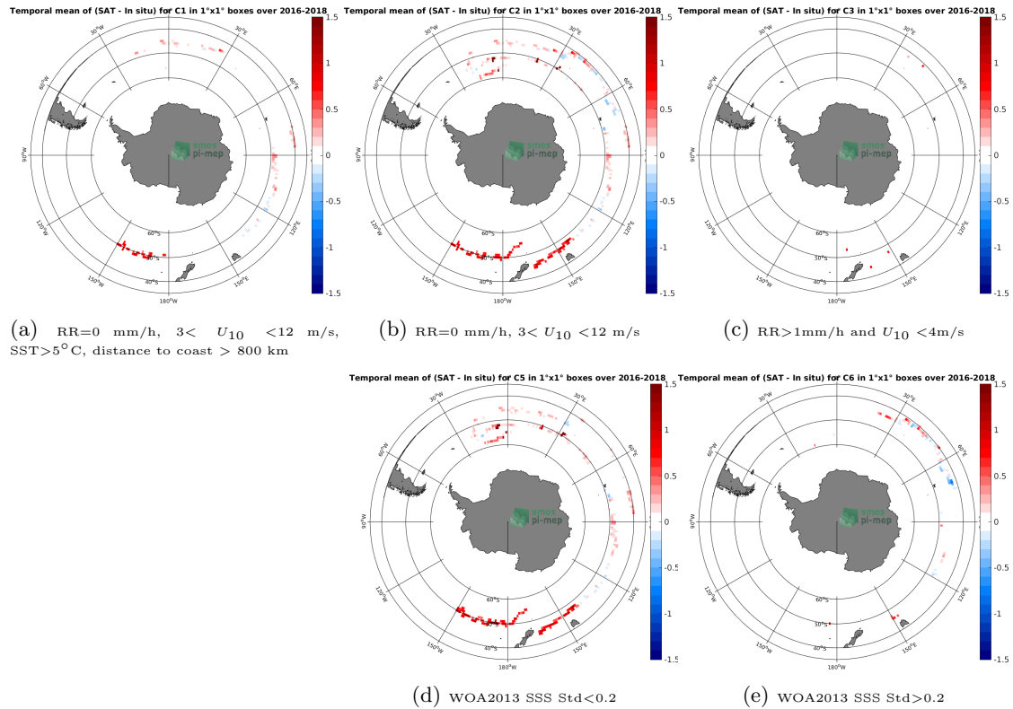
Figure 11: Temporal mean gridded over spatial boxes of size 1^{\circ}\times 1^{\circ} of \Delta\text{SSS} (CCI SSS L4 Merged-OI v2.31 - 7-day running (ESA) - Surface drifters) for 5 different subdatasets corresponding to:RR=0 mm/h, 3 < U_{10} < 12 m/s, SST >5^{\circ}\text{C} , distance to coast > 800 km (a), RR=0 mm/h, 3 < U_{10} < 12 m/s (b), RR >1 mm/h and U_{10} < 4 m/s (c), WOA2013 SSS Std <0.2 (d), WOA2013 SSS Std >0.2 (e).
