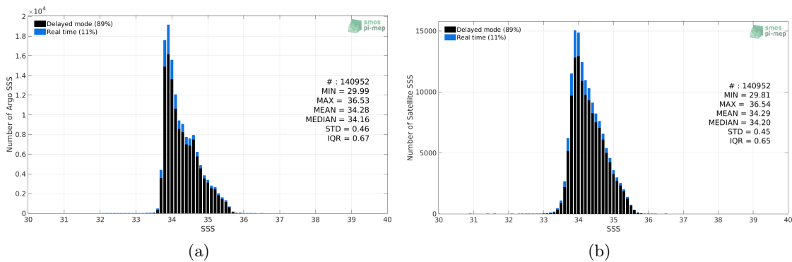
Figure 2: Histograms of SSS from Argo (a) and CCI L4 Merged-OI v2.31 - 7-day running (ESA) (b) considering all match-up pairs per bins of 0.1 over the Roaring Forties and Furious Fifties Pi-MEP region and for the full satellite product period.
