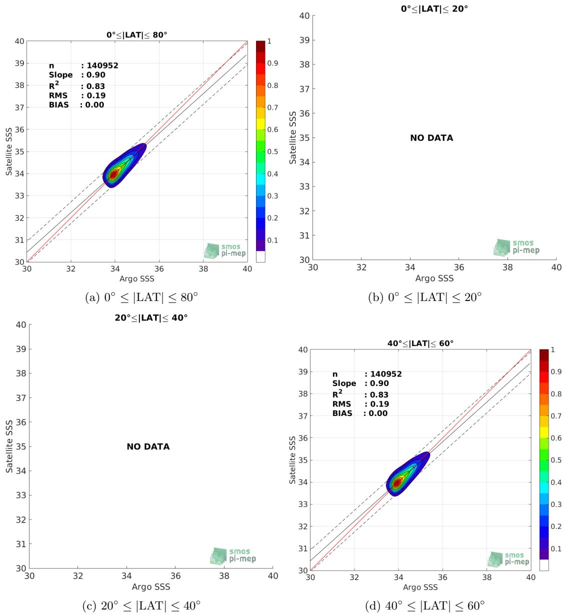
Figure 9: Contour maps of the concentration of CCI L4 Merged-OI v2.31 - 7-day running (ESA) SSS (y-axis) versus Argo SSS (x-axis) at match-up pairs for different latitude bands. For each plot, the red line shows x=y . The black thin and dashed lines indicate a linear fit through the data cloud and the \pm 95\% confidence levels, respectively. The number match-up pairs n , the slope and R^2 coefficient of the linear fit, the root mean square (RMS) and the mean bias between satellite and in situ data are indicated for each latitude band in each plots.
