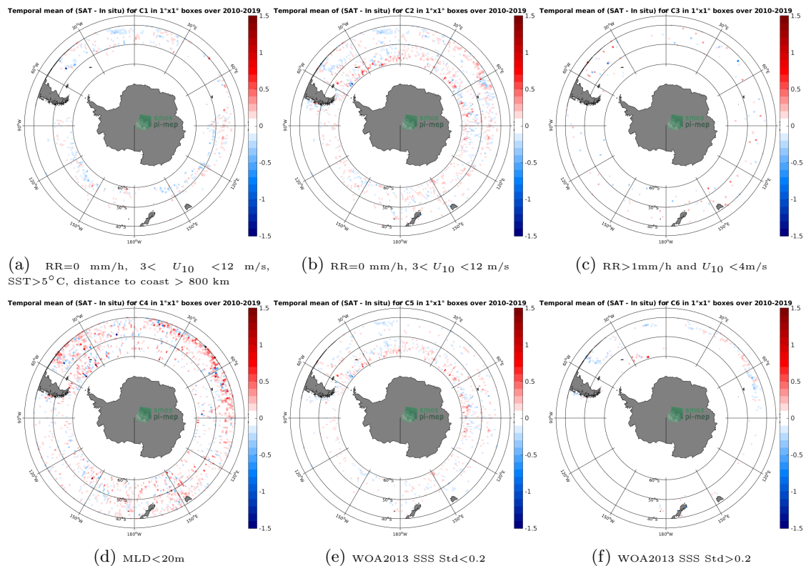
Figure 12: Temporal mean gridded over spatial boxes of size 1^{\circ}\times 1^{\circ} of \Delta\text{SSS} (CCI L4 Merged-OI v2.31 - 7-day running (ESA) - Argo) for 6 different subdatasets corresponding to:RR=0 mm/h, 3 < U_{10} < 12 m/s, SST > 5^{\circ}\text{C} , distance to coast > 800 km (a), RR=0 mm/h, 3 < U_{10} < 12 m/s (b), RR > 1 mm/h and U_{10} < 4 m/s (c),MLD < 20\text{m} (d),WOA2013 SSS Std < 0.2 (e),WOA2013 SSS Std > 0.2 (f).
