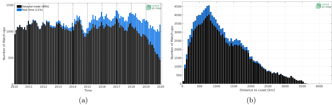
Figure 1: Number of match-ups between Argo and CCI L4 Merged-OI v2.31 - 7-day running (ESA) SSS as a function of time (a) and as function of the distance to coast (b) over the Roaring Forties and Furious Fifties Pi-MEP region and for the full satellite product period.
