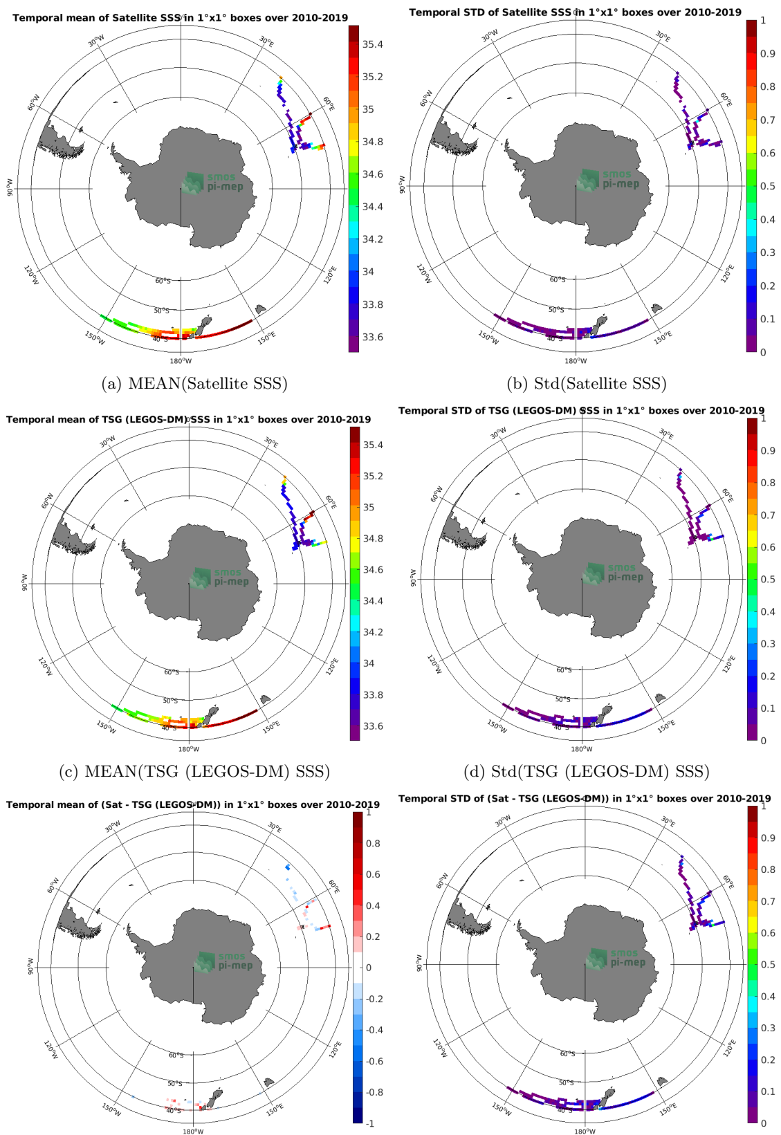
Figure 6: Temporal mean (left) and Std (right) of SSS from CCI SSS L4 Merged-OI v2.31 - 30-day running (ESA) (top), TSG (LEGOS-DM) (middle), and of \Delta SSS (Satellite - TSG (LEGOS-DM)). Only match-up pairs are used to generate these maps.
