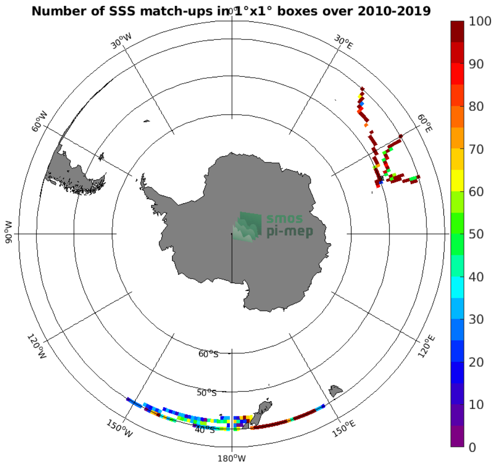
Figure 4: Number of SSS match-ups between TSG (LEGOS-DM) SSS and the CCI SSS L4 Merged-OI v2.31 - 30-day running (ESA) SSS product for the Roaring Forties and Furious Fifties Pi-MEP region over 1^\circ \times 1^\circ boxes and for the full satellite product period.
