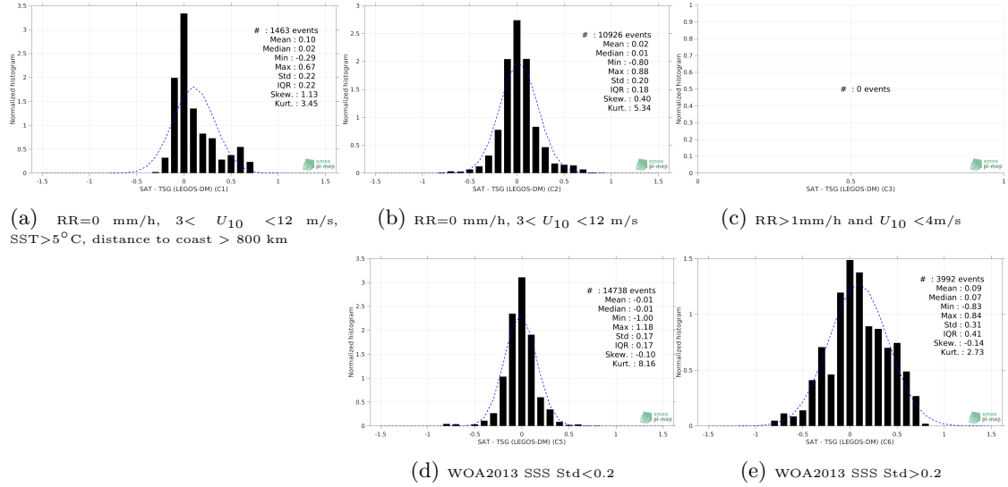
Figure 13: Normalized histogram of \Delta\text{SSS} (CCI SSS L4 Merged-OI v2.31 - 30-day running (ESA) - TSG (LEGOS-DM)) for 5 different subdatasets corresponding to: RR=0 mm/h, 3 < U_{10} < 12 m/s, SST >5^{\circ}\text{C} , distance to coast > 800 km (a), RR=0 mm/h, 3 < U_{10} < 12 m/s (b), RR >1 mm/h and U_{10} < 4 m/s (c), WOA2013 SSS Std <0.2 (d), WOA2013 SSS Std >0.2 (e).
