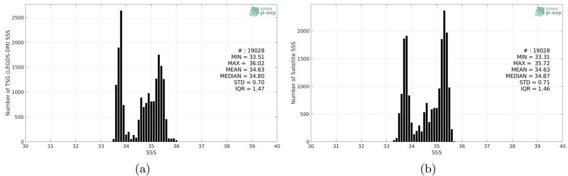
Figure 2: Histograms of SSS from TSG (LEGOS-DM) (a) and CCI SSS L4 Merged-OI v2.31 - 30-day running (ESA) (b) considering all match-up pairs per bins of 0.1 over the Roaring Forties and Furious Fifties Pi-MEP region and for the full satellite product period.
