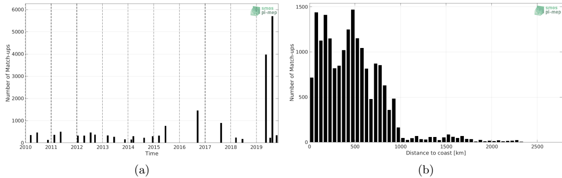
Figure 1: Number of match-ups between TSG (LEGOS-DM) and CCI SSS L4 Merged-OI v2.31 - 30-day running (ESA) SSS as a function of time (a) and as function of the distance to coast (b) over the Roaring Forties and Furious Fifties Pi-MEP region and for the full satellite product period.
