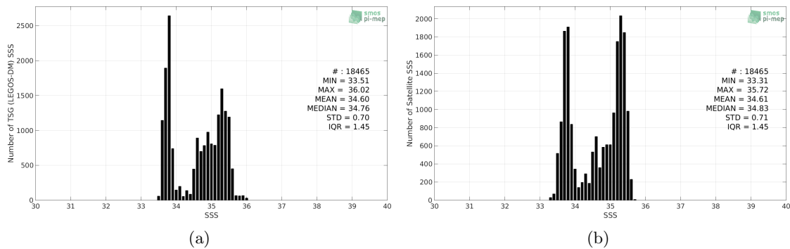
Figure 2: Histograms of SSS from TSG (LEGOS-DM) (a) and CCI L4 Merged-OI v2.31 - 30-day running (ESA) (b) considering all match-up pairs per bins of 0.1 over the Roaring Forties and Furious Fifties Pi-MEP region and for the full satellite product period.
