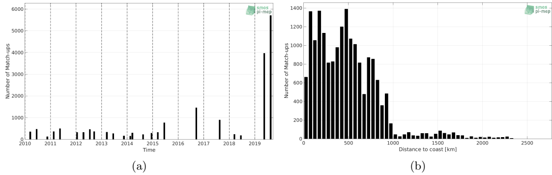
Figure 1: Number of match-ups between TSG (LEGOS-DM) and CCI L4 Merged-OI v2.31 - 30-day running (ESA) SSS as a function of time (a) and as function of the distance to coast (b) over the Roaring Forties and Furious Fifties Pi-MEP region and for the full satellite product period.
