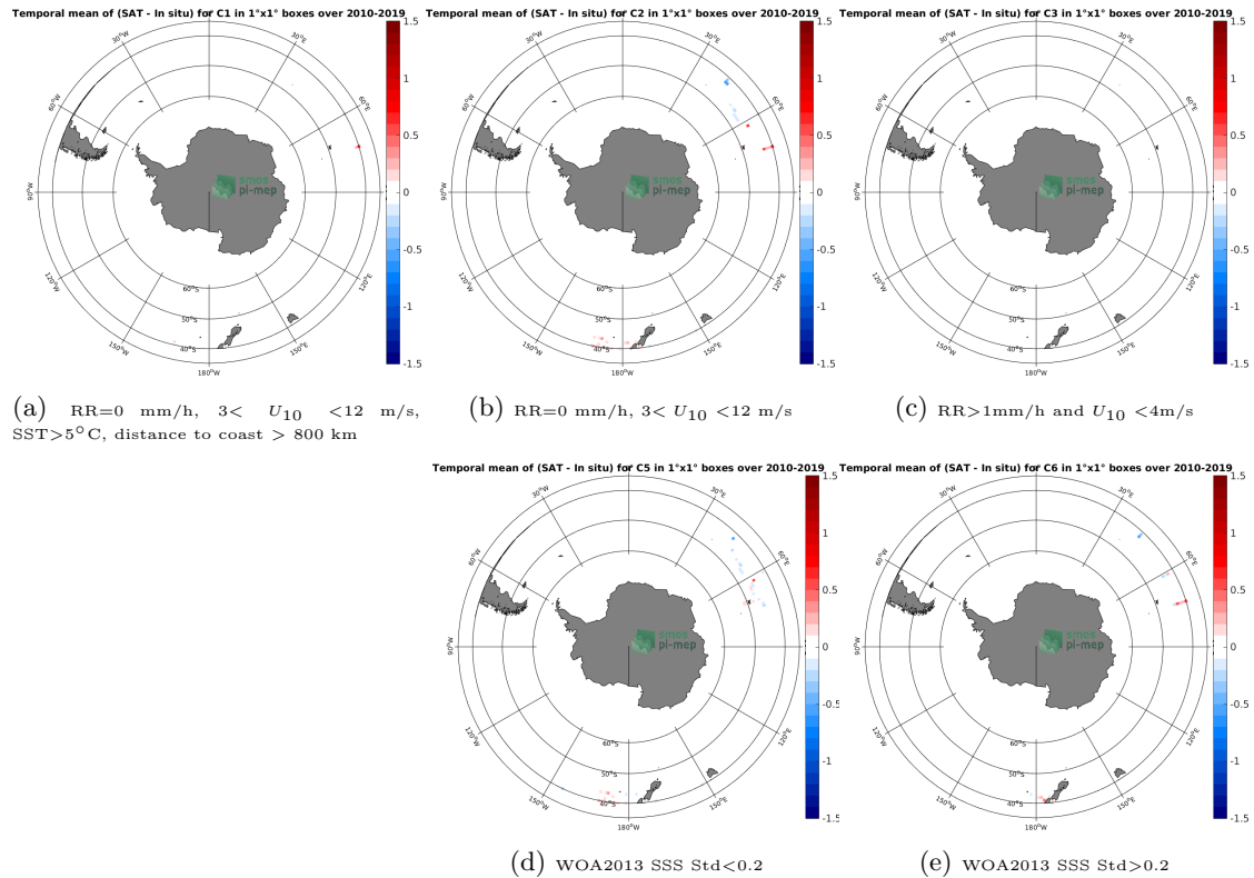
Figure 12: Temporal mean gridded over spatial boxes of size 1^{\circ}\times 1^{\circ} of \Delta\text{SSS} (CCI L4 Merged-OI v2.31 - 30-day running (ESA) - TSG (LEGOS-DM)) for 5 different subdatasets corresponding to: RR=0 mm/h, 3 < U_{10} < 12 m/s, SST >5^{\circ}\text{C} , distance to coast > 800 km (a), RR=0 mm/h, 3 < U_{10} < 12 m/s (b), RR >1 mm/h and U_{10} < 4 m/s (c), WOA2013 SSS Std <0.2 (d), WOA2013 SSS Std >0.2 (e).
