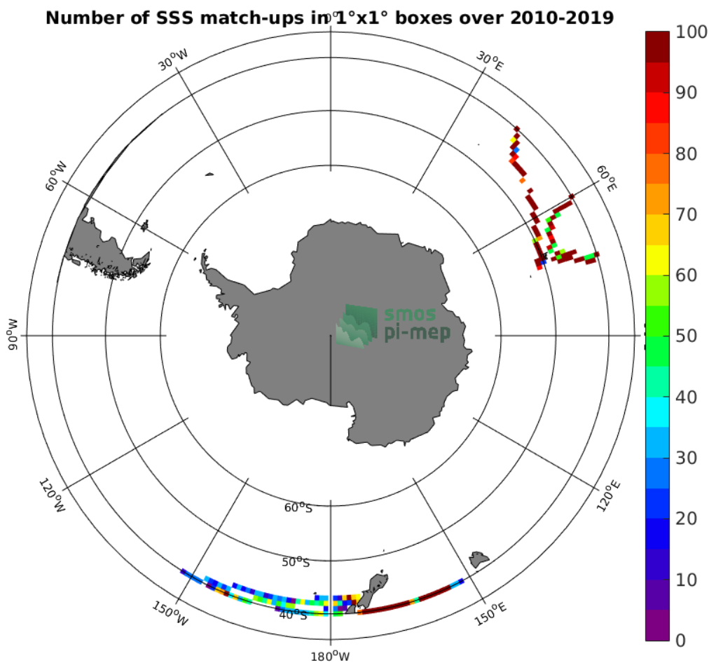
Figure 4: Number of SSS match-ups between TSG (LEGOS-DM) SSS and the CCI L4 Merged-OI v2.31 - 30-day running (ESA) SSS product for the Roaring Forties and Furious Fifties Pi-MEP region over 1°x1° boxes and for the full satellite product period.
