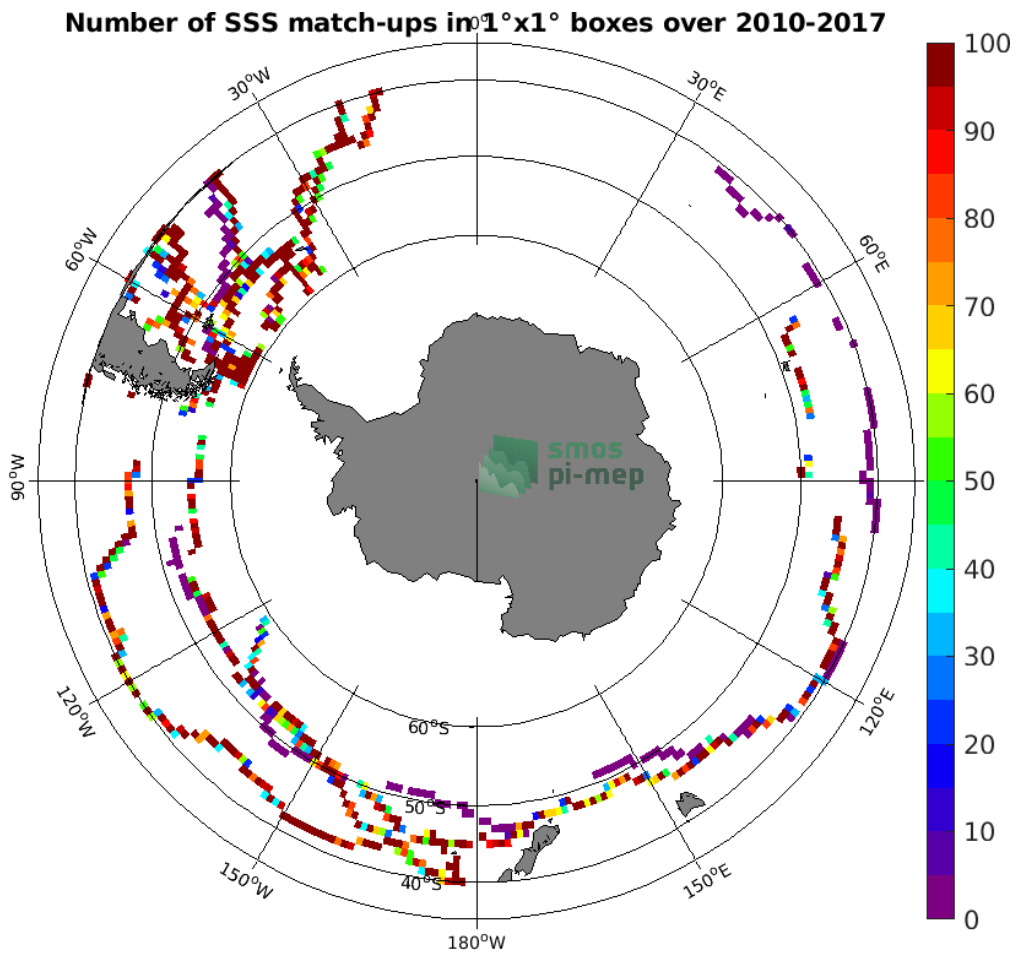
Figure 4: Number of SSS match-ups between TSG (GOSUD-Sailing-ship) SSS and the CCI SSS L4 Merged-OI v2.31 - 30-day running (ESA) SSS product for the Roaring Forties and Furious Fifties Pi-MEP region over 1^\circ \times 1^\circ boxes and for the full satellite product period.
