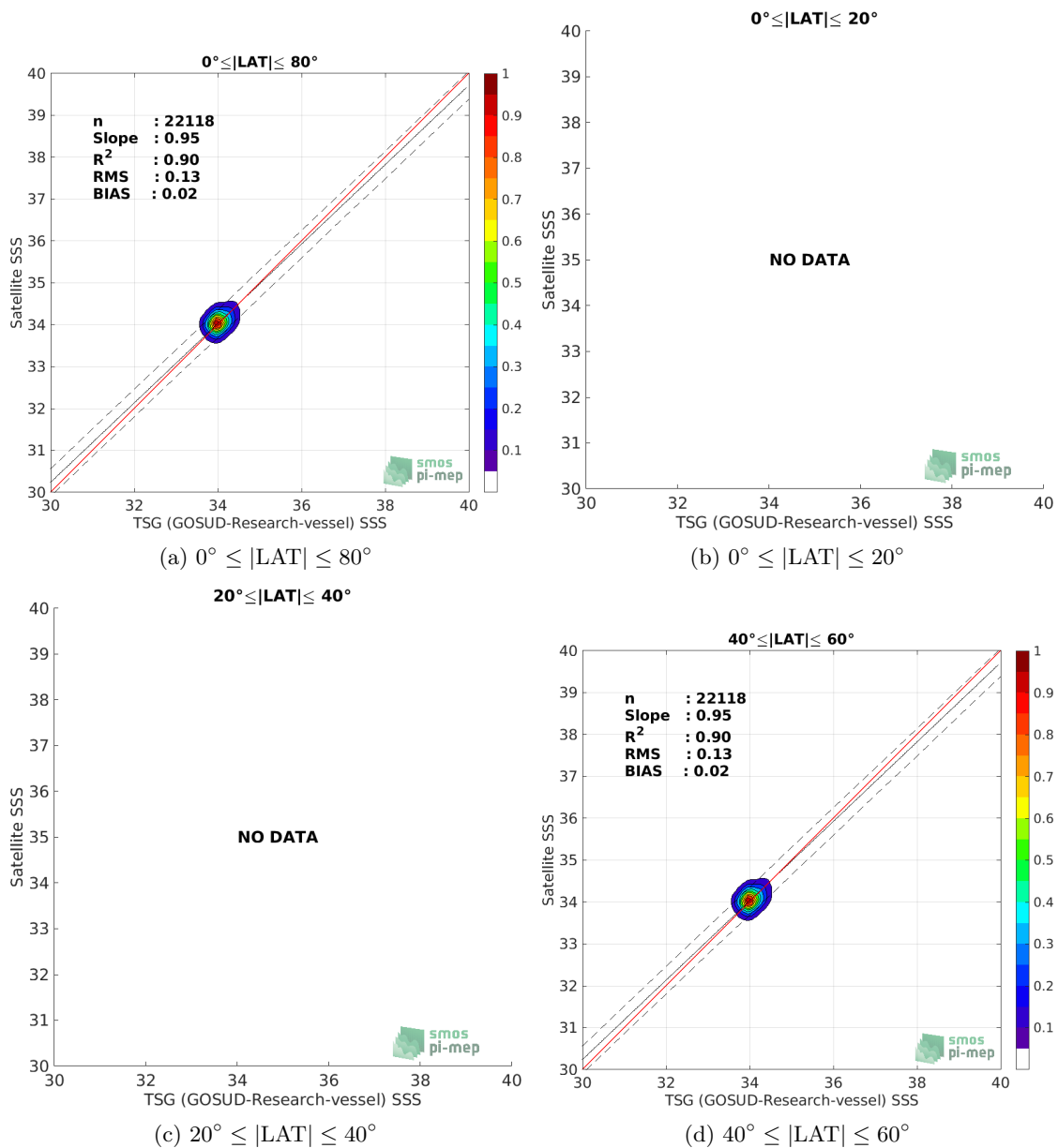
Figure 9: Contour maps of the concentration of CCI SSS L4 Merged-OI v2.31 - 30-day running (ESA) SSS (y-axis) versus TSG (GOSUD-Research-vessel) SSS (x-axis) at match-up pairs for different latitude bands. For each plot, the red line shows x=y . The black thin and dashed lines indicate a linear fit through the data cloud and the \pm 95\% confidence levels, respectively. The number match-up pairs n , the slope and R^2 coefficient of the linear fit, the root mean square (RMS) and the mean bias between satellite and in situ data are indicated for each latitude band in each plots.
