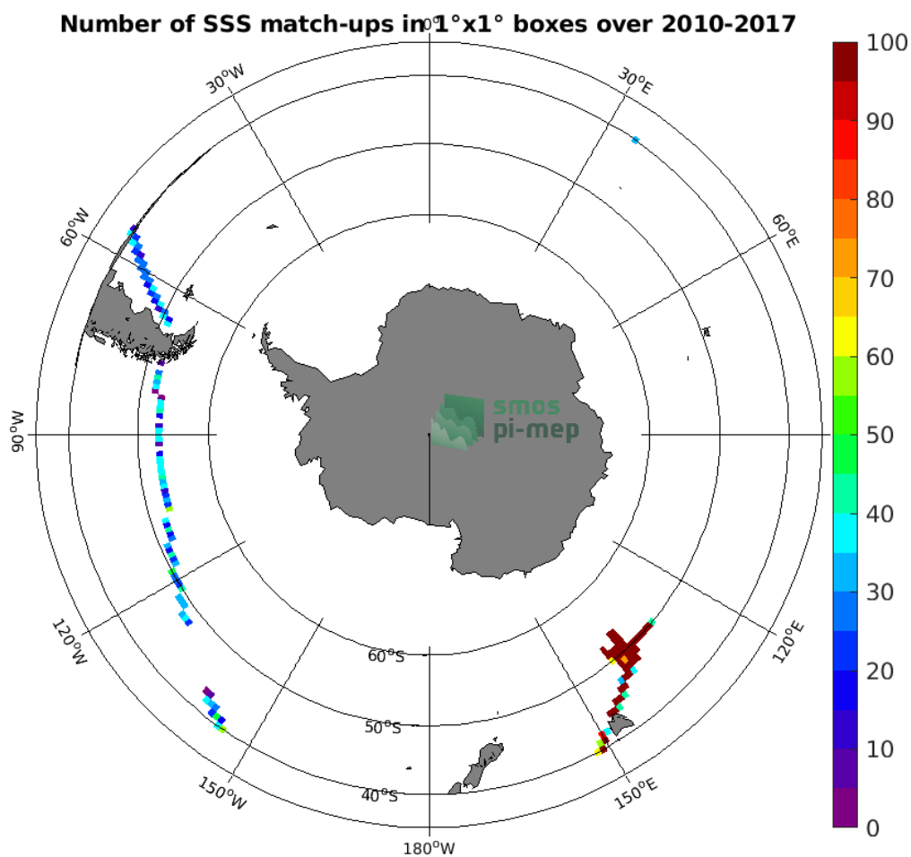
Figure 4: Number of SSS match-ups between TSG (GOSUD-Research-vessel) SSS and the CCI SSS L4 Merged-OI v2.31 - 30-day running (ESA) SSS product for the Roaring Forties and Furious Fifties Pi-MEP region over 1^\circ \times 1^\circ boxes and for the full satellite product period.
