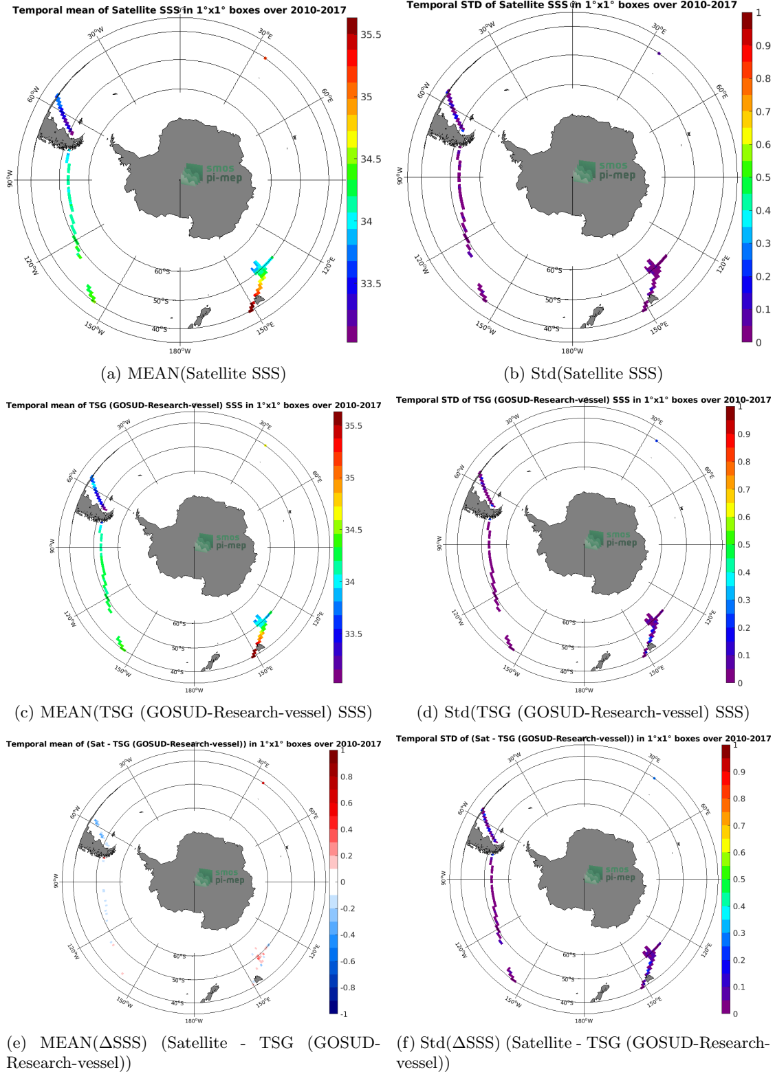
Figure 6: Temporal mean (left) and Std (right) of SSS from CCI SSS L4 Merged-OI v2.31 - 30-day running (ESA) (top), TSG (GOSUD-Research-vessel) (middle), and of \Delta SSS (Satellite - TSG (GOSUD-Research-vessel)). Only match- ed pairs are used to generate these maps.
