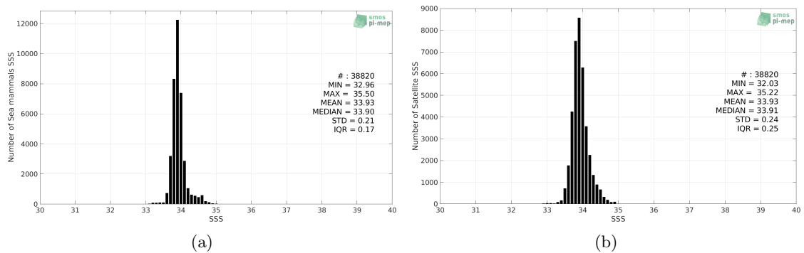
Figure 2: Histograms of SSS from Sea mammals (a) and CCI SSS L4 Merged-OI v2.31 - 30-day running (ESA) (b) considering all match-up pairs per bins of 0.1 over the Roaring Forties and Furious Fifties Pi-MEP region and for the full satellite product period.
