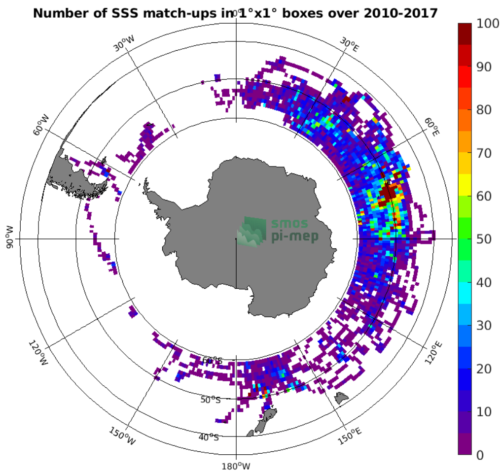
Figure 4: Number of SSS match-ups between Sea mammals SSS and the CCI SSS L4 Merged-OI v2.31 - 30-day running (ESA) SSS product for the Roaring Forties and Furious Fifties Pi-MEP region over 1^\circ \times 1^\circ boxes and for the full satellite product period.
