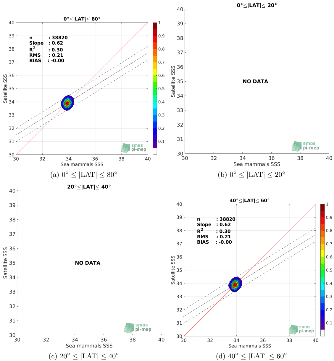
Figure 9: Contour maps of the concentration of CCI SSS L4 Merged-OI v2.31 - 30-day running (ESA) SSS (y-axis) versus Sea mammals SSS (x-axis) at match-up pairs for different latitude bands. For each plot, the red line shows x=y . The black thin and dashed lines indicate a linear fit through the data cloud and the \pm 95\% confidence levels, respectively. The number match-up pairs n , the slope and R^2 coefficient of the linear fit, the root mean square (RMS) and the mean bias between satellite and in situ data are indicated for each latitude band in each plots.
