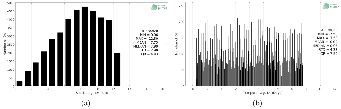
Figure 5: Histograms of the spatial (a) and temporal (b) lags between the location/time of the Sea mammals measurement and the date of the corresponding CCI SSS L4 Merged-OI v2.31 - 30-day running (ESA) SSS pixel.
