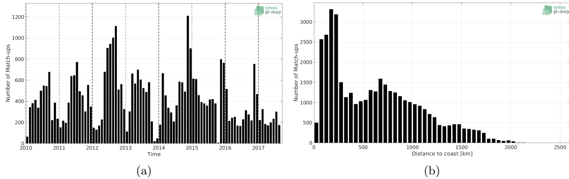
Figure 1: Number of match-ups between Sea mammals and CCI SSS L4 Merged-OI v2.31 - 30-day running (ESA) SSS as a function of time (a) and as function of the distance to coast (b) over the Roaring Forties and Furious Fifties Pi-MEP region and for the full satellite product period.
