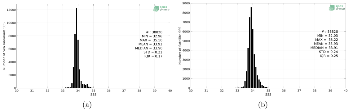
Figure 2: Histograms of SSS from Sea mammals (a) and CCI L4 Merged-OI v2.31 - 30-day running (ESA) (b) considering all match-up pairs per bins of 0.1 over the Roaring Forties and Furious Fifties Pi-MEP region and for the full satellite product period.
