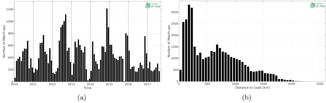
Figure 1: Number of match-ups between Sea mammals and CCI L4 Merged-OI v2.31 - 30-day running (ESA) SSS as a function of time (a) and as function of the distance to coast (b) over the Roaring Forties and Furious Fifties Pi-MEP region and for the full satellite product period.
