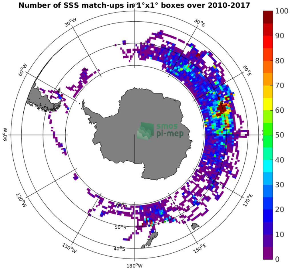
Figure 4: Number of SSS match-ups between Sea mammals SSS and the CCI L4 Merged-OI v2.31 - 30-day running (ESA) SSS product for the Roaring Forties and Furious Fifties Pi-MEP region over 1°x1° boxes and for the full satellite product period.
