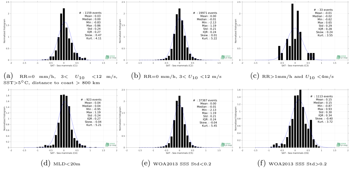
Figure 13: Normalized histogram of \Delta SSS (CCI L4 Merged-OI v2.31 - 30-day running (ESA) - Sea mammals) for 6 different subdatasets corresponding to: RR=0 mm/h, 3 < U_{10} < 12 m/s, SST > 5°C, distance to coast > 800 km (a), RR=0 mm/h, 3 < U_{10} < 12 m/s (b), RR > 1mm/h and U_{10} < 4 m/s (c), MLD < 20m (d), WOA2013 SSS Std < 0.2 (e), WOA2013 SSS Std > 0.2 (f).
