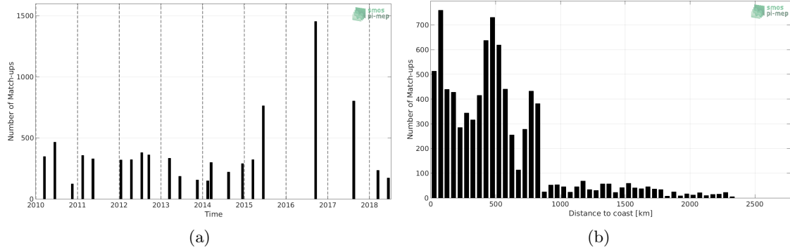
Figure 1: Number of match-ups between TSG-LEGOS-DM and CCI L4 Merged-OI v1.8 - 7-day running (ESA) SSS as a function of time (a) and as function of the distance to coast (b) over the Roaring Forties and Furious Fifties Pi-MEP region and for the full satellite product period.
