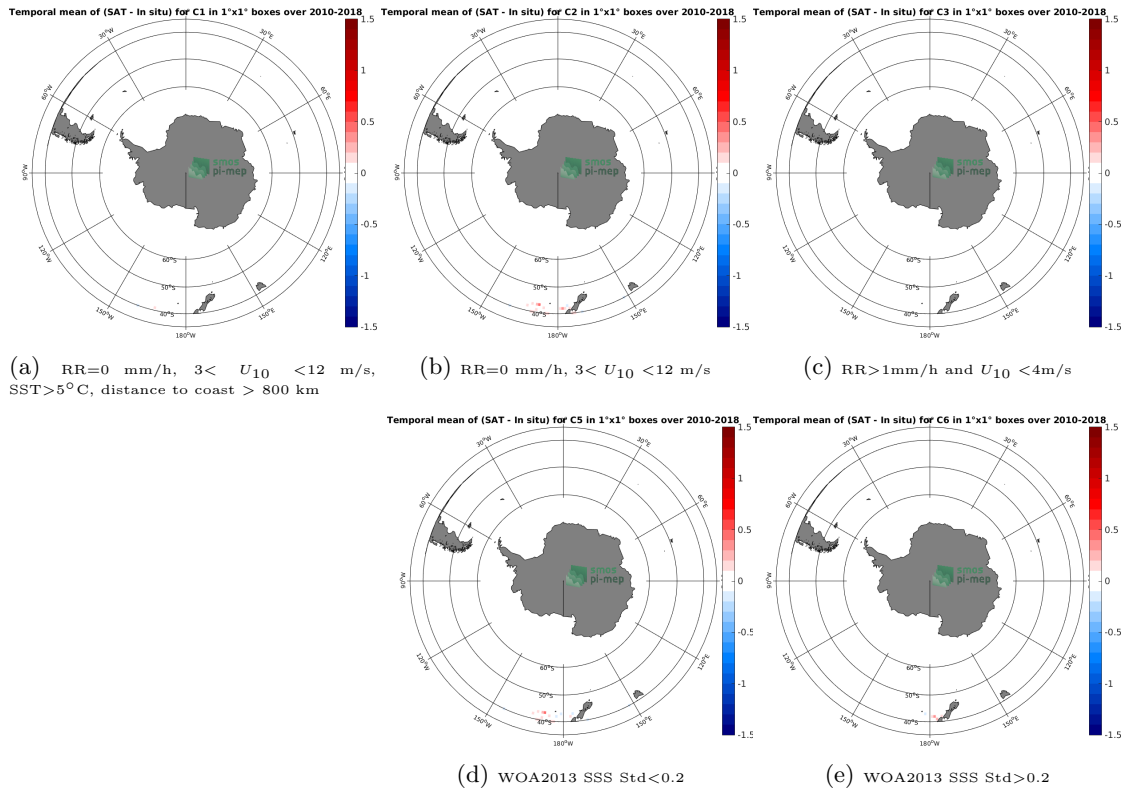
Figure 12: Temporal mean gridded over spatial boxes of size 1^{\circ}\times 1^{\circ} of \Delta\text{SSS} (CCI L4 Merged-OI v1.8 - 7-day running (ESA) - TSG-LEGOS-DM) for 5 different subdatasets corresponding to:RR=0 mm/h, 3 < U_{10} < 12 m/s, SST >5^{\circ}\text{C} , distance to coast > 800 km (a), RR=0 mm/h, 3 < U_{10} < 12 m/s (b), RR >1 mm/h and U_{10} < 4 m/s (c), WOA2013 SSS Std <0.2 (d), WOA2013 SSS Std >0.2 (e).
