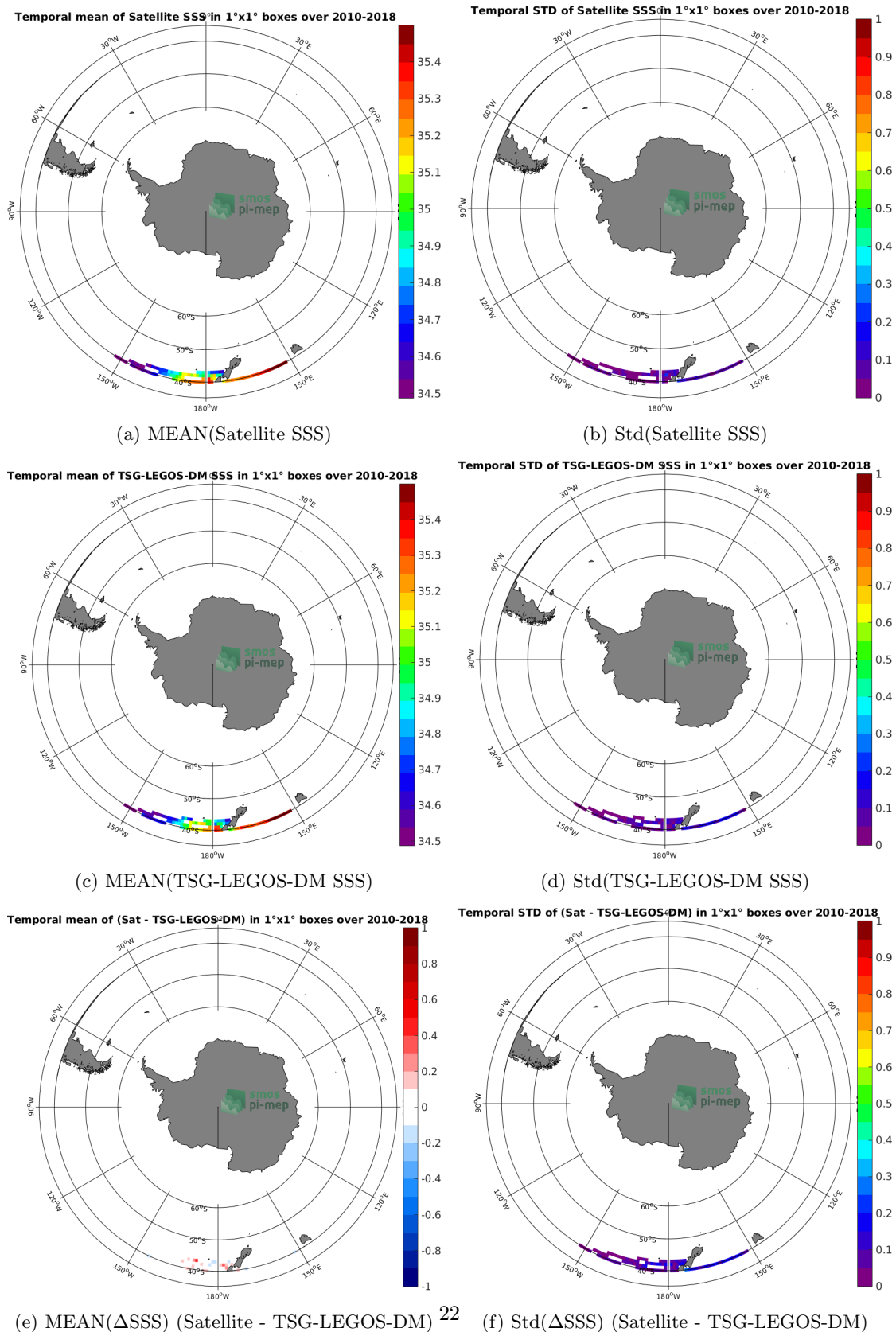
Figure 6: Temporal mean (left) and Std (right) of SSS from CCI L4 Merged-OI v1.8 - 7-day running (ESA) (top), TSG-LEGOS-DM (middle), and of \Delta SSS (Satellite - TSG-LEGOS-DM). Only match-up pairs are used to generate these maps.
