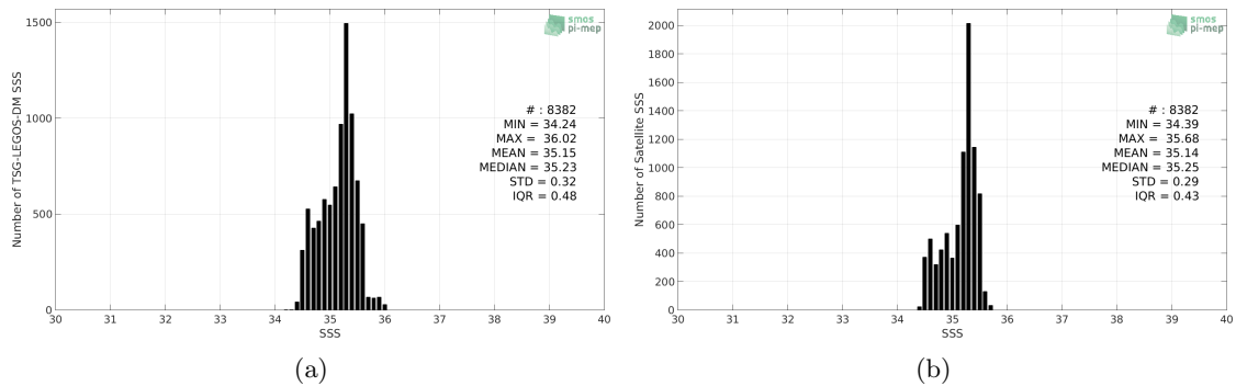
Figure 2: Histograms of SSS from TSG-LEGOS-DM (a) and CCI L4 Merged-OI v1.8 - 7-day running (ESA) (b) considering all match-up pairs per bins of 0.1 over the Roaring Forties and Furious Fifties Pi-MEP region and for the full satellite product period.
