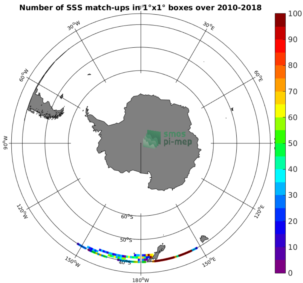
Figure 4: Number of SSS match-ups between TSG-LEGOS-DM SSS and the CCI L4 Merged-OI v1.8 - 7-day running (ESA) SSS product for the Roaring Forties and Furious Fifties Pi-MEP region over 1^\circ \times 1^\circ boxes and for the full satellite product period.
