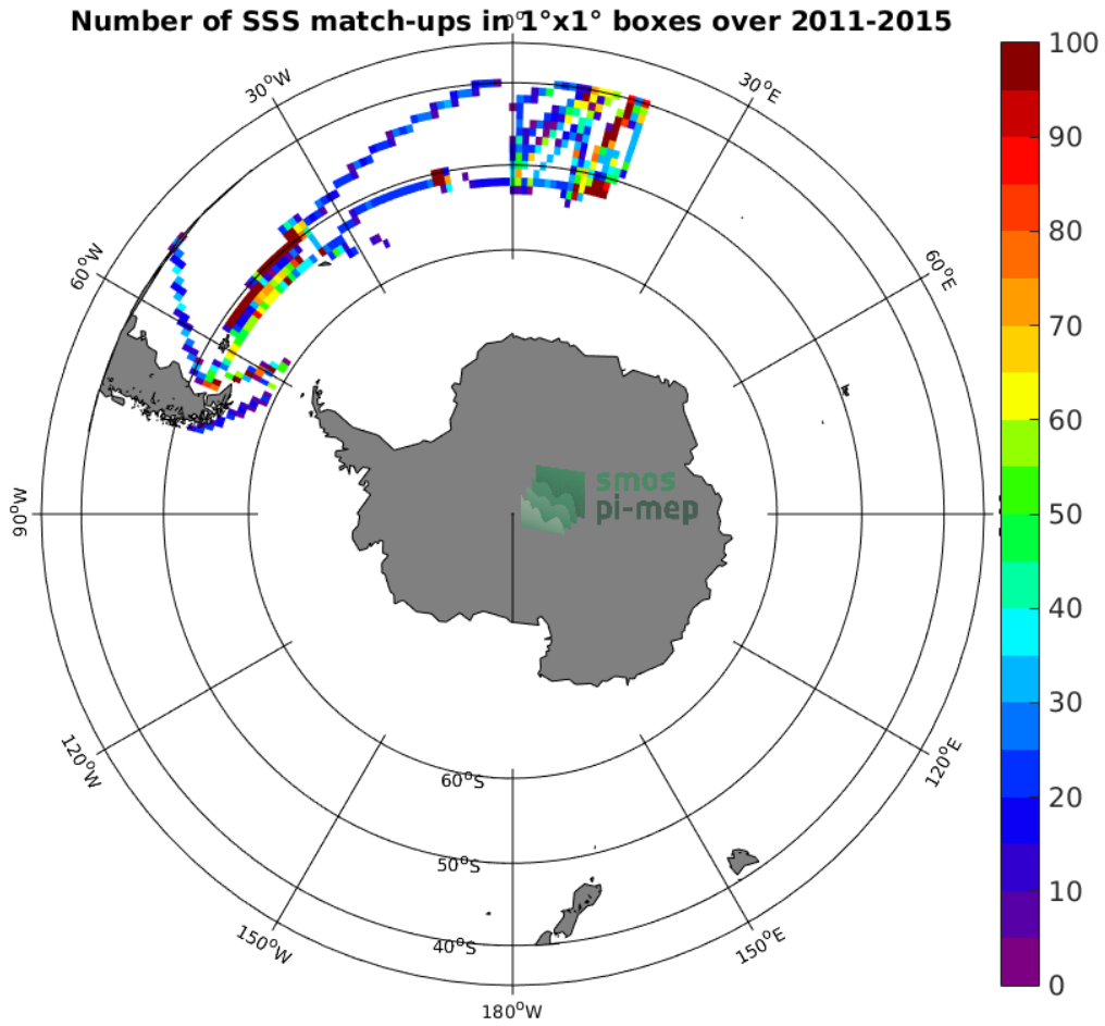
Figure 4: Number of SSS match-ups between TSG-POLARSTERN SSS and the Aquarius-L4-IPRC-V5-WEEKLY SSS product for the Roaring Forties and Furious Fifties Pi-MEP region over 1°x1° boxes and for the full satellite product period.
