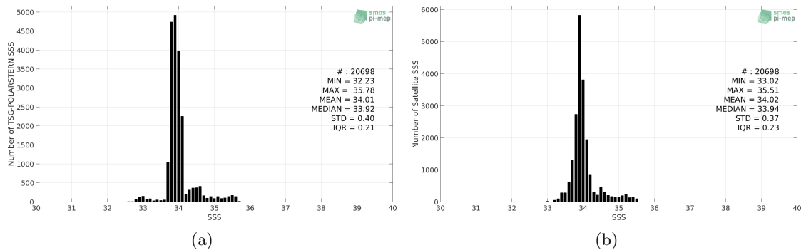
Figure 2: Histograms of SSS from TSG-POLARSTERN (a) and Aquarius-L4-IPRC-V5-WEEKLY (b) considering all match-up pairs per bins of 0.1 over the Roaring Forties and Furious Fifties Pi-MEP region and for the full satellite product period.
