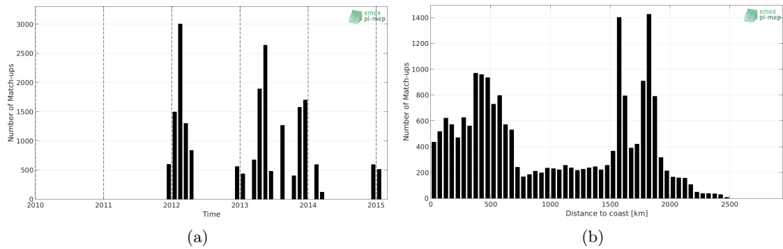
Figure 1: Number of match-ups between TSG-POLARSTERN and Aquarius-L4-IPRC-V5-WEEKLY SSS as a function of time (a) and as function of the distance to coast (b) over the Roaring Forties and Furious Fifties Pi-MEP region and for the full satellite product period.
