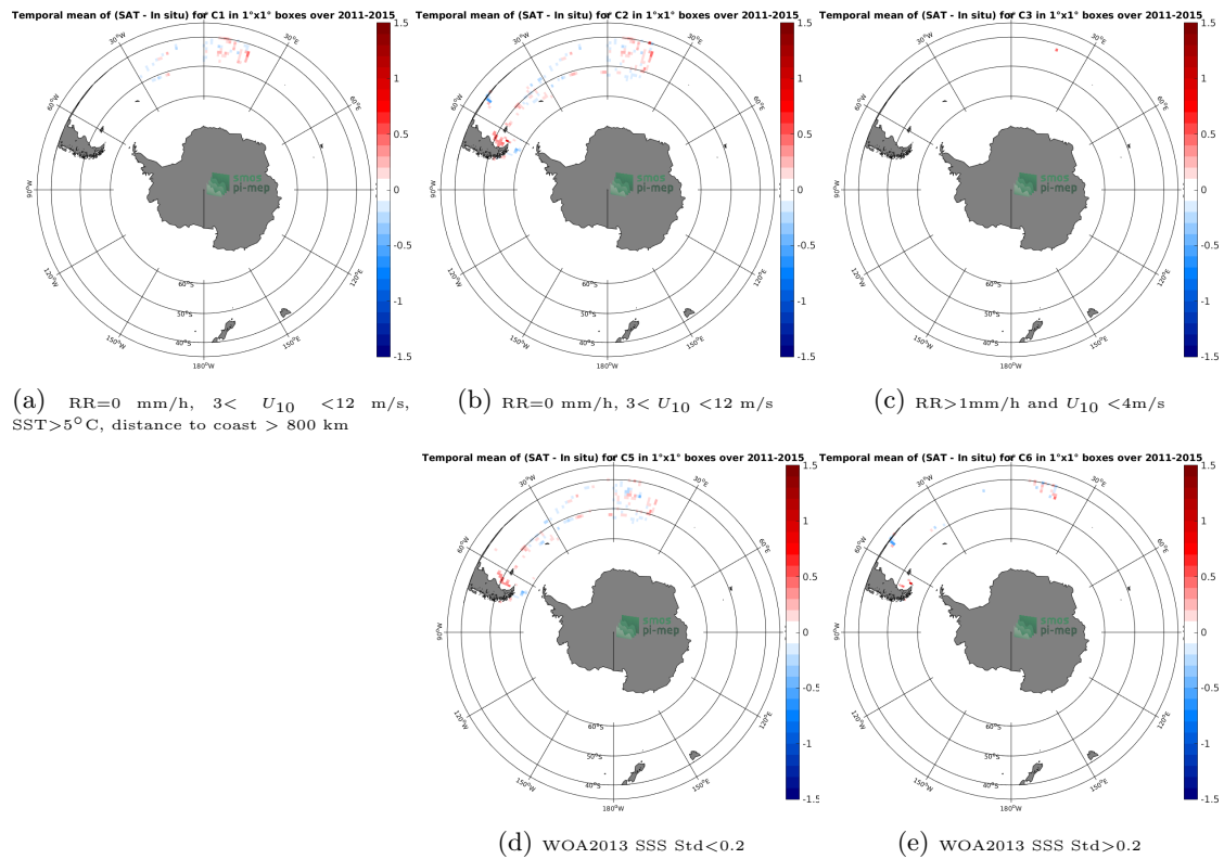
Figure 12: Temporal mean gridded over spatial boxes of size 1^{\circ}\times 1^{\circ} of \Delta\text{SSS} (Aquarius-L4-IPRC-V5-WEEKLY - TSG-POLARSTERN) for 5 different subdatasets corresponding to:RR=0 mm/h, 3 < U_{10} < 12 m/s, SST >5^{\circ}\text{C} , distance to coast > 800 km (a), RR=0 mm/h, 3 < U_{10} < 12 m/s (b), RR >1 mm/h and U_{10} < 4 m/s (c), WOA2013 SSS Std <0.2 (d), WOA2013 SSS Std >0.2 (e).
