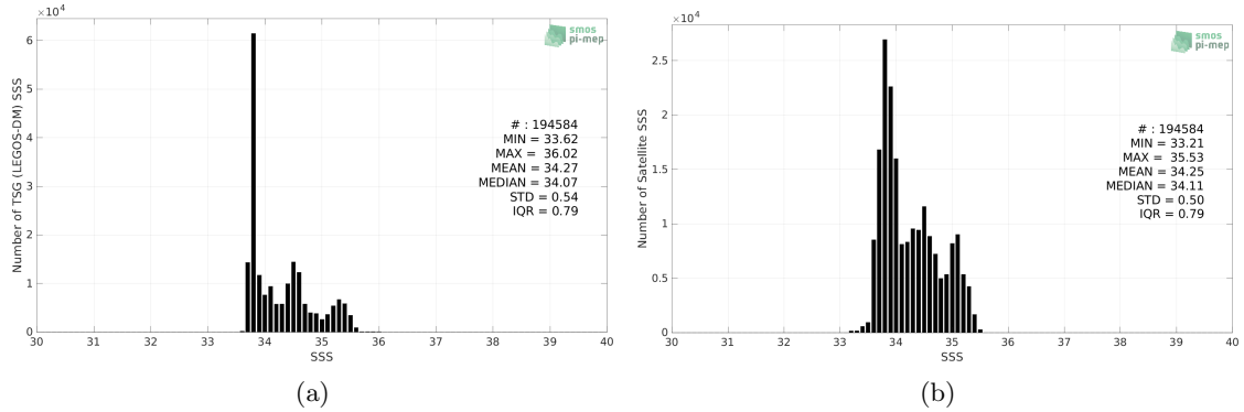
Figure 2: Histograms of SSS from TSG (LEGOS-DM) (a) and Aquarius SSS L4 OI v5 - Weekly (IPRC) (b) considering all match-up pairs per bins of 0.1 over the Roaring Forties and Furious Fifties Pi-MEP region and for the full satellite product period.
