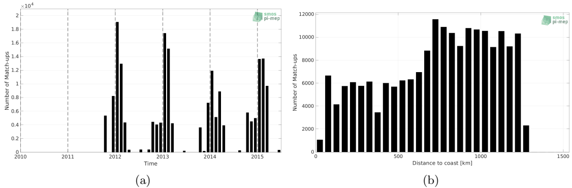
Figure 1: Number of match-ups between TSG (LEGOS-DM) and Aquarius SSS L4 OI v5 - Weekly (IPRC) SSS as a function of time (a) and as function of the distance to coast (b) over the Roaring Forties and Furious Fifties Pi-MEP region and for the full satellite product period.
