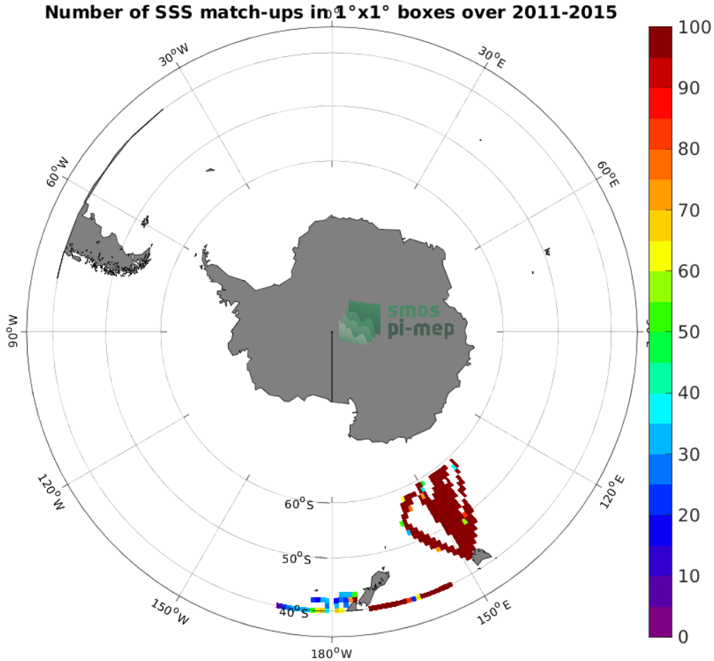
Figure 4: Number of SSS match-ups between TSG (LEGOS-DM) SSS and the Aquarius SSS L4 OI v5 - Weekly (IPRC) SSS product for the Roaring Forties and Furious Fifties Pi-MEP region over 1^\circ \times 1^\circ boxes and for the full satellite product period.
