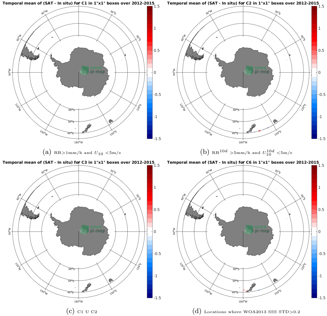
Figure 12: Temporal mean gridded over spatial boxes of size 1^\circ \times 1^\circ of \Delta SSS (Aquarius-L4-IPRC-V5-WEEKLY - TSG-LEGOS-DM) for 4 different subdatasets corresponding to:RR >1 mm/h and U_{10} < 5 m/s (a), RR 10d > 5 mm/h and U_{10}^{10d} < 5 m/s (b), C1 U C2 (c),Locations where WOA2013 SSS STD > 0.2 (d).
