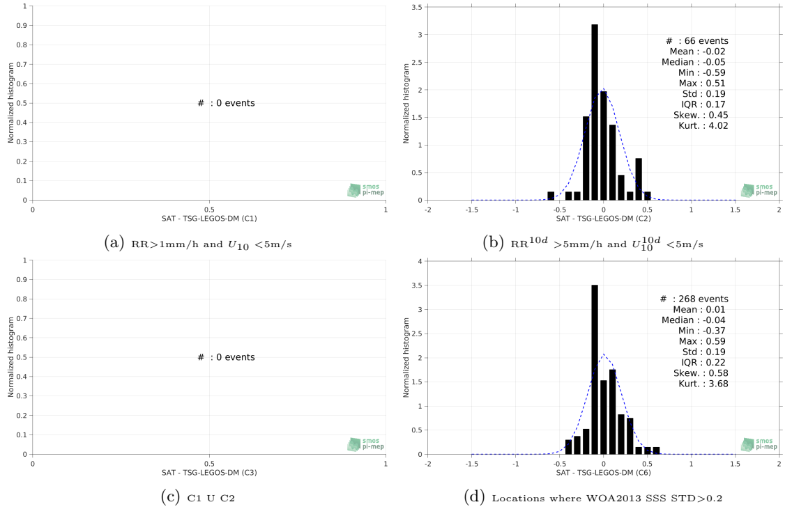
Figure 13: Normalized histogram of \Delta\text{SSS} (Aquarius-L4-IPRC-V5-WEEKLY - TSG-LEGOS-DM) for 6 different subdatasets corresponding to: RR > 1\text{mm/h} and U_{10} < 5\text{m/s} (a), RR^{10d} > 5\text{mm/h} and U_{10}^{10d} < 5\text{m/s} (b), C1 \cup C2 (c), Locations where WOA2013 SSS STD > 0.2 (d).
