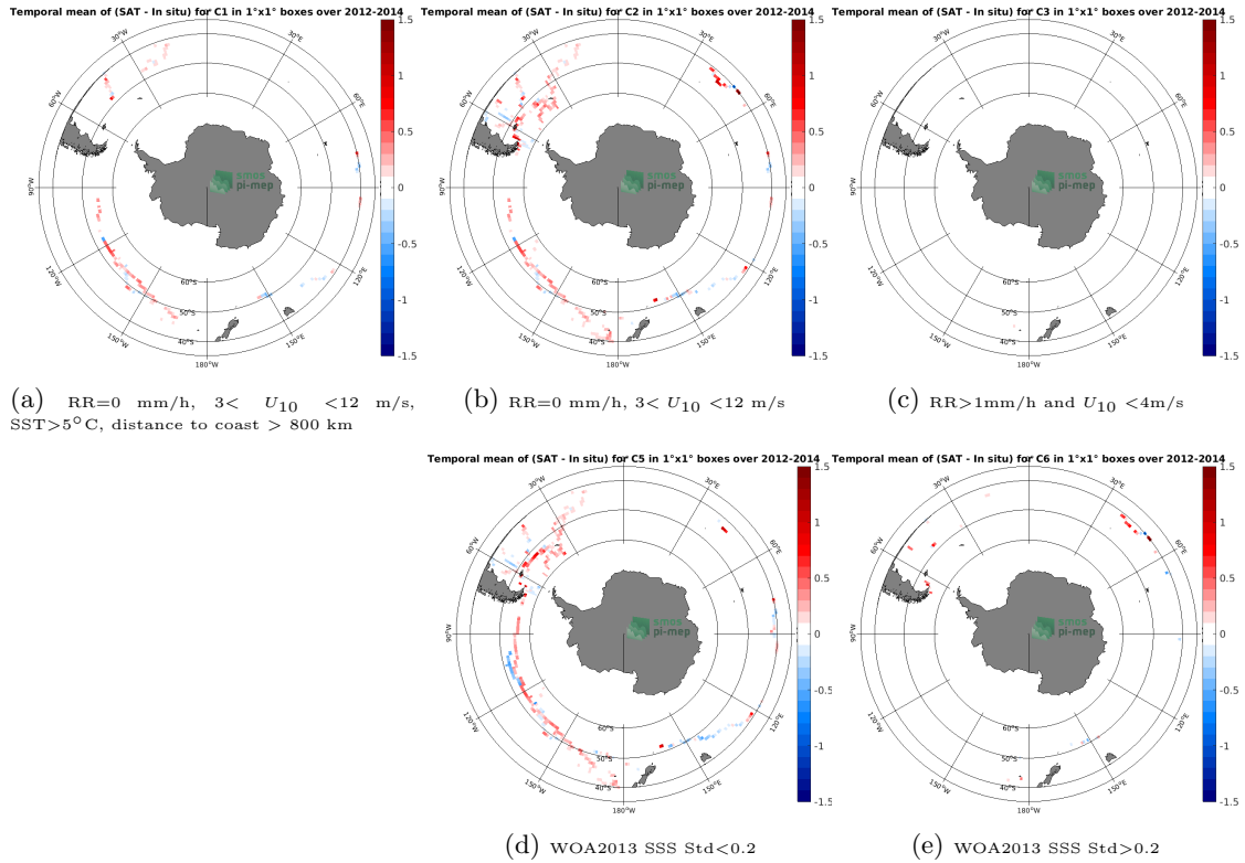
Figure 12: Temporal mean gridded over spatial boxes of size 1°x1° of \Delta SSS (Aquarius SSS L4 OI v5 - Weekly (IPRC) - TSG (GOSUD-Sailing-ship)) for 5 different subdatasets corresponding to:RR=0 mm/h, 3 < U_{10} < 12 m/s, SST>5°C, distance to coast > 800 km (a), RR=0 mm/h, 3 < U_{10} < 12 m/s (b), RR>1mm/h and U_{10} < 4 m/s (c), WOA2013 SSS Std<0.2 (d), WOA2013 SSS Std>0.2 (e).
